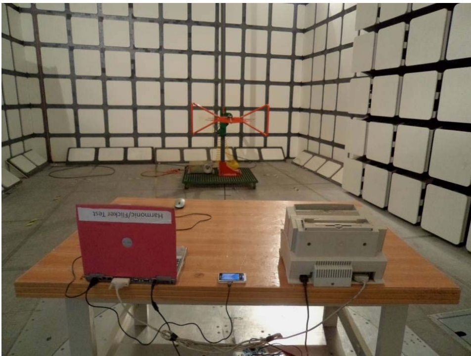
Radiated Spurious Emissions - Rear View
