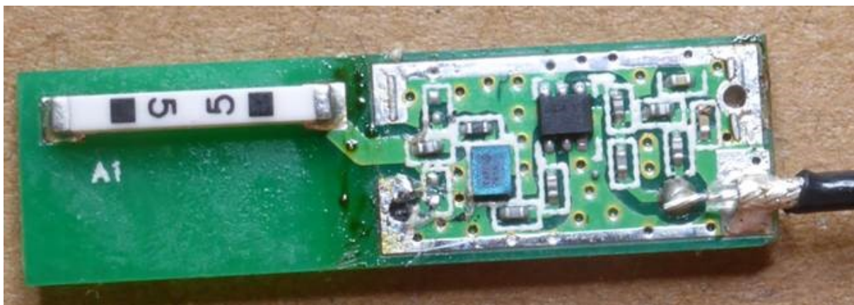
PCB Top (shielding removed)
