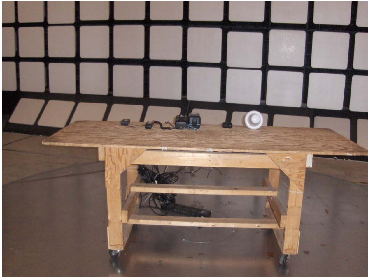
Photo #2(b): IsatDOCK MARINE, Model ISD-Marine + AT1595-82 (from 30 MHz – 1 GHz)
