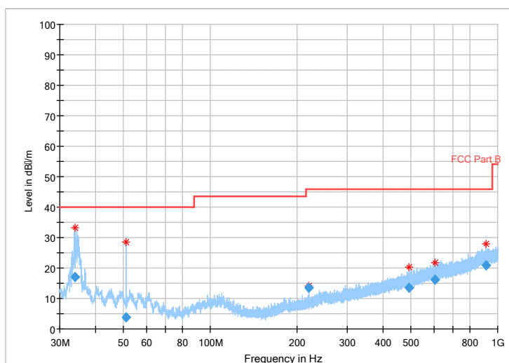
Fig.43 Radiated emission: \pi/4 DQPSK, Ch78, 30MHz~1GHz
