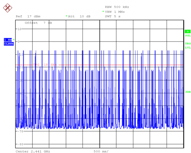
Fig.64 Time of occupancy (Dwell Time): Ch39,Packet 3-DH1
