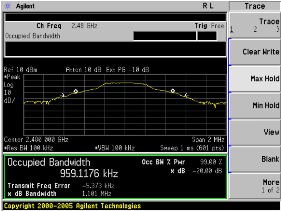
TEST PLOT OF BANDWIDTH FOR TOP CHANNEL
