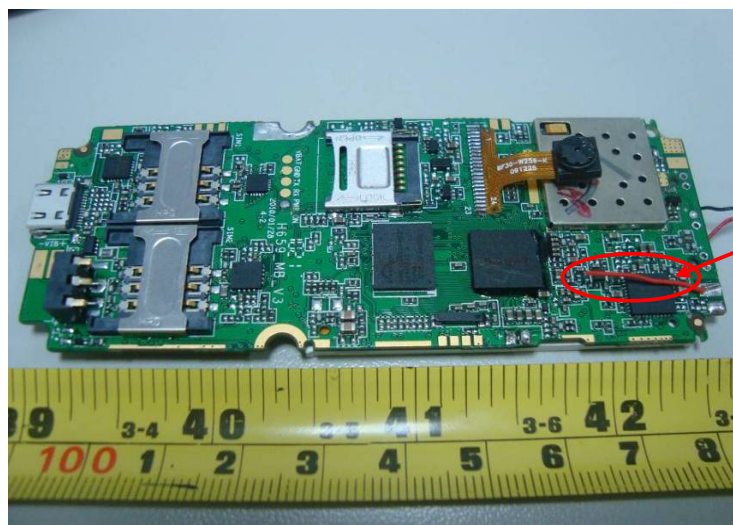
Bluetooth antenna
