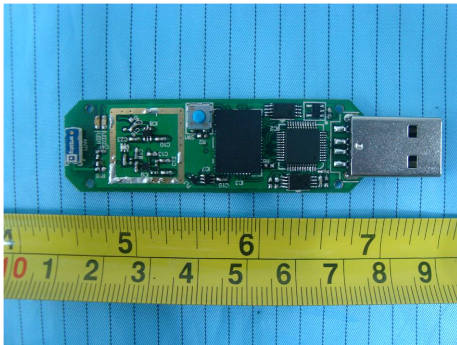
EUT – Main Board RF Cover off Top View
