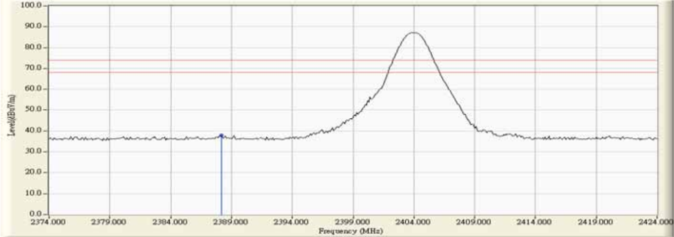
Horizontal (Peak) TX 2404MHz
