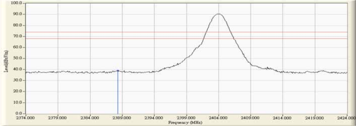
Vertical (Peak) TX 2404MHz
