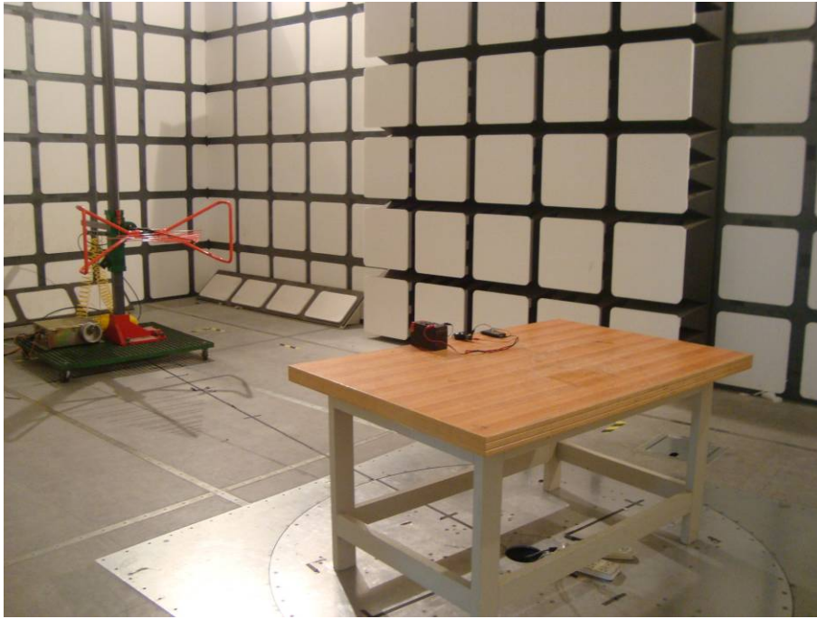
Below 1GHz: Radiated Emissions - Front View for Transmitting
