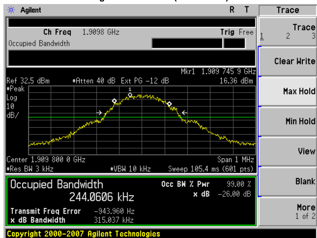
Figure Channel 810 (1909.80MHz)
