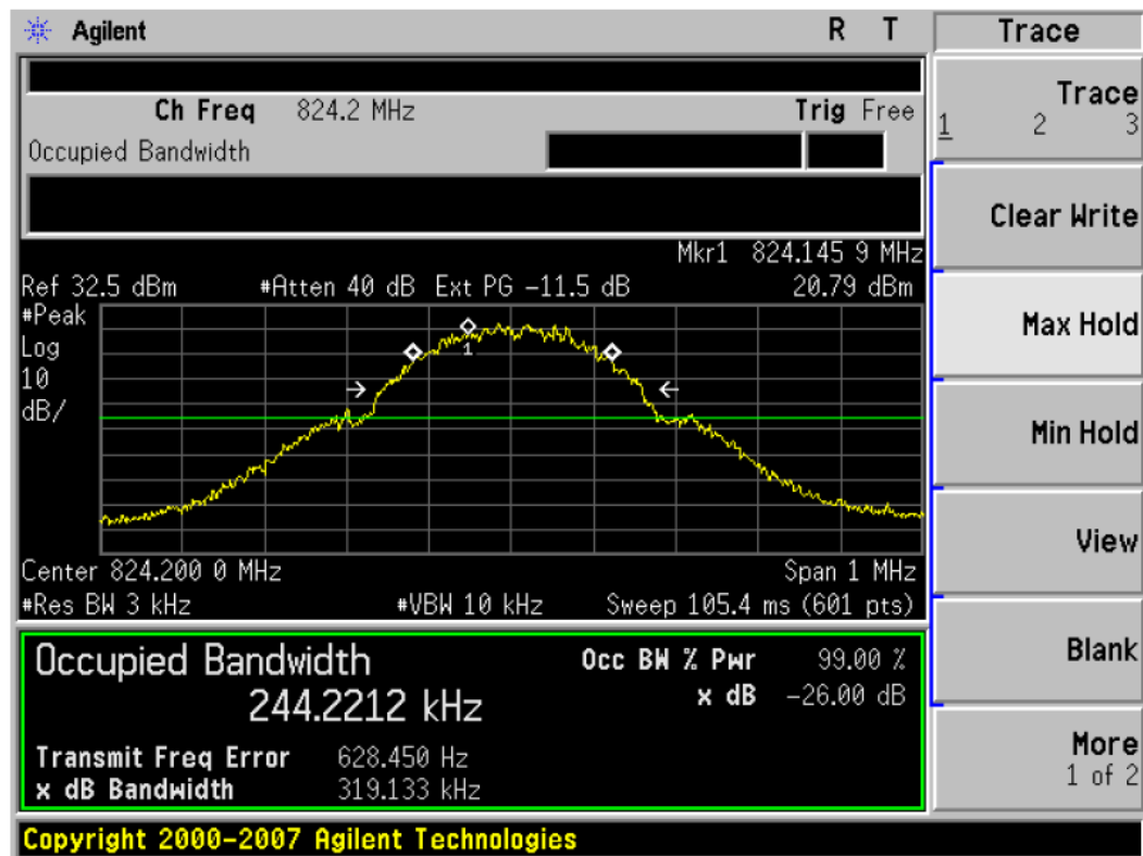
Figure Channel 128 (824.20MHz)
