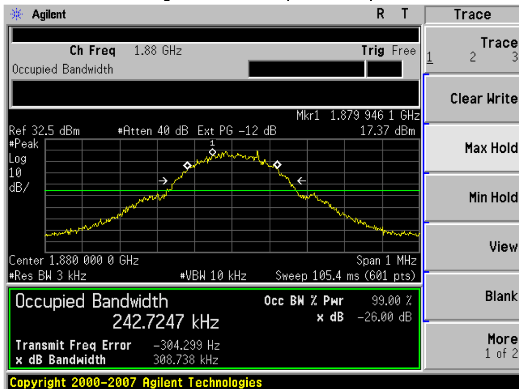
Figure Channel 661 (1880.00MHz)
