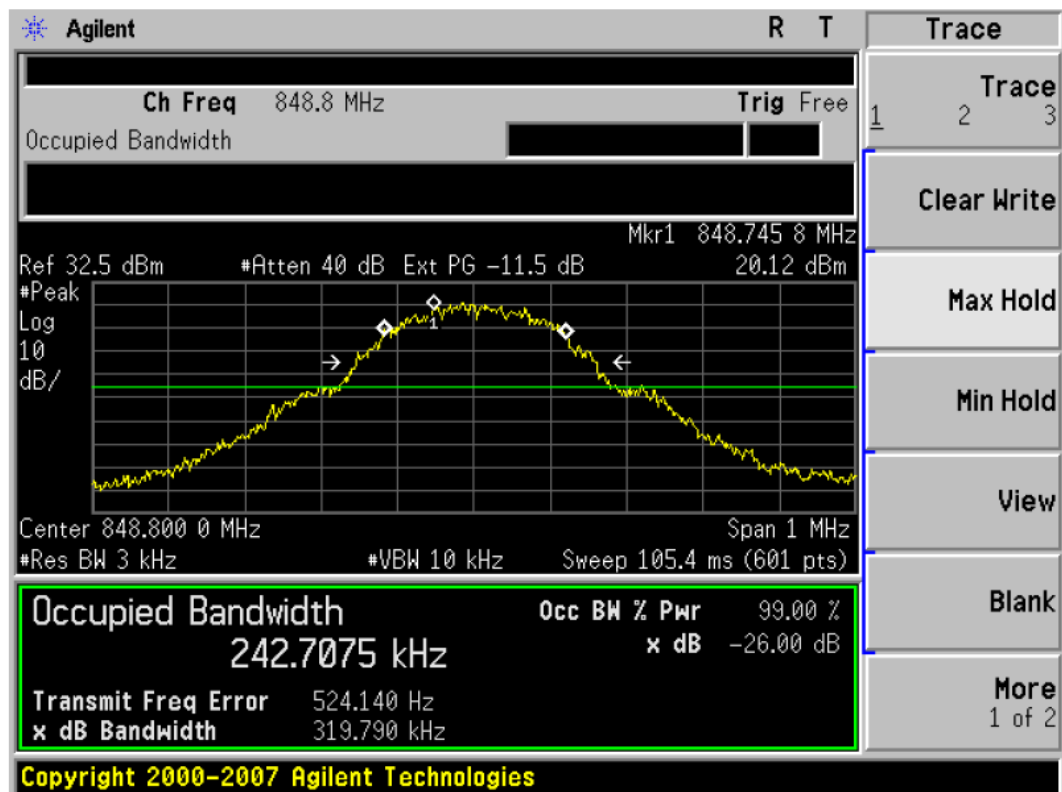
Figure Channel 251 (848.80MHz)
