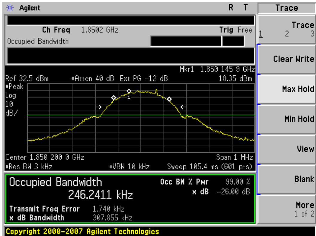
Figure Channel 512 (1850.20MHz)
