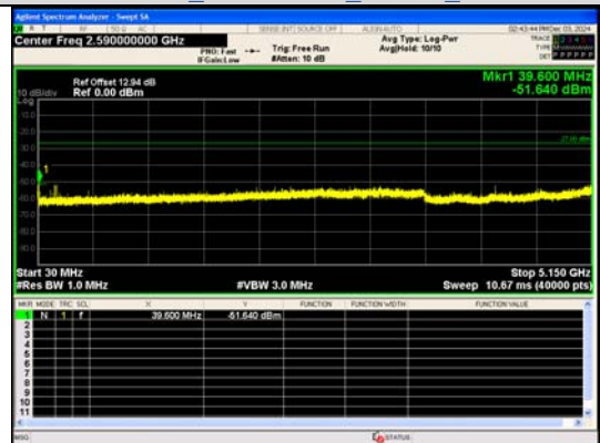
Spurious Emission:30.0~5150 MHz IEEE 802.11n_Channel 64_20MHz_Antenna 0
