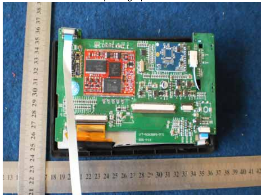
LCD PCB photograph of EUT
