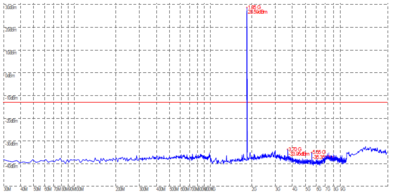
(Plot D: GSM 1900MHz Channel = 512, 30MHz to 20GHz)
