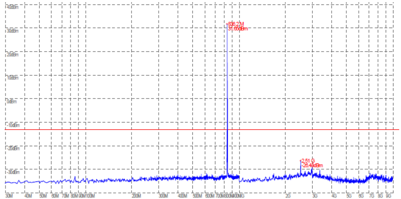
(Plot B: GSM 850MHz Channel = 190, 30MHz to 10GHz)
