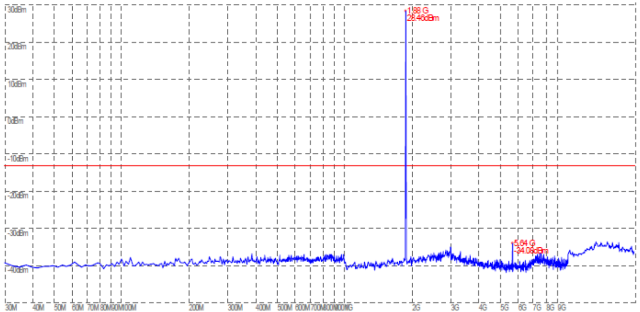
(Plot E: GSM 1900MHz Channel = 661, 30MHz to 20GHz)
