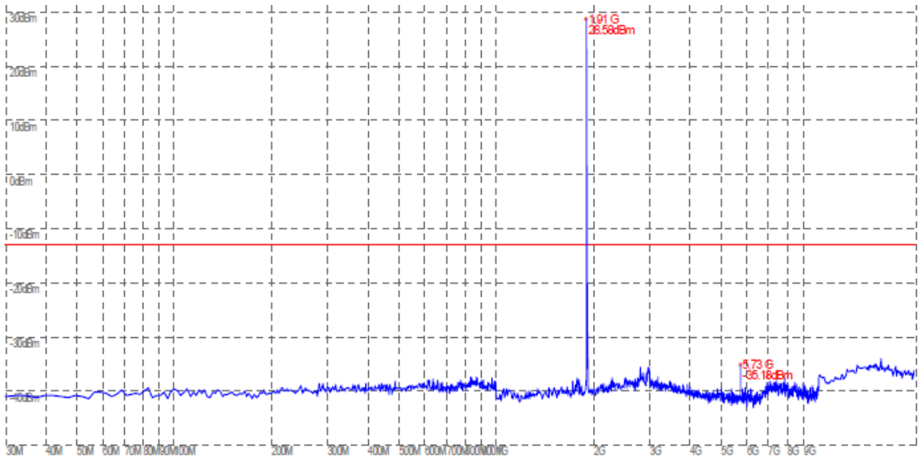
(Plot F: GSM 1900MHz Channel = 810, 30MHz to 20GHz)
