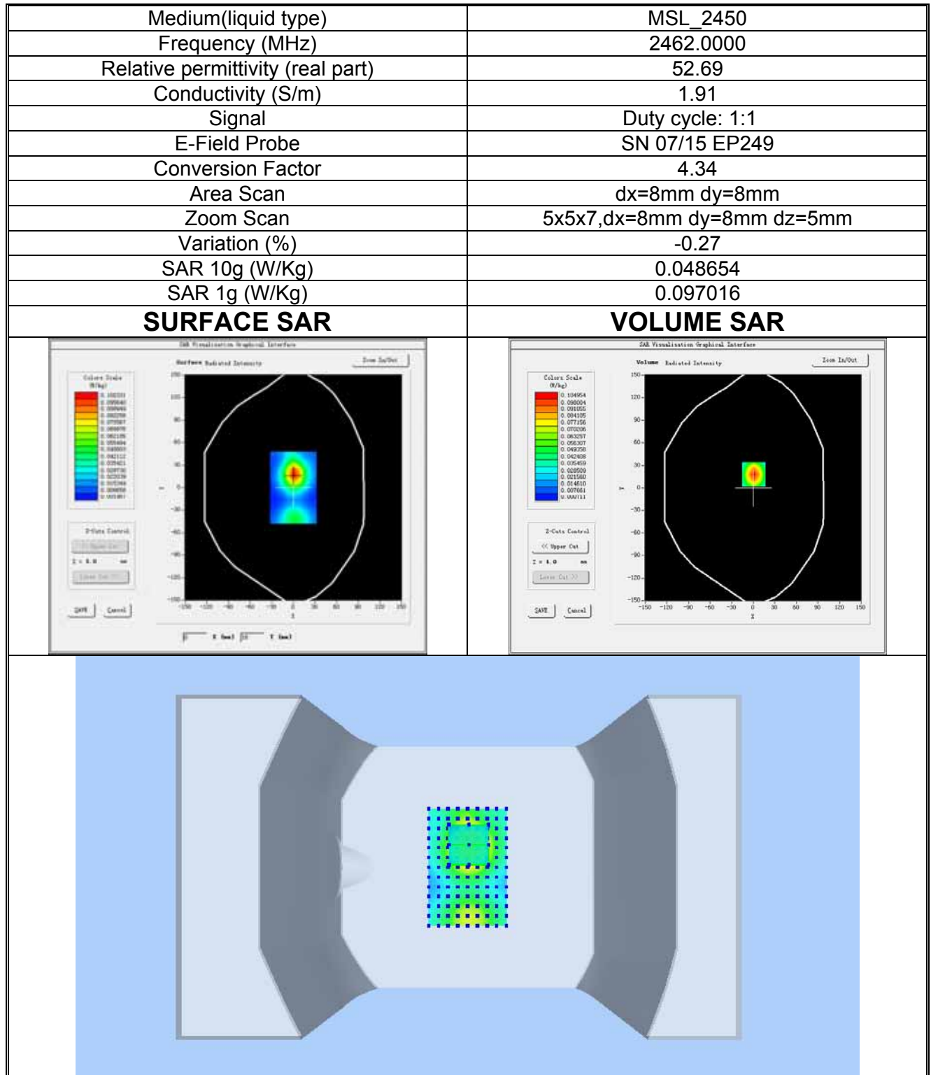
Plot 4:High channel (Body, Left edge) Product Description: Hardware wallet Test Date: 2018-08-21
