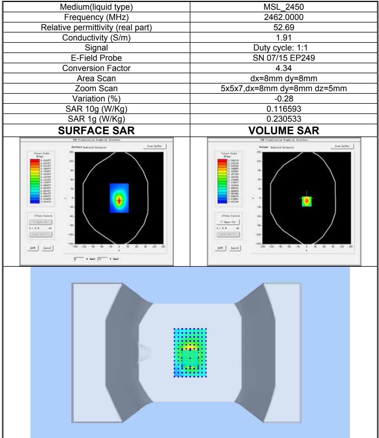
Plot 3:High channel (Body, Top edge) Product Description: Hardware wallet Test Date: 2018-08-21
