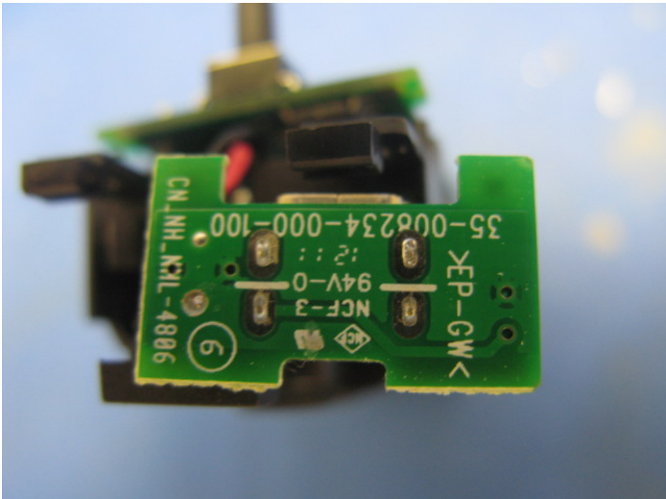
WiFi Camera USB Port rear side
