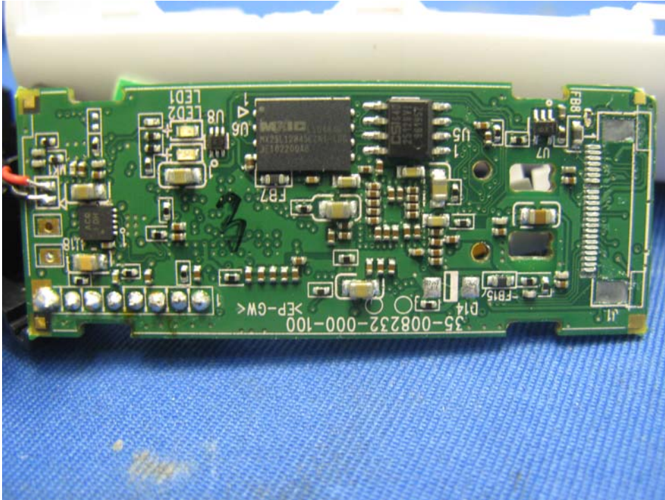
WiFi Camera Main PCB solder side (View 2)
