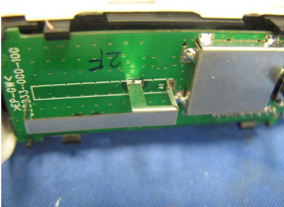
WiFi Camera RF Module PCB solder side
