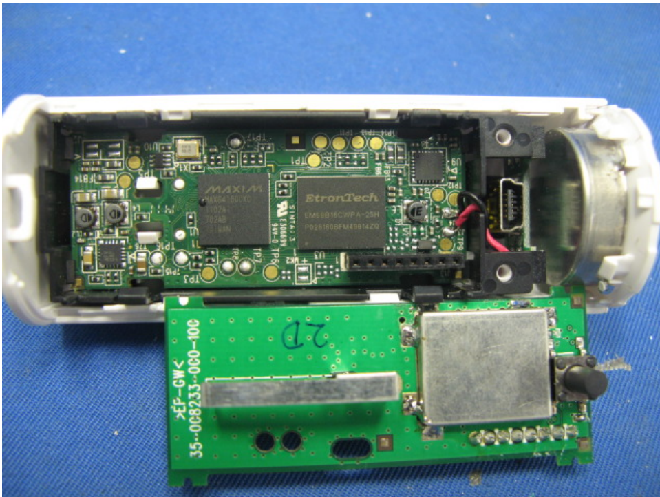
WiFi Camera assembly (View 2)
