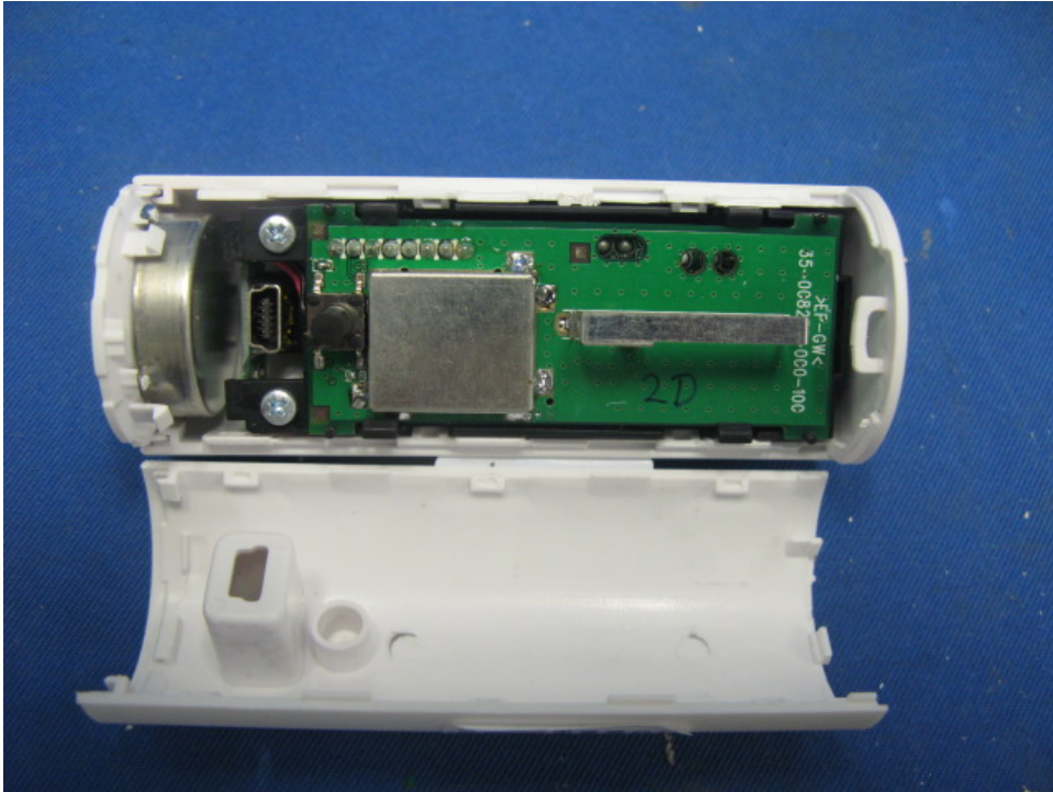
WiFi Camera assembly (View 1)
