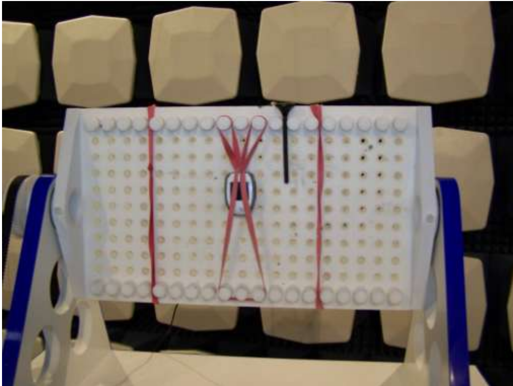
Photo: measurements of radiated field strength, set-up 2
