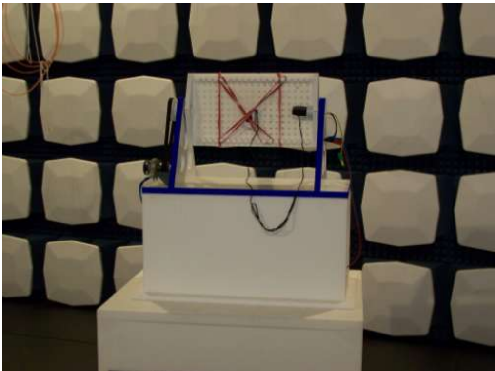
Photo: measurements of radiated field strength, set-up 1
