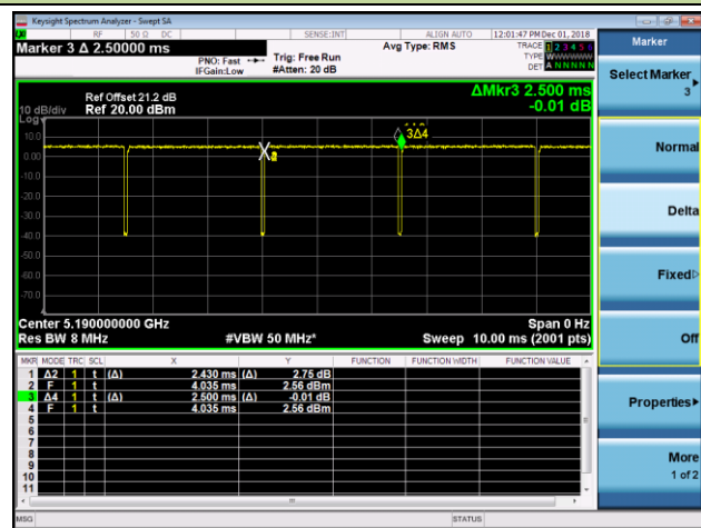
802.11ac-VHT40 (T = 2.430ms)
