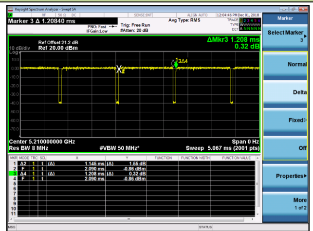
802.11ac-VHT80 (T = 1.145ms)
