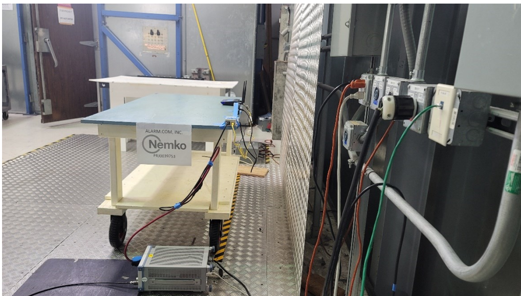
Figure 15 – Test setup, side view.
