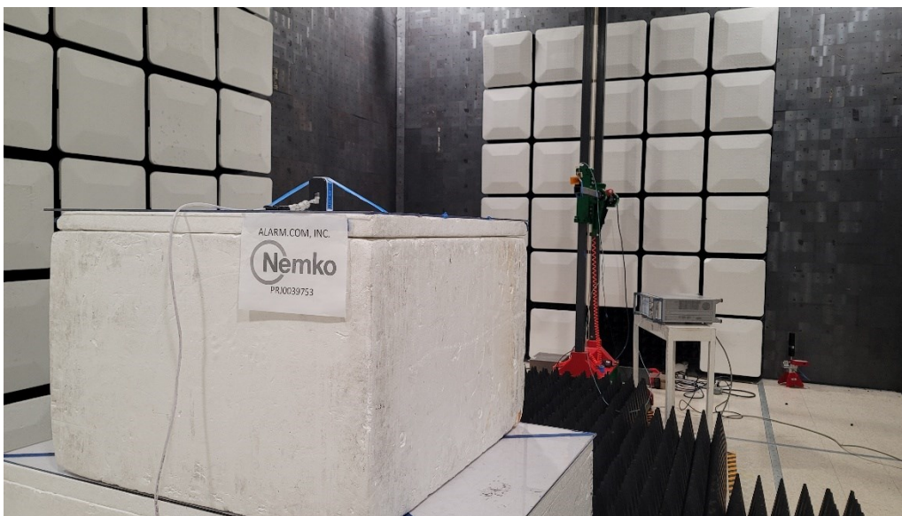
Figure 9- Radiated emissions above 1 GHz (26.5 – 40 GHz), rear view.
