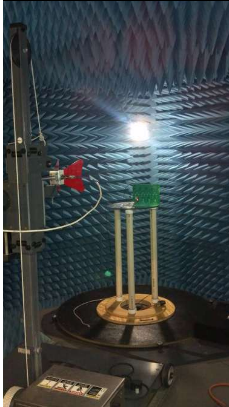
Photograph 5. Radiated Spurious Emissions, Test Setup
