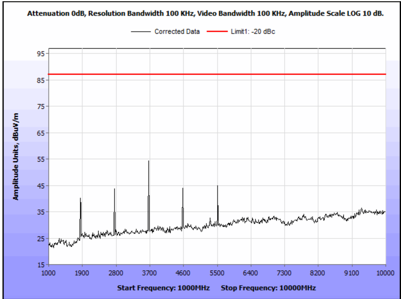
Plot 22. Radiated Spurious Emissions, Mid Channel, 100 kHz, RBW
