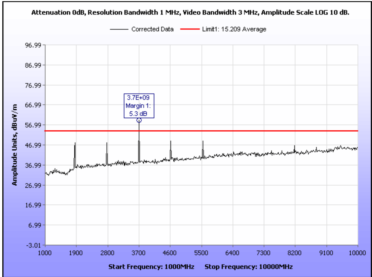
Plot 24. Radiated Spurious Emissions, High Channel, Peak under Average
