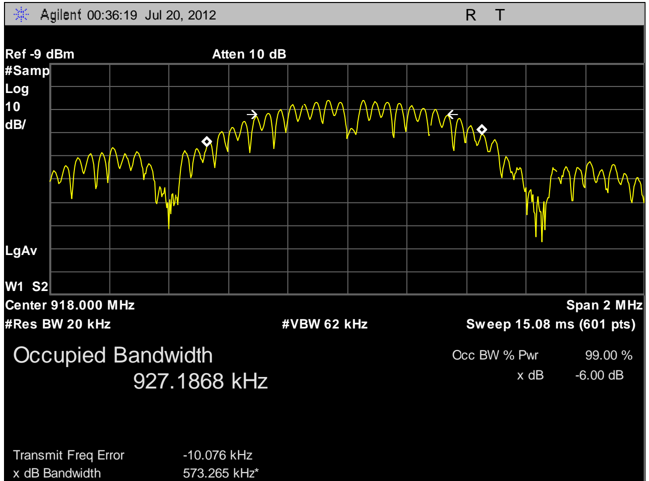
Plot 10. 99% Occupied Bandwidth, Mid Channel
