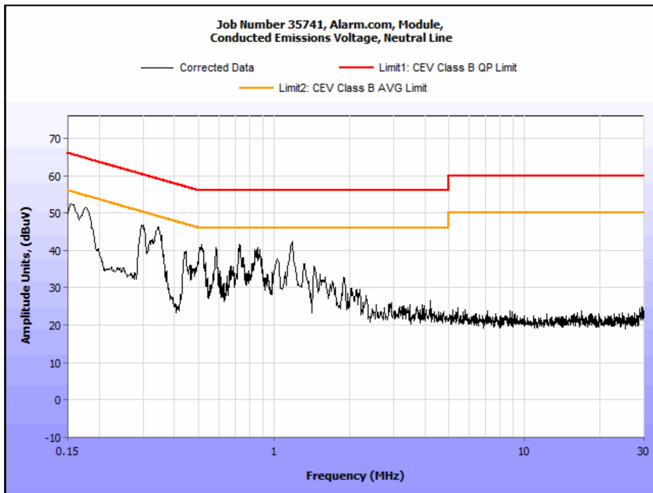
Plot 5. Conducted Emissions, 15.207(a), Neutral Line
