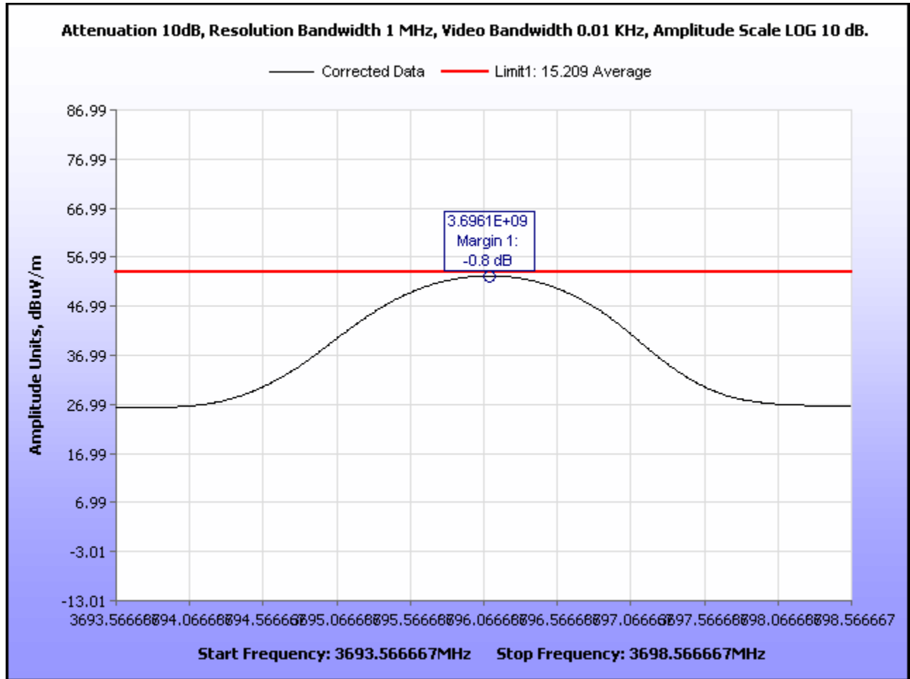
Plot 25. Radiated Spurious Emissions, High Channel, 3700 MHz, Average
