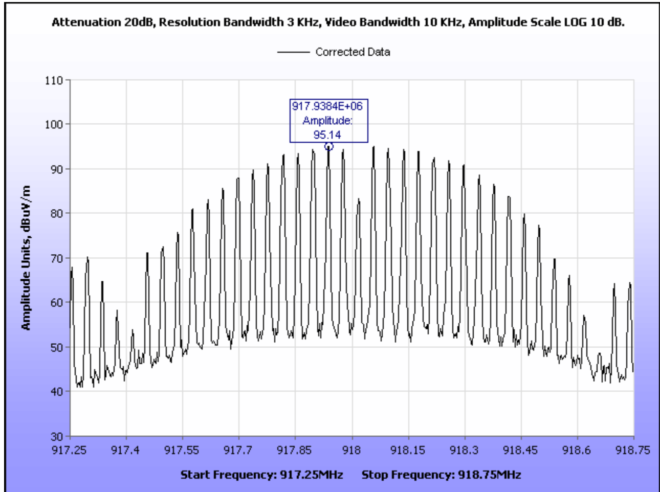
Plot 31. Peak Power Spectral Density, Mid Channel, Peak Determination
