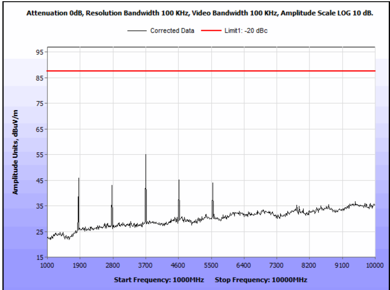
Plot 26. Radiated Spurious Emissions, High Channel, 100 kHz, RBW
