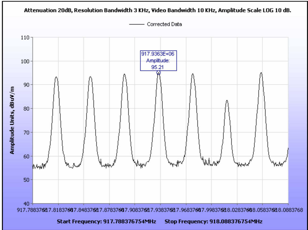
Plot 32. Peak Power Spectral Density, Mid, Channel
