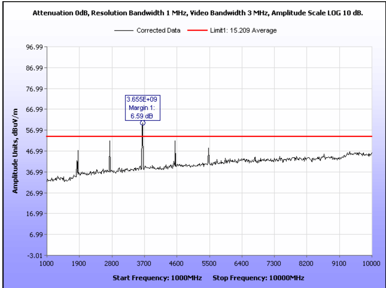
Plot 16. Radiated Spurious Emissions, Low Channel, Peak under Average
