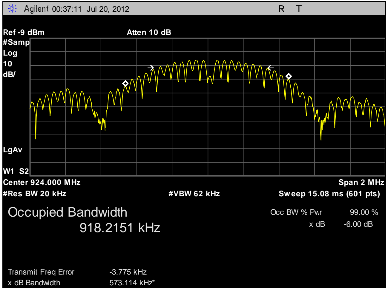
Plot 11. 99% Occupied Bandwidth, High Channel
