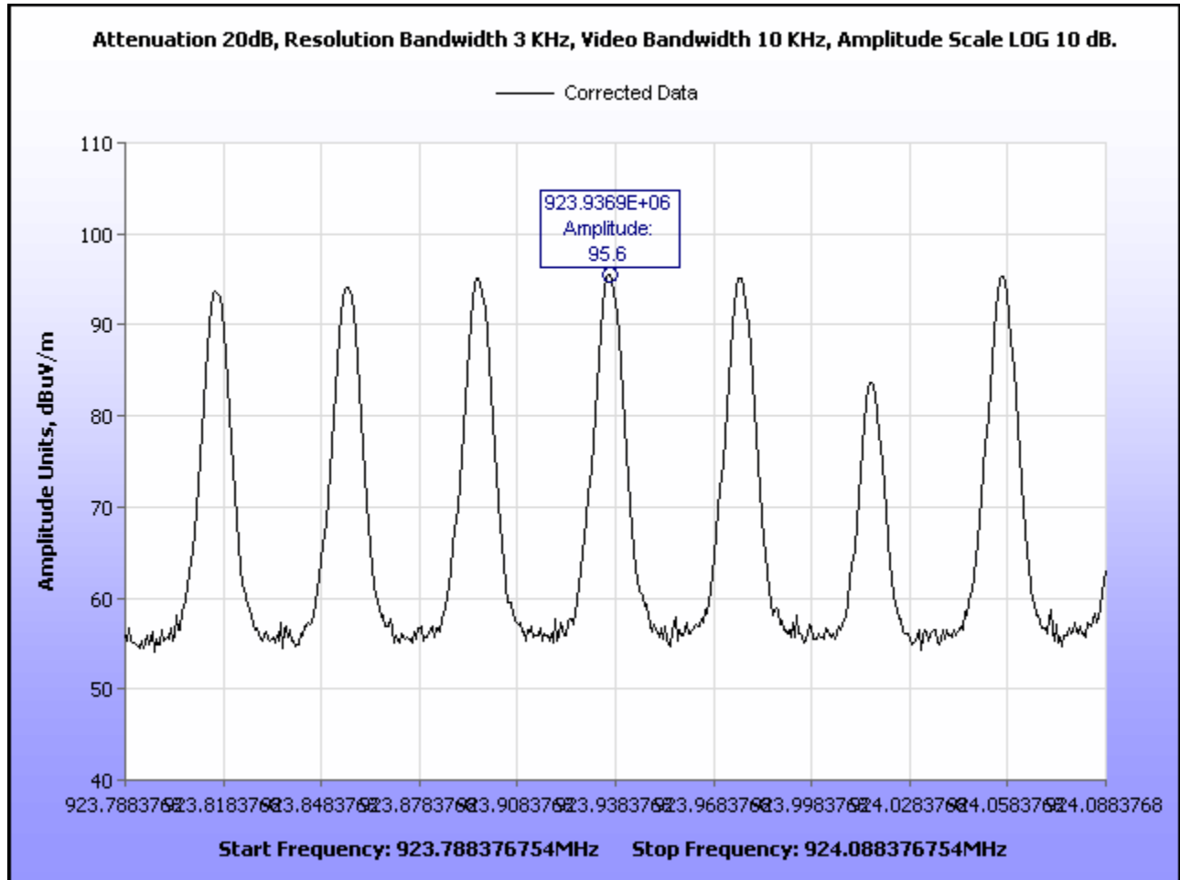
Plot 34. Peak Power Spectral Density, High Channel
