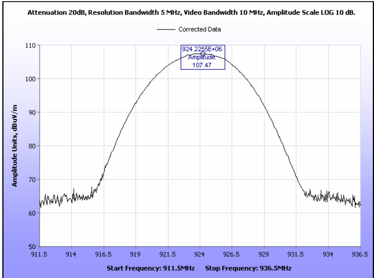
Plot 14. Peak Power Output, High Channel
