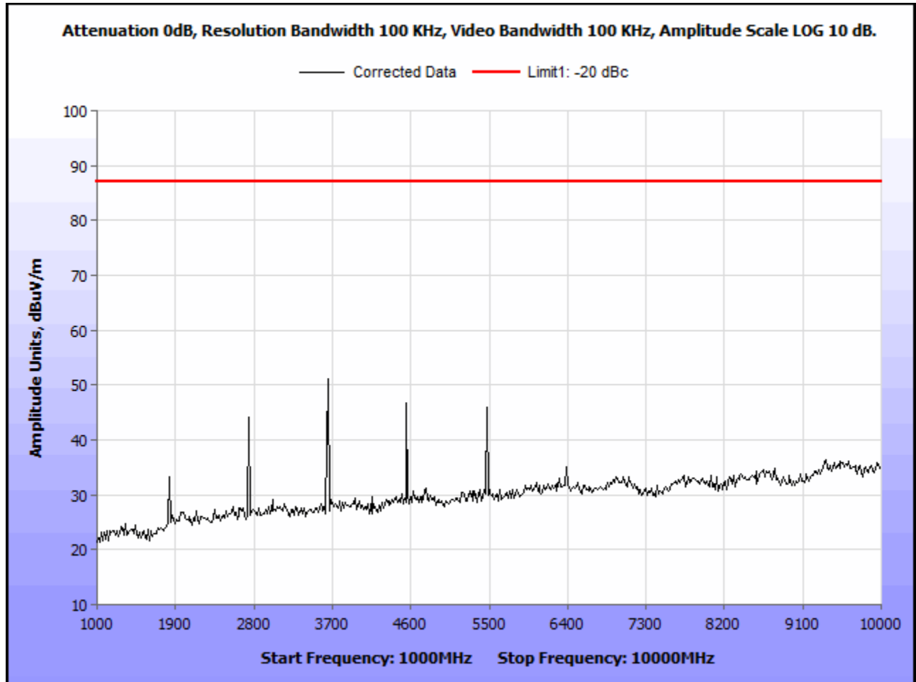
Plot 18. Radiated Spurious Emissions, Low Channel, 100 kHz, RBW
