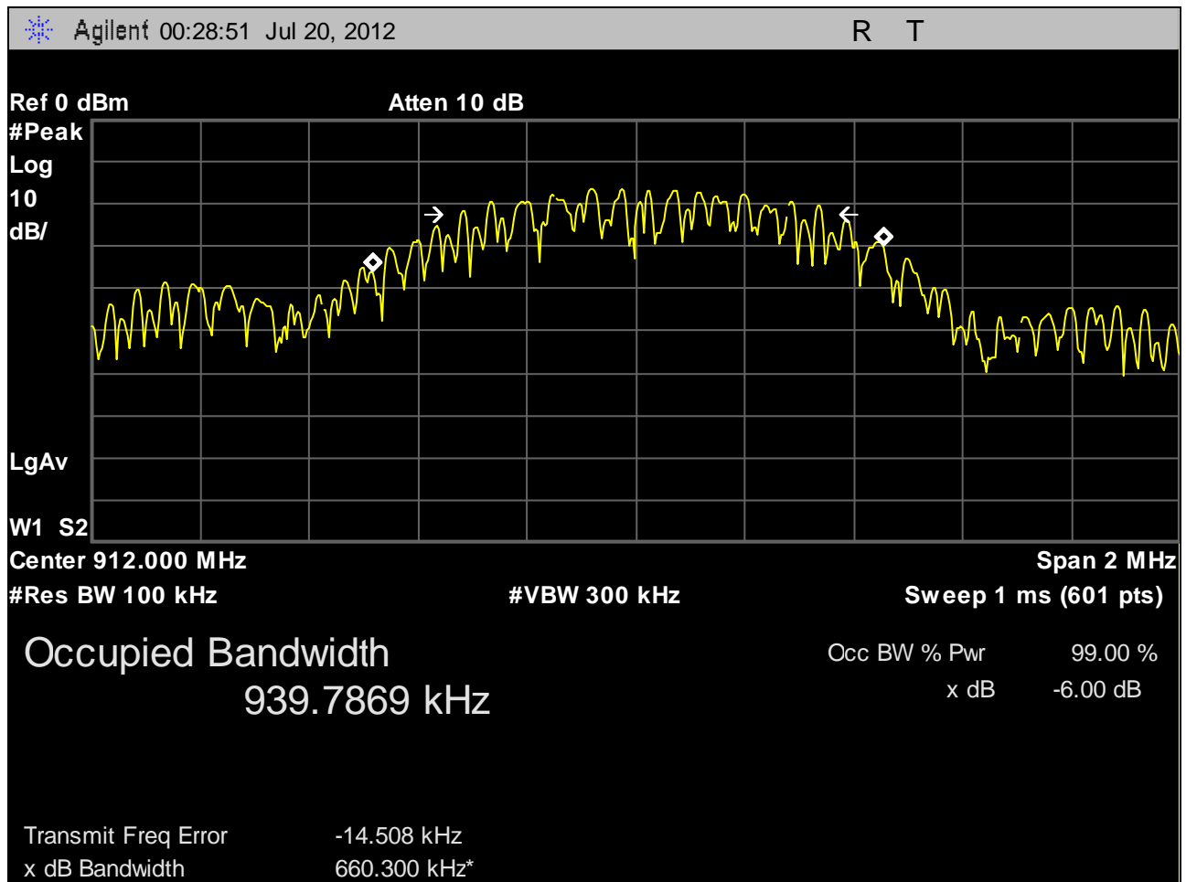
Plot 6. 6 dB Occupied Bandwidth, Low Channel
