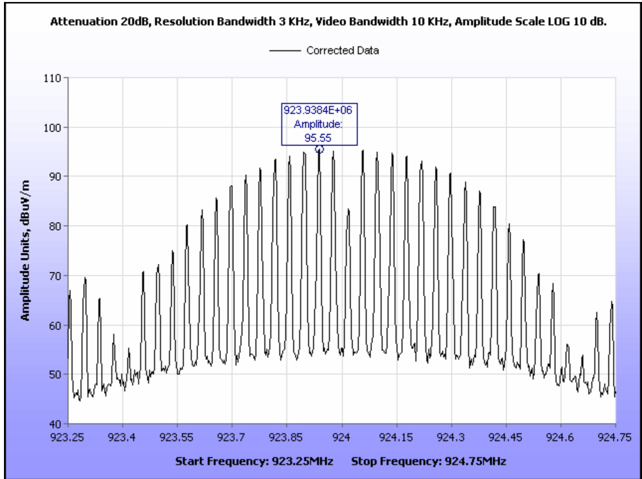
Plot 33. Peak Power Spectral Density, High Channel, Peak Determination
