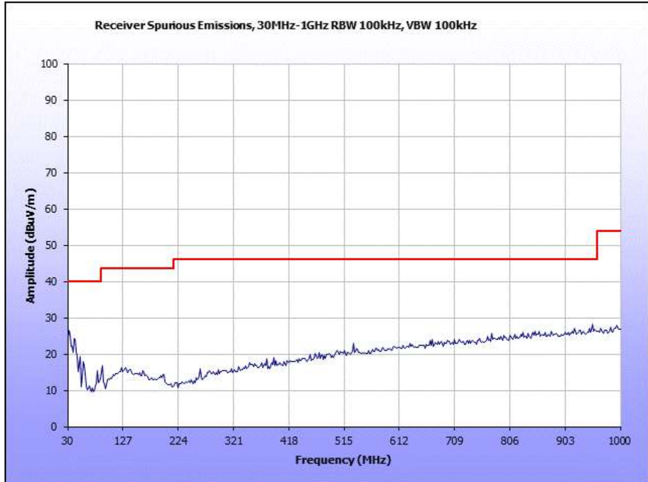
Plot 35. Receiver Spurious Emission, 30 MHz – 1 GHz
