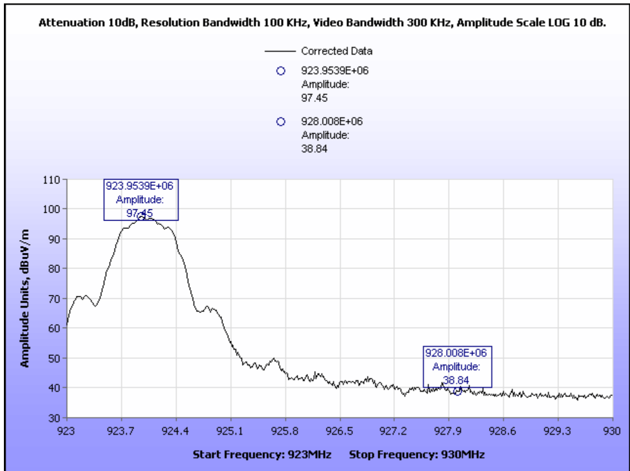
Plot 28. Radiated Band Edge, High Channel
