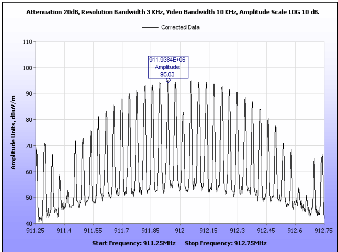
Plot 29. Peak Power Spectral Density, Low Channel, Peak Determination
