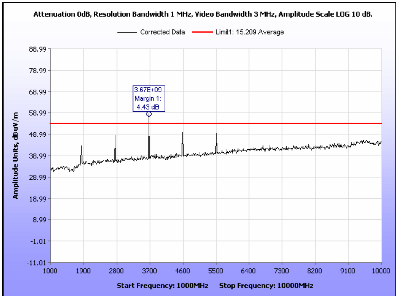
Plot 20. Radiated Spurious Emissions, Mid Channel, Peak under Average
