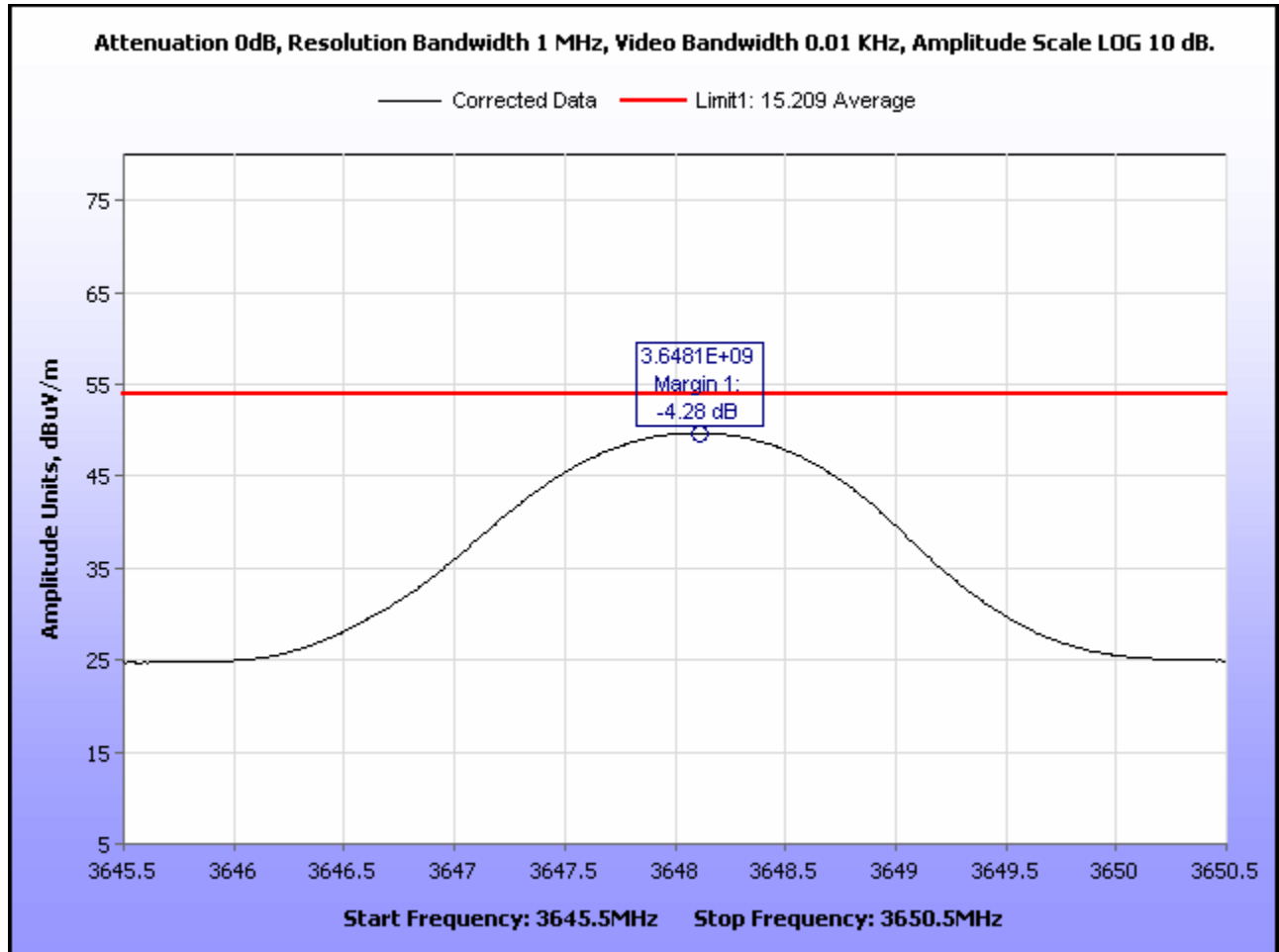
Plot 17. Radiated Spurious Emissions, Low Channel, 3648 MHz, Average
