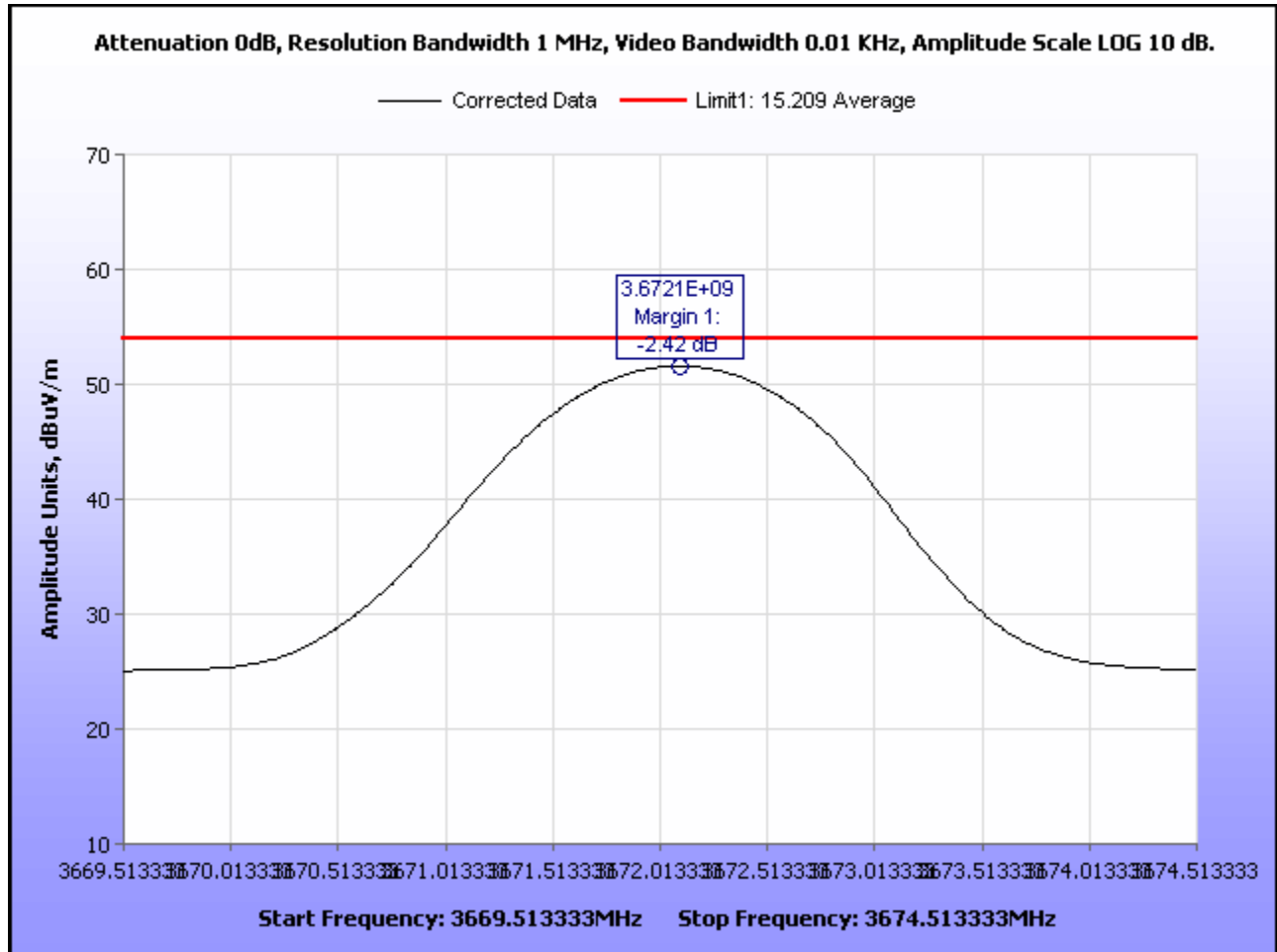
Plot 21. Radiated Spurious Emissions, Mid Channel, 3670 MHz, Average
