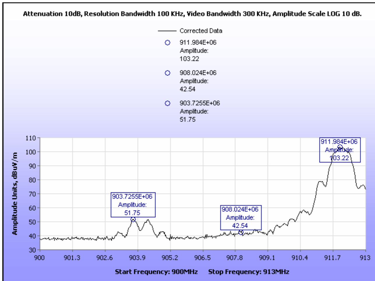
Plot 27. Radiated Band Edge, Low Channel
