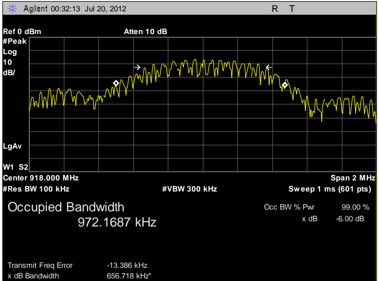
Plot 7. 6 dB Occupied Bandwidth, Mid Channel
