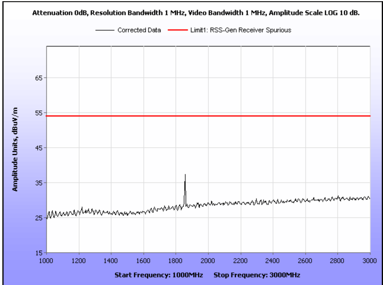
Plot 36. Receiver Spurious Emission, 1 GHz – 3 GHz
