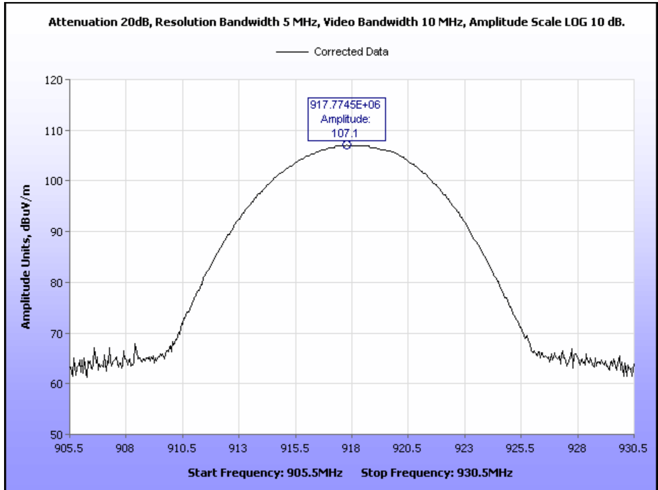
Plot 13. Peak Power Output, Mid Channel
