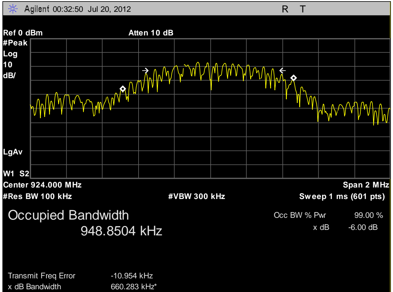
Plot 8. 6 dB Occupied Bandwidth, High Channel
