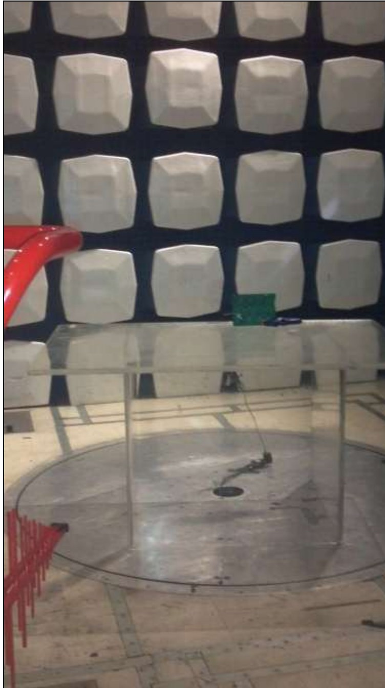
Photograph 3. Radiated Emission, Test Setup
