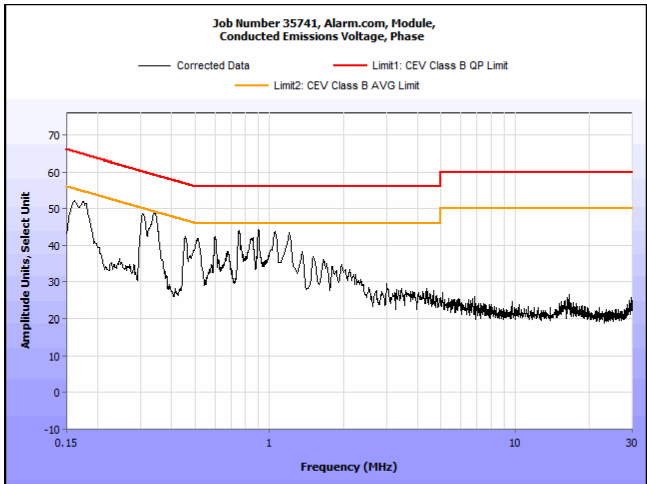
Plot 4. Conducted Emissions, 15.207(a), Phase Line
