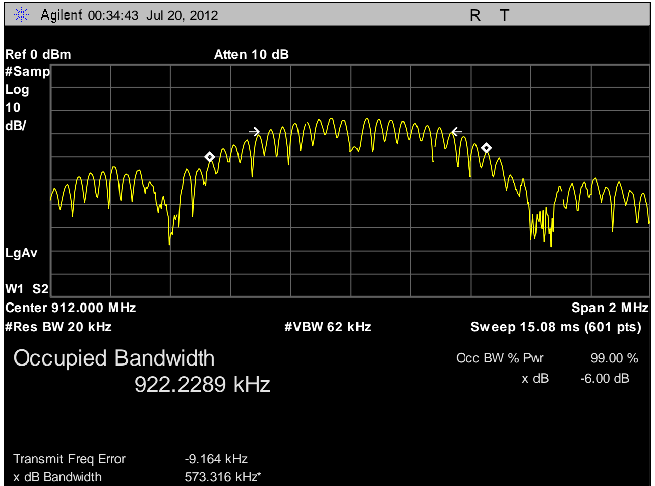
Plot 9. 99% Occupied Bandwidth, Low Channel
