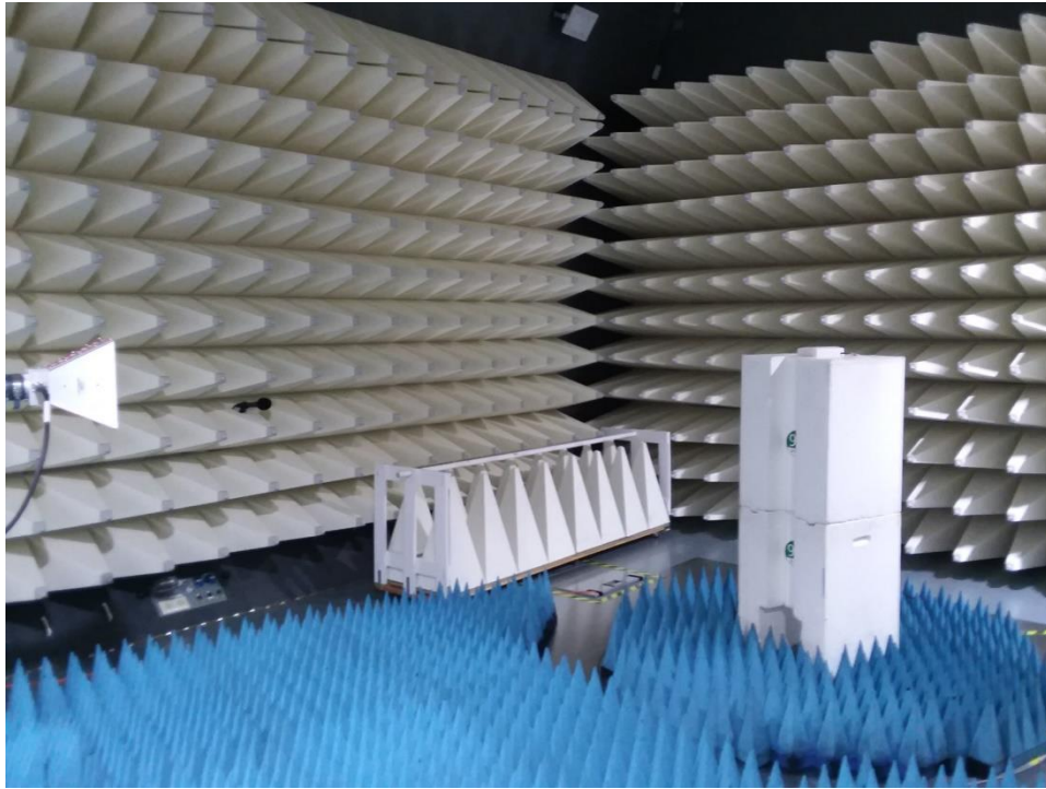
Figure B5. High Range Radiated Emission test setup
