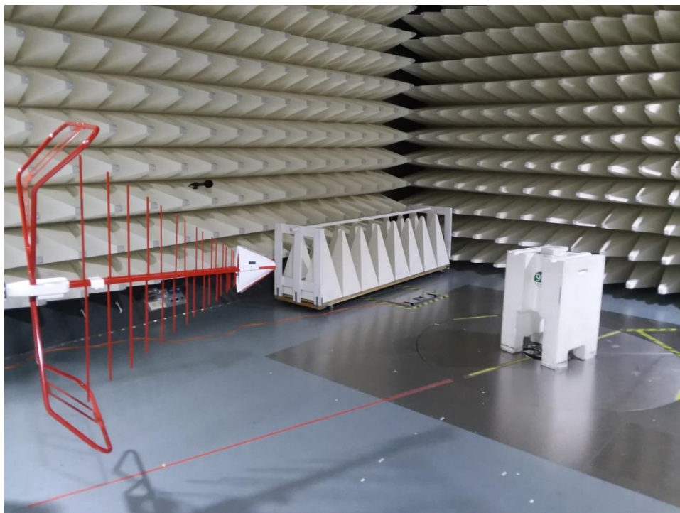
Figure B4. Low Range Radiated Emission test setup
