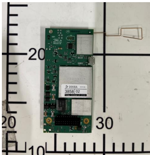
Figure B4. Rear View of DUT with Concord antenna
