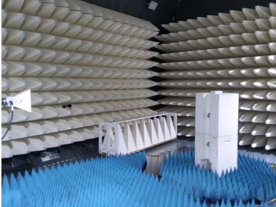
Figure B9. High Range Radiated Emission test setup
