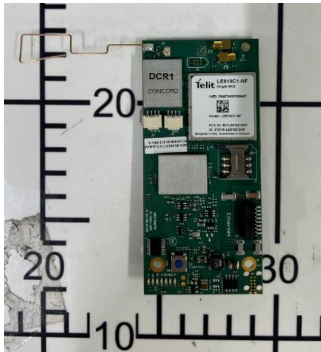
Figure B3. Front View of DUT with Concord antenna
