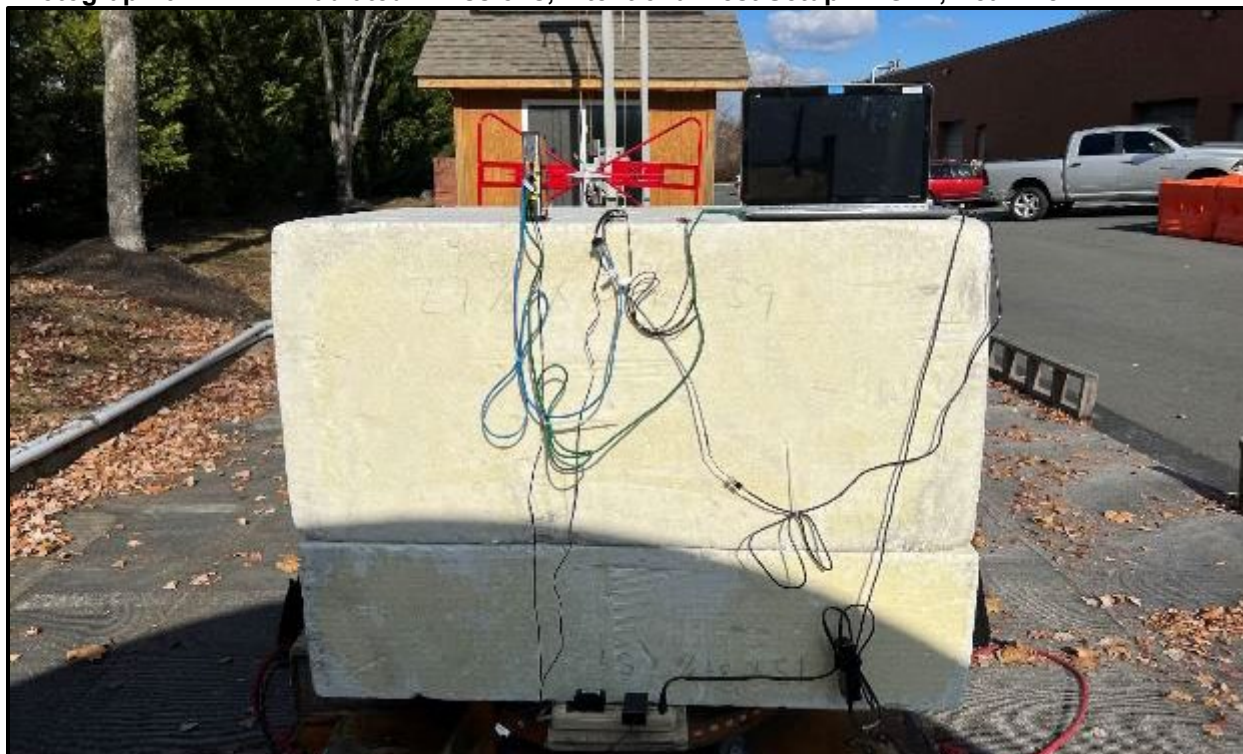
Photograph 6: Radiated Emissions, Intentional Test Setup >1 GHz, Rear View
