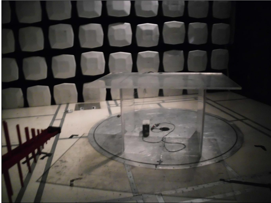
Photograph 3. Radiated Spurious, Test Setup
