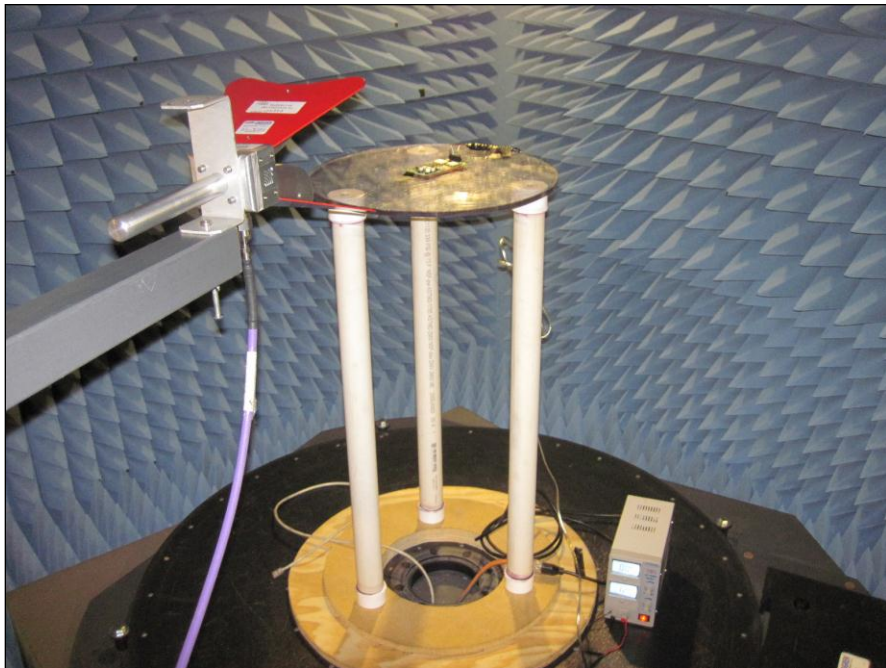
Photograph 4. Radiated Spurious, Test Setup, Above 1 GHz
