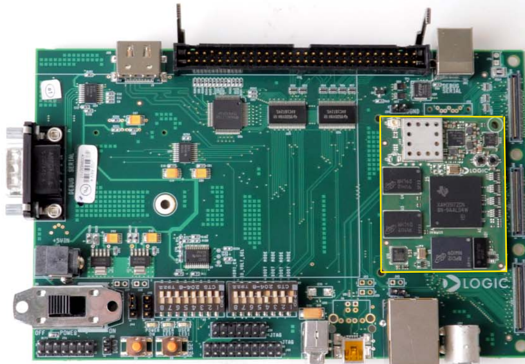
AM3X SOM-M2 (OUTLINED IN YELLOW) ATTACHED TO APPLICATION BASEBOARD
