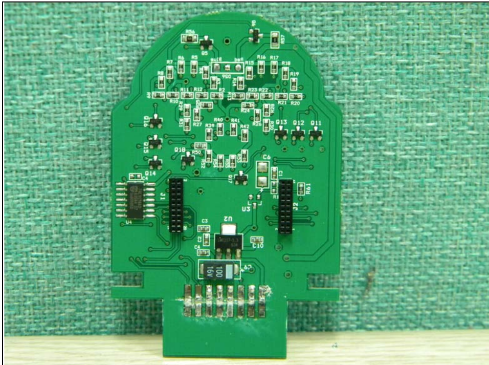
Bottom view of LED board
