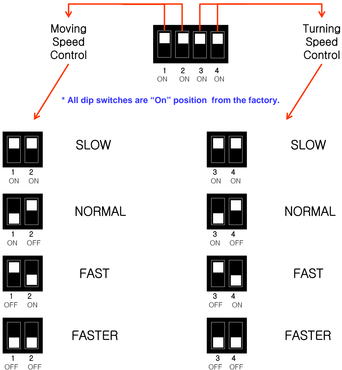
< The location of Robot Speed Control Dip Switch >
