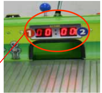
Score FND
