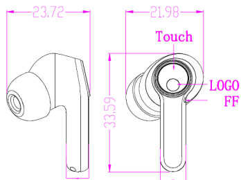
Bluetooth heast
