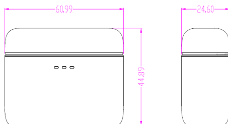
Charging box
