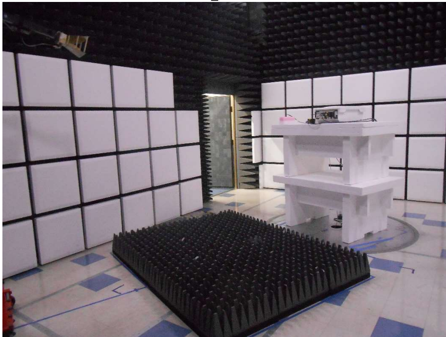
RF Radiated_ above 1 GHz #1
