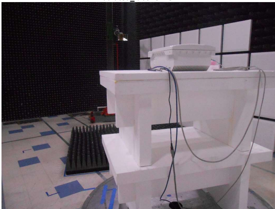
RF Radiated_ above 1 GHz #2
