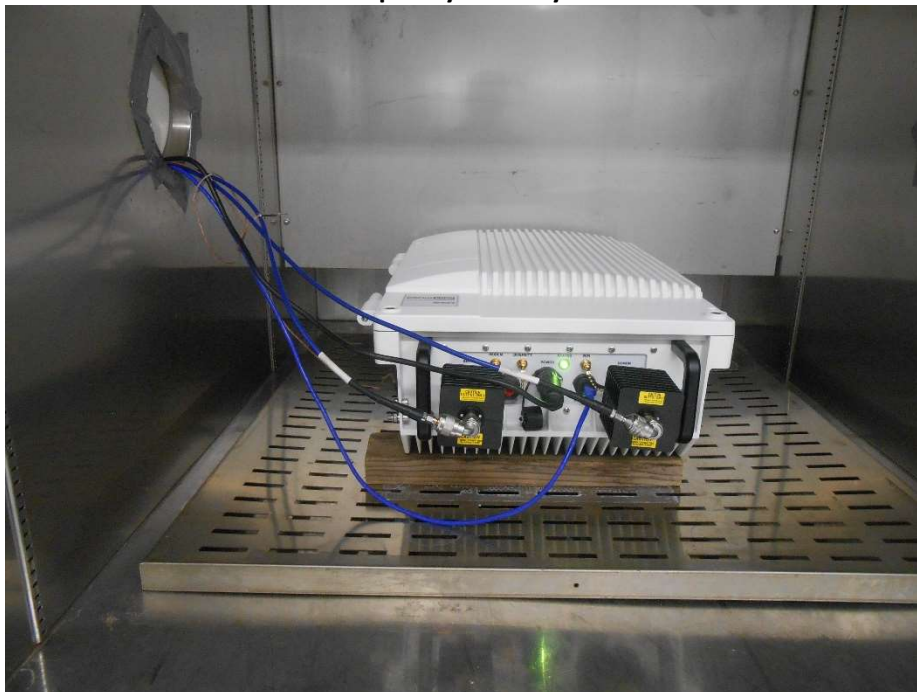
Frequency Stability #1
