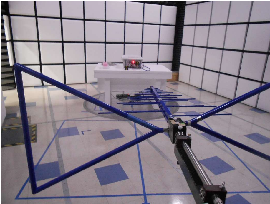
RF Radiated_ below 1 GHz #1
