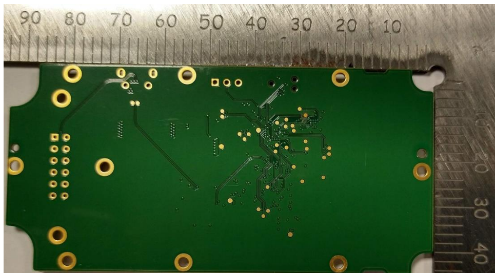
Figure 2 - External Bottom
