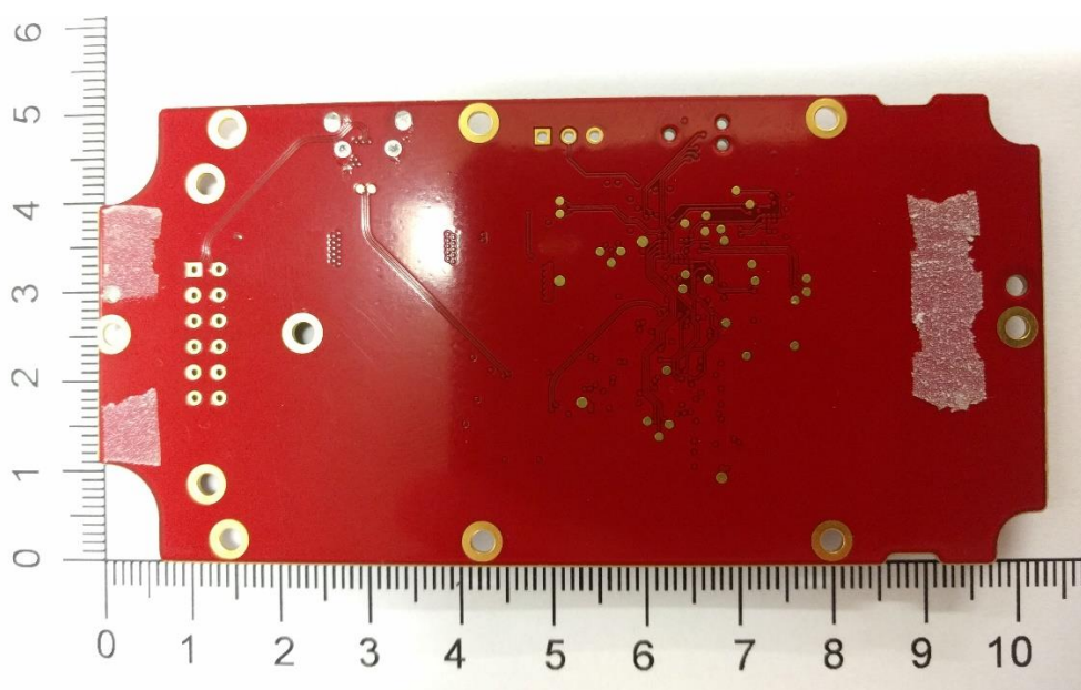
Figure 2- External Bottom
