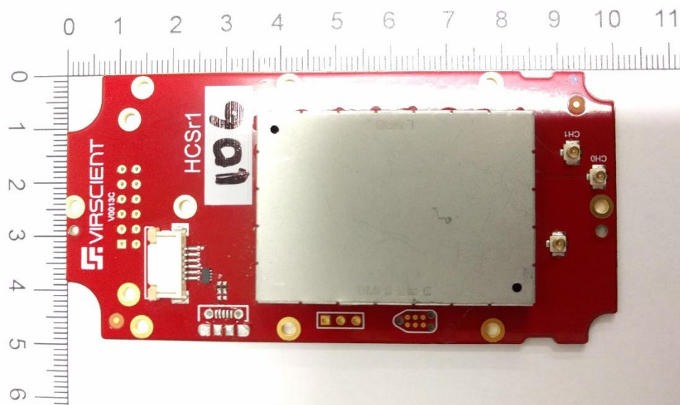
Figure 1 - External Top
