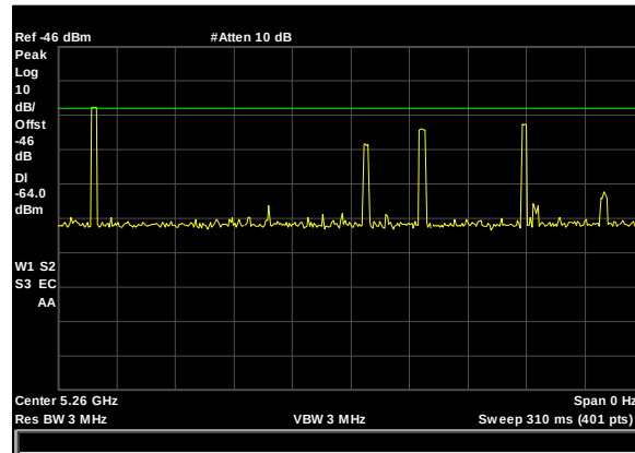
Plot 7. Radar Waveform Calibration, 5260 MHz, Type 6, 20 MHz
