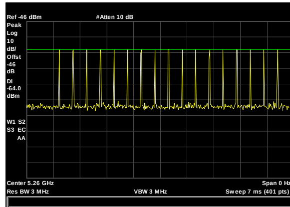
Plot 4. Radar Waveform Calibration, 5260 MHz, Type 3, 20 MHz
