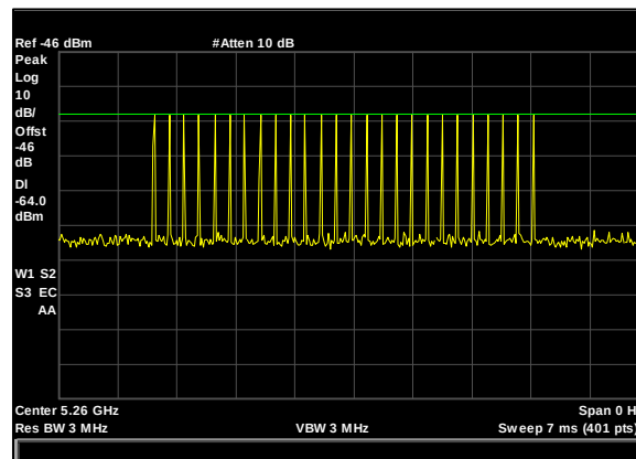
Plot 3. Radar Waveform Calibration, 5260 MHz, Type 2, 20 MHz
