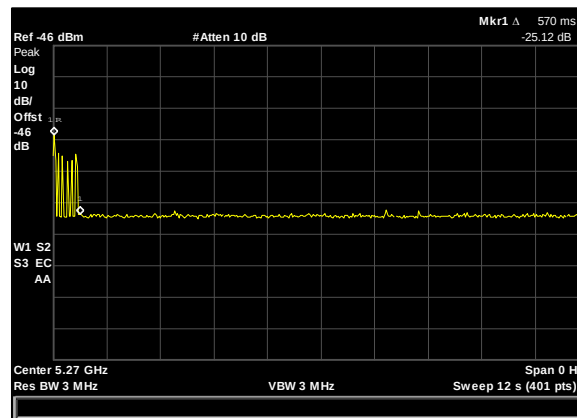
Plot 19. Channel Move Time
