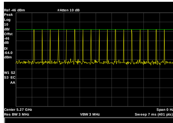
Plot 11. Radar Waveform Calibration, 5270 MHz, Type 3, 40 MHz
