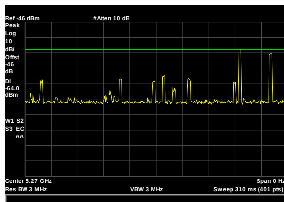
Plot 14. Radar Waveform Calibration, 5270 MHz, Type 6, 40 MHz
