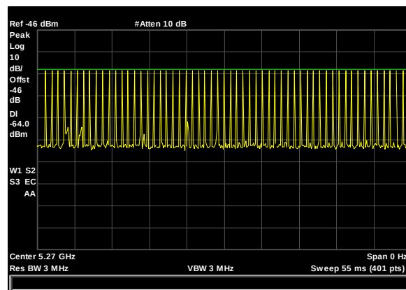
Plot 9. Radar Waveform Calibration, 5270 MHz, Type 1, 40 MHz
