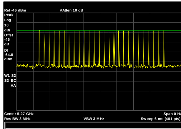
Plot 10. Radar Waveform Calibration, 5270 MHz, Type 2, 40 MHz
