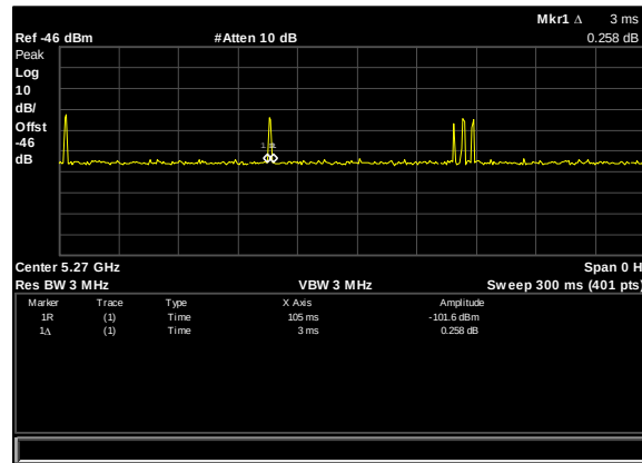
Plot 18. Channel Close Time
