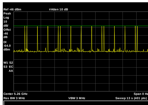
Plot 6. Radar Waveform Calibration, 5260 MHz, Type 5, 20 MHz
