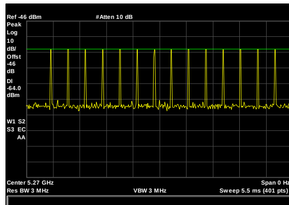
Plot 12. Radar Waveform Calibration, 5270 MHz, Type 4, 40 MHz
