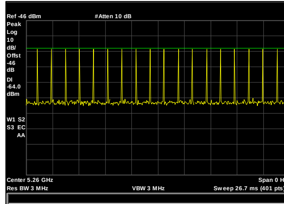
Plot 1. Radar Waveform Calibration, 5260 MHz, Type 0, 20 MHz
