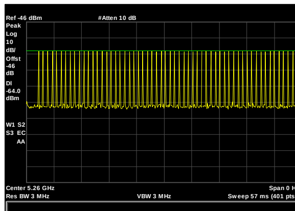
Plot 2. Radar Waveform Calibration, 5260 MHz, Type 1, 20 MHz
