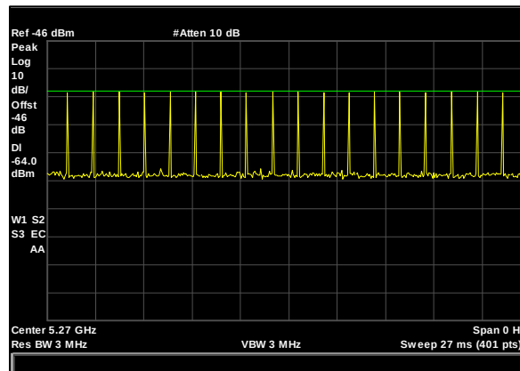
Plot 8. Radar Waveform Calibration, 5270 MHz, Type 0, 40 MHz
