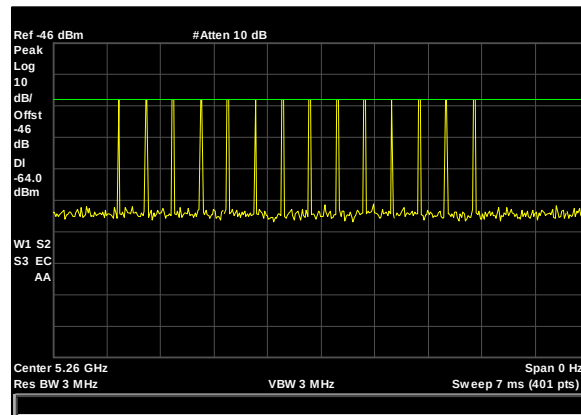
Plot 5. Radar Waveform Calibration, 5260 MHz, Type 4, 20 MHz
