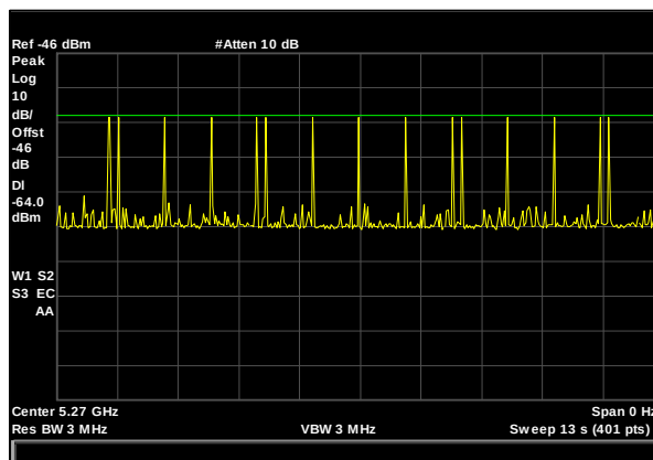
Plot 13. Radar Waveform Calibration, 5270 MHz, Type 5, 40 MHz
