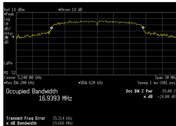
Plot 9. 26 dB Occupied Bandwidth, 26 dB, BW 20 M, Ch. 5240 MHz, A mode, ANT 0
