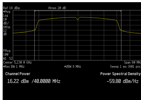
Plot 32. Conducted Output Power, BW 40M, Ch. 5230 MHz, N mode, ANT 0
