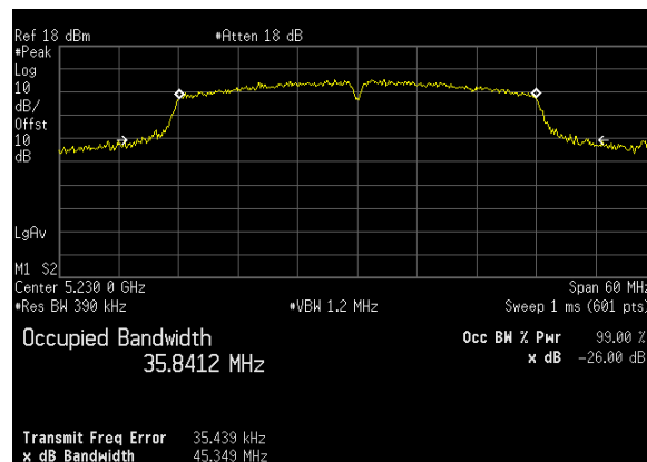
Plot 16. 26 dB Occupied Bandwidth, 26 dB, BW 40 M, Ch. 5230 MHz, N mode, ANT 1
