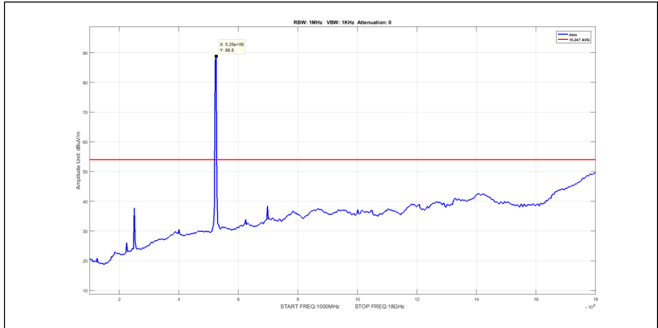
Plot 81. Undesirable Emissions, Average Spurious Emission 1-18GHz, BW 20M, Ch 5240M, A Mode ANT 1 (worst-case) V
