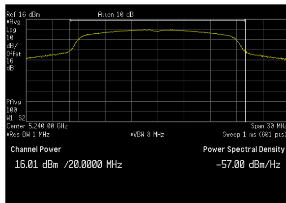
Plot 29. Conducted Output Power, BW 20M, Ch. 5240 MHz, N mode, ANT 1
