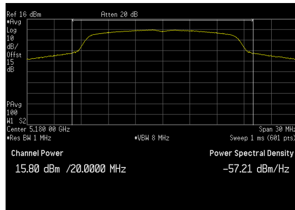
Plot 19. Conducted Output Power, BW 20M, Ch. 5180 MHz, A mode, ANT 1
