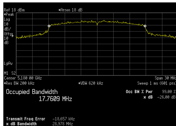
Plot 4. 26 dB Occupied Bandwidth, 26 dB, BW 20 M, Ch. 5180 MHz, N mode, ANT 1
