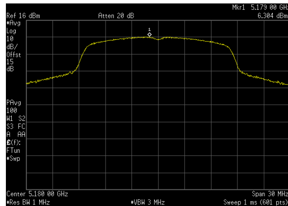
Plot 36. Power Spectral Density, BW 20 M, Ch. 5180 MHz, A mode, ANT 0
