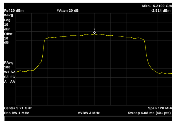
Plot 52. Power Spectral Density, BW 80 M, Ch. 5210 MHz, AC mode, ANT 0
