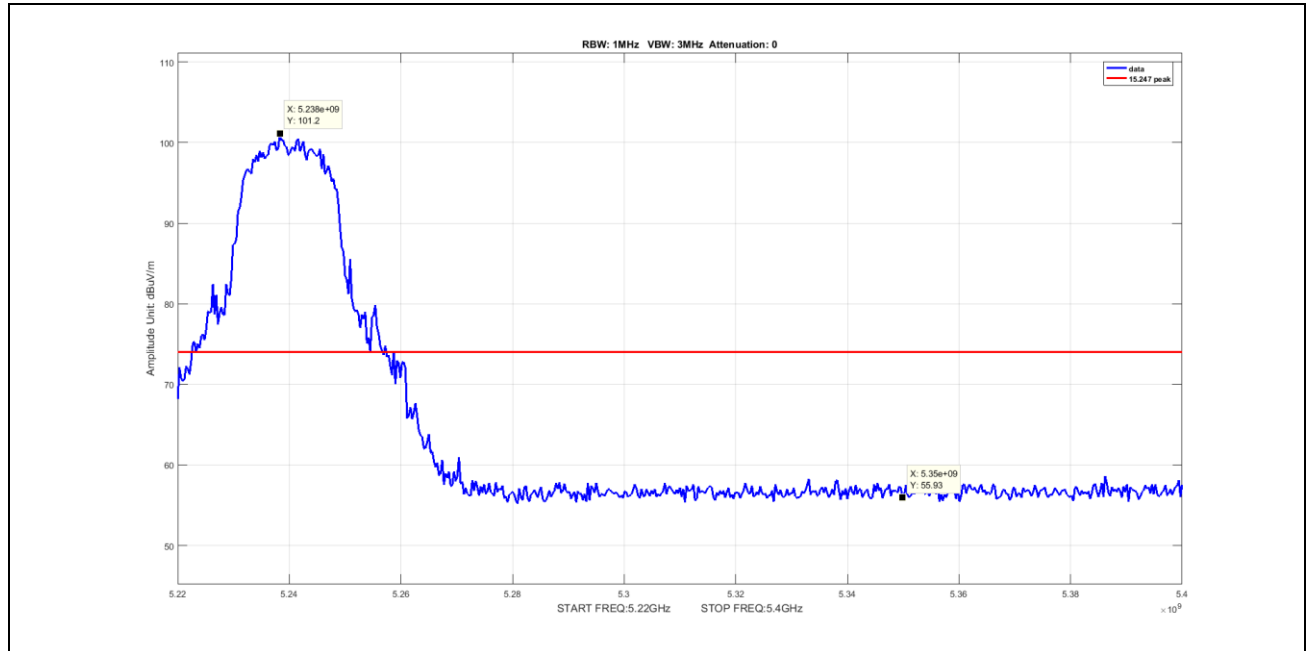
Plot 70. Undesirable Emissions, Peak Band Edge Spurious, BW 20M, Ch 5240M, N Mode ANT 0 (worst-case) V
