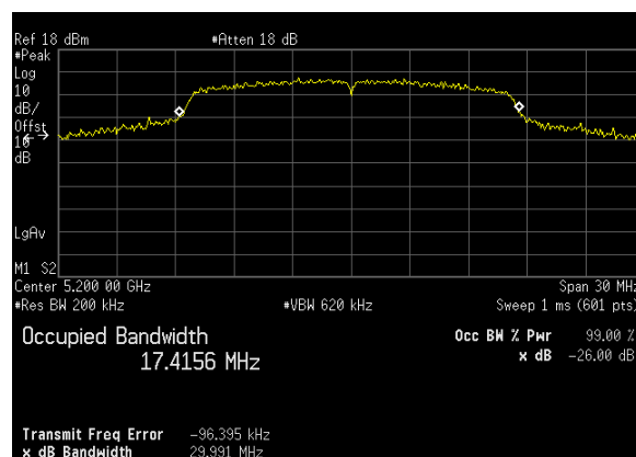
Plot 5. 26 dB Occupied Bandwidth, 26 dB, BW 20 M, Ch. 5200 MHz, A mode, ANT 0
