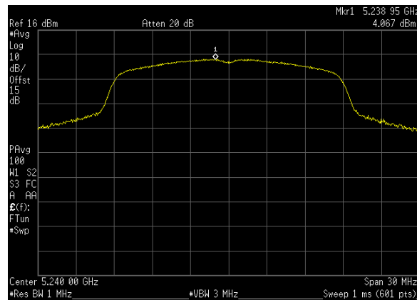
Plot 47. Power Spectral Density, BW 20 M, Ch. 5240 MHz, N mode, ANT 1
