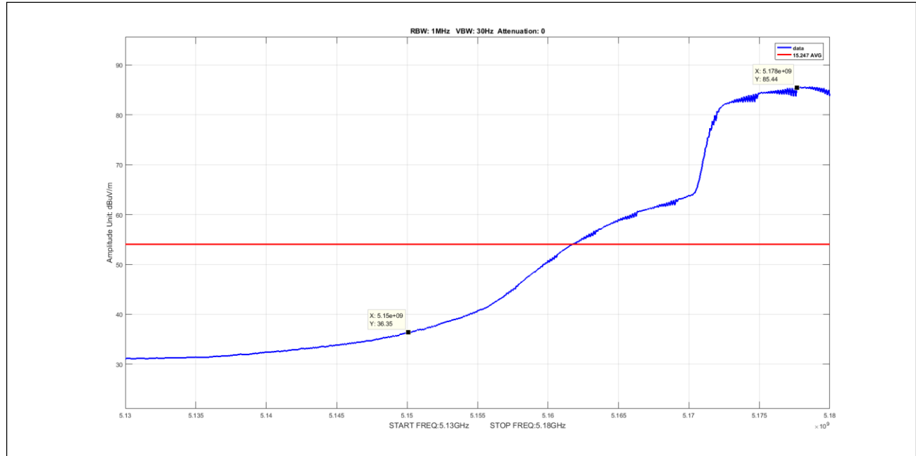
Plot 54. Undesirable Emissions, Average Band Edge Spurious, BW 20M, Ch 5180M, A Mode ANT 1 (worst-case) V
