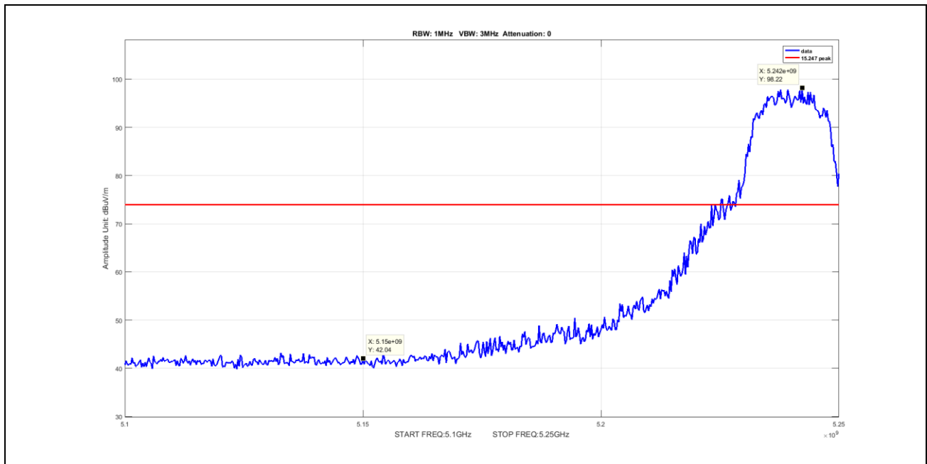
Plot 67. Undesirable Emissions, Peak Band Edge Spurious, BW 20M, Ch 5240M, A Mode ANT 1 (worst-case) V
