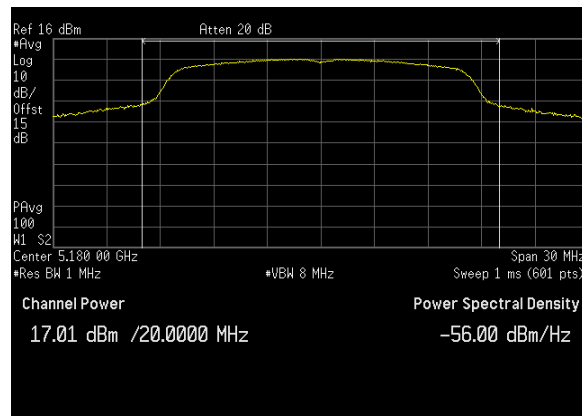
Plot 18. Conducted Output Power, BW 20M, Ch. 5180 MHz, A mode, ANT 0
