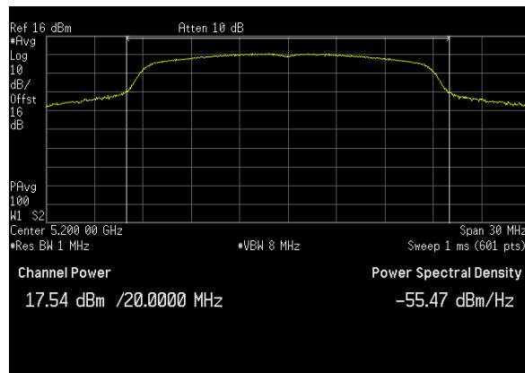
Plot 24. Conducted Output Power, BW 20M, Ch. 5200 MHz, N mode, ANT 0
