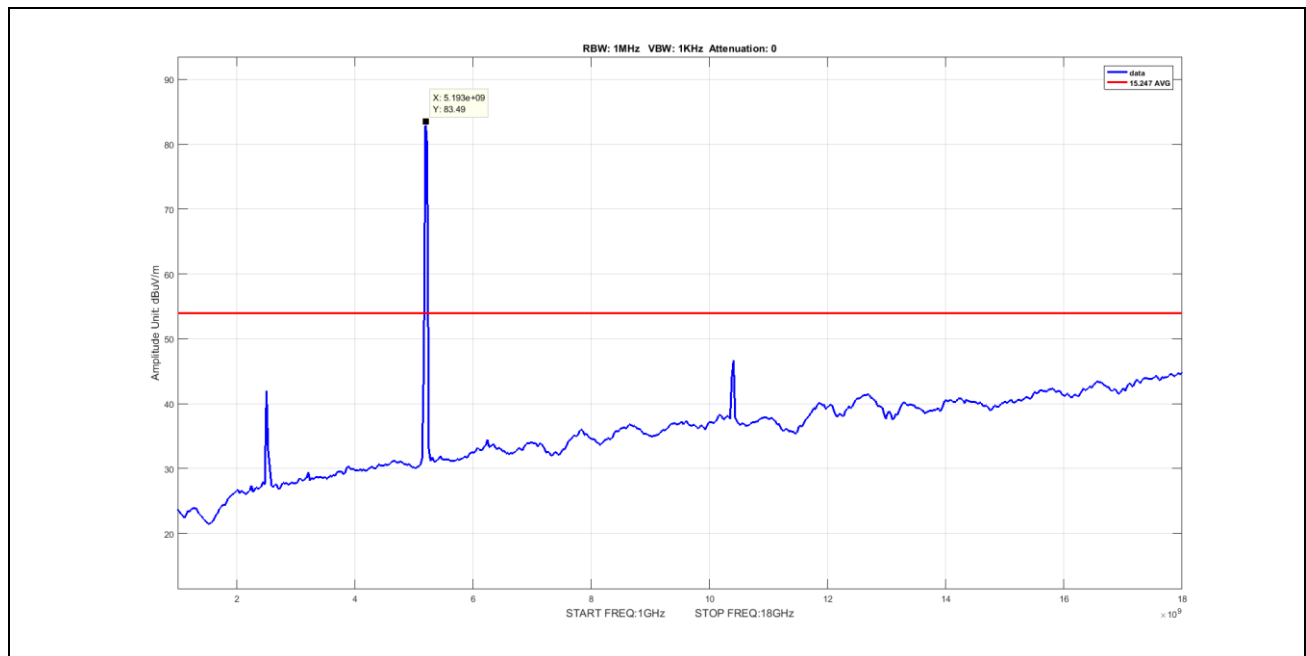
Plot 80. Undesirable Emissions, Average Spurious Emission 1-18GHz, BW 20M, Ch 5200M, N Mode ANT 0 (worst-case) V
