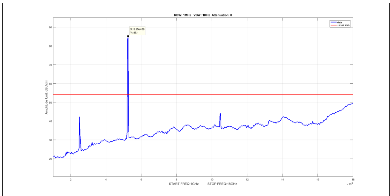
Plot 82. Undesirable Emissions, Average Spurious Emission 1-18GHz, BW 20M, Ch 5240M, A Mode ANT 0 (worst-case) V
