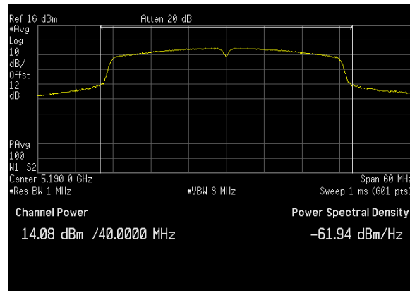
Plot 31. Conducted Output Power, BW 40M, Ch. 5190 MHz, N mode, ANT 1
