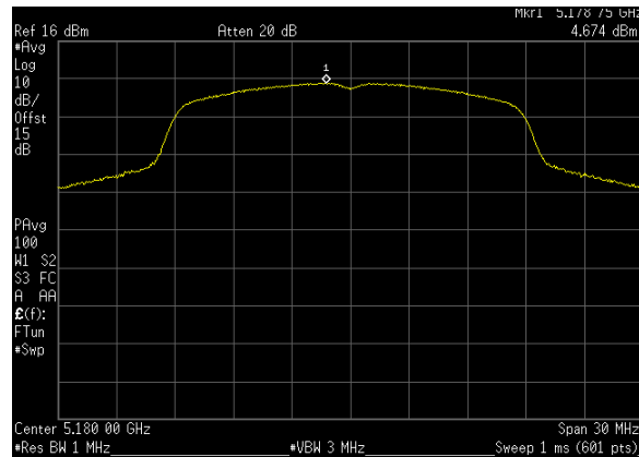
Plot 39. Power Spectral Density, BW 20 M, Ch. 5180 MHz, N mode, ANT 1
