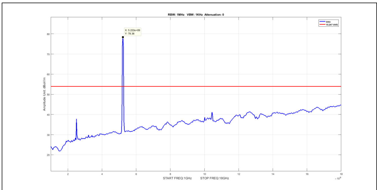
Plot 88. Undesirable Emissions, Average Spurious Emission 1-18GHz, BW 40M, Ch 5230M, N Mode ANT 0 (worst-case) V
