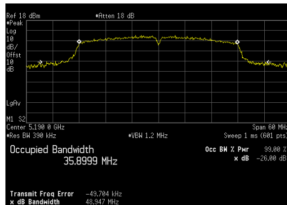
Plot 14. 26 dB Occupied Bandwidth, 26 dB, BW 40 M, Ch.5190 MHz, N mode, ANT 1
