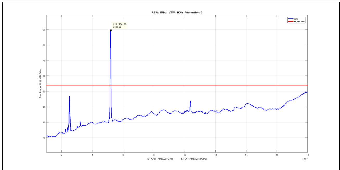
Plot 74. Undesirable Emissions, Average Spurious Emission 1-18GHz, BW 20M, Ch 5180M, A Mode ANT 0 (worst-case) V
