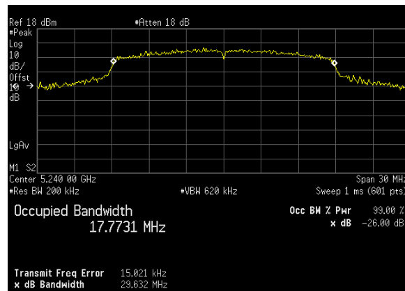
Plot 12. 26 dB Occupied Bandwidth, 26 dB, BW 20 M, Ch. 5240 MHz, N mode, ANT 1
