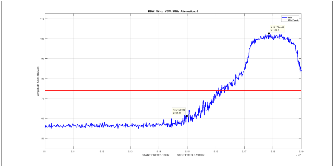
Plot 64. Undesirable Emissions, Peak Band Edge Spurious, BW 20M, Ch 5180M, A Mode ANT 0 (worst-case) V
