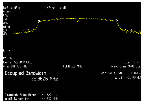
Plot 15. 26 dB Occupied Bandwidth, 26 dB, BW 40 M, Ch. 5230 MHz, N mode, ANT 0
