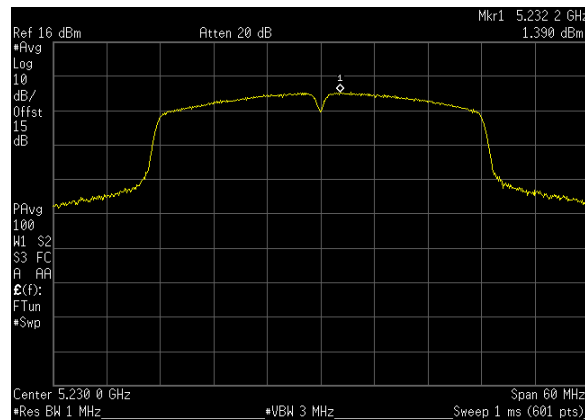
Plot 50. Power Spectral Density, BW 40 M, Ch. 5230 MHz, N mode, ANT 0
