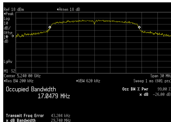
Plot 10. 26 dB Occupied Bandwidth, 26 dB, BW 20 M, Ch. 5240 MHz, A mode, ANT 1
