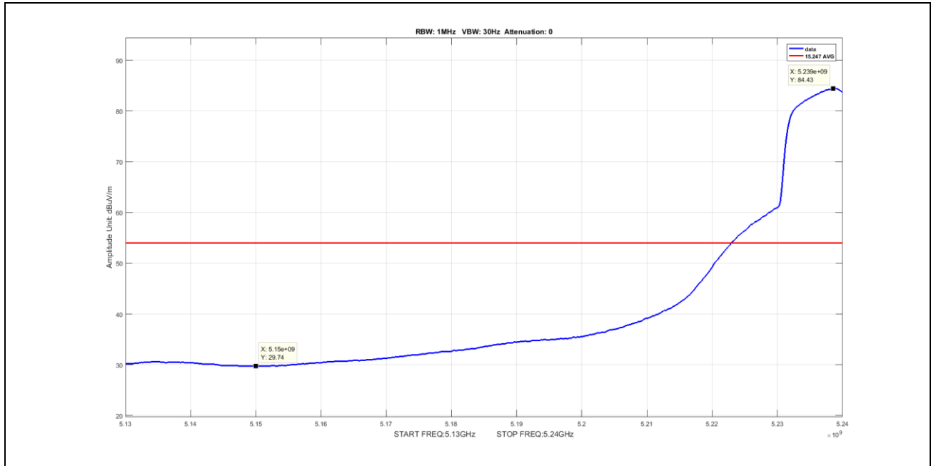
Plot 58. Undesirable Emissions, Average Band Edge Spurious, BW 20M, Ch 5240M, A Mode ANT 1 (worst-case) V
