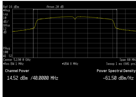
Plot 30. Conducted Output Power, BW 40M, Ch. 5190 MHz, N mode, ANT 0
