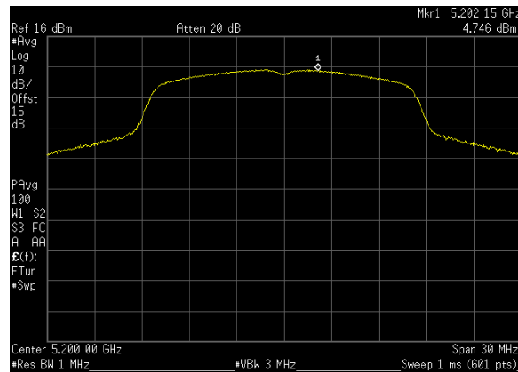
Plot 41. Power Spectral Density, BW 20 M, Ch. 5200 MHz, A mode, ANT 1
