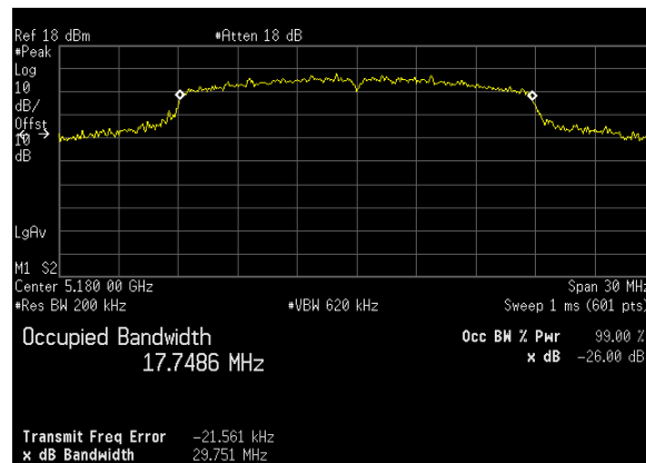
Plot 3. 26 dB Occupied Bandwidth, 26 dB, BW 20 M, Ch. 5180 MHz, N mode, ANT 0
