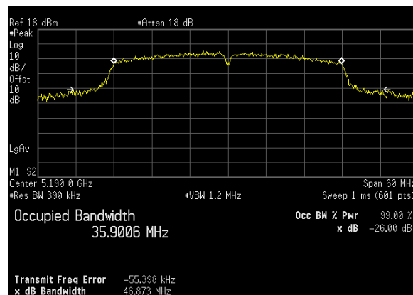
Plot 13. 26 dB Occupied Bandwidth, 26 dB, BW 40 M, Ch. 5190MHz, N mode, ANT 0
