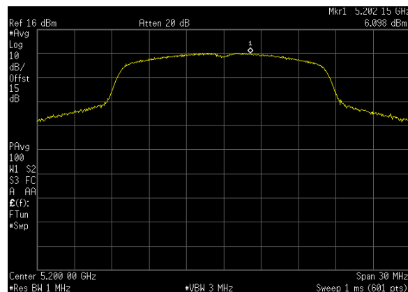
Plot 40. Power Spectral Density, BW 20 M, Ch. 5200 MHz, A mode, ANT 0
