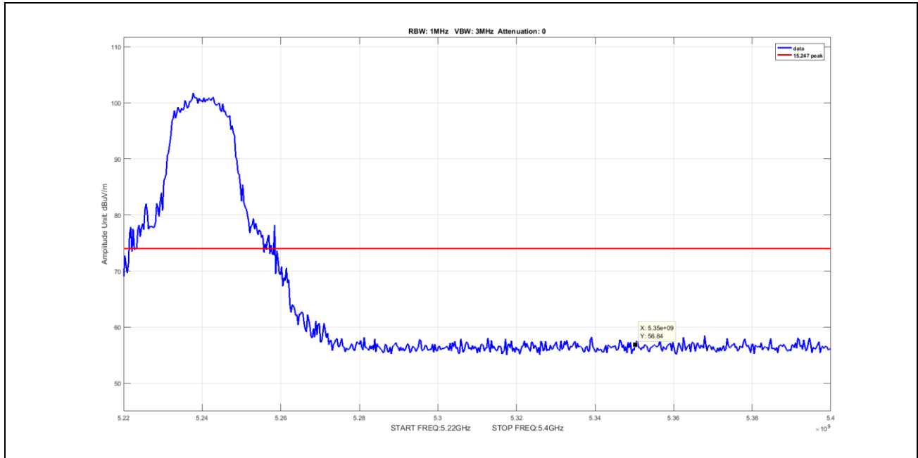
Plot 68. Undesirable Emissions, Peak Band Edge Spurious, BW 20M, Ch 5240M, A Mode ANT 0 (worst-case) V
