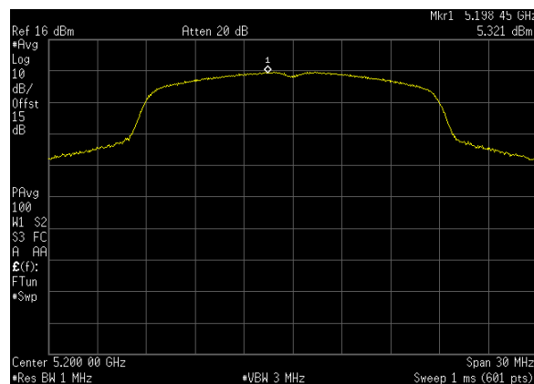
Plot 42. Power Spectral Density, BW 20 M, Ch. 5200 MHz, N mode, ANT 0
