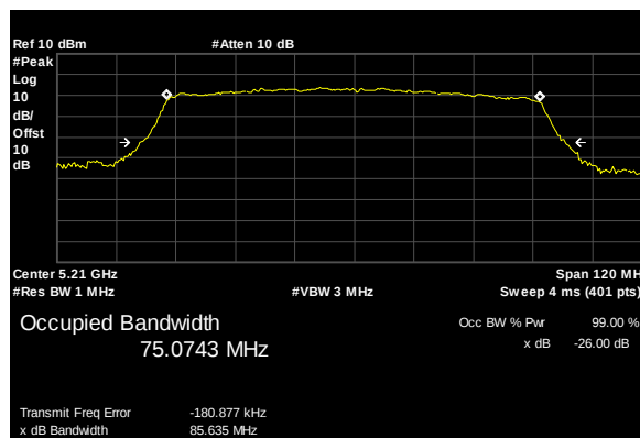
Plot 17. 26 dB Occupied Bandwidth, 26 dB, BW 80M, CH. 5210 MHz, AC Mode, ANT 0
