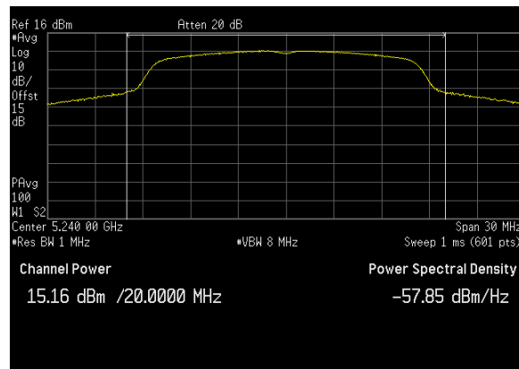
Plot 27. Conducted Output Power, BW 20M, Ch. 5240 MHz, A mode, ANT 1
