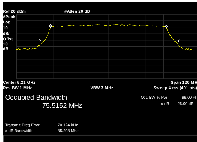
Plot 18. 26 dB Occupied Bandwidth, 26 dB, BW 80M, CH. 5210 MHz, AC Mode, ANT 1
