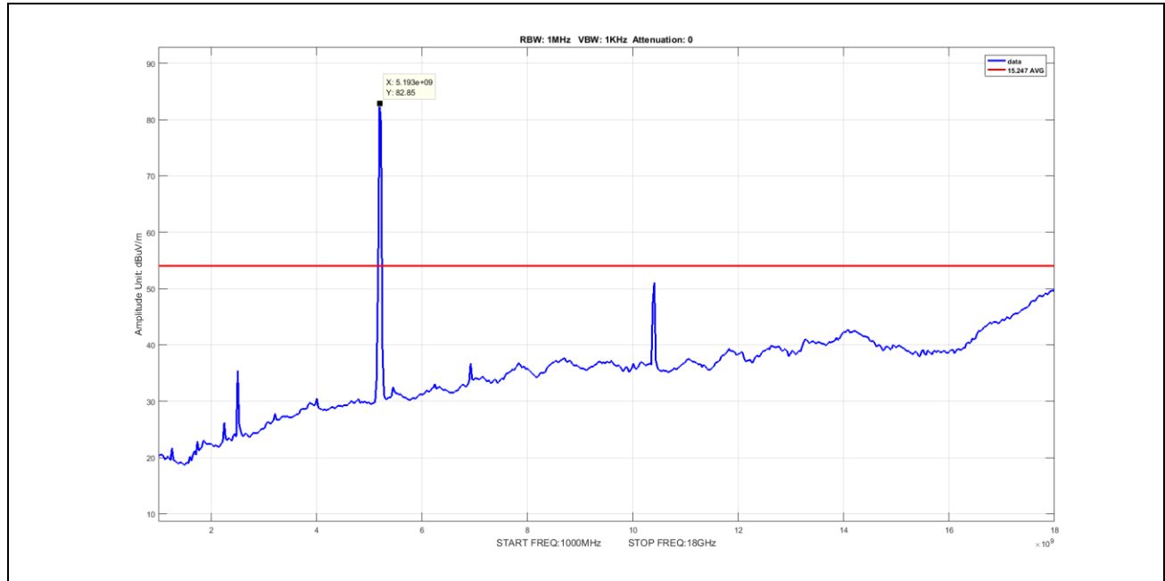
Plot 77. Undesirable Emissions, Average Spurious Emission 1-18GHz, BW 20M, Ch 5200M, A Mode ANT 1 (worst-case) V
