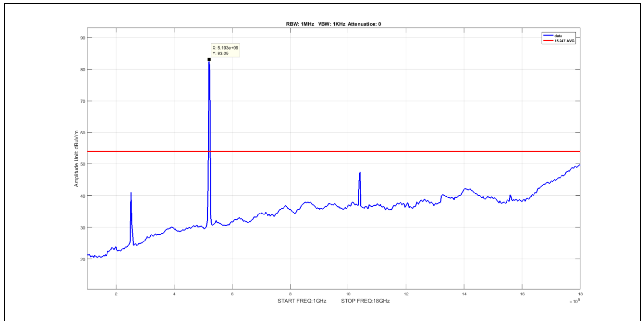
Plot 78. Undesirable Emissions, Average Spurious Emission 1-18GHz, BW 20M, Ch 5200M, A Mode ANT 0 (worst-case) V
