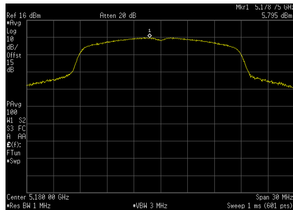
Plot 38. Power Spectral Density, BW 20 M, Ch. 5180 MHz, N mode, ANT 0
