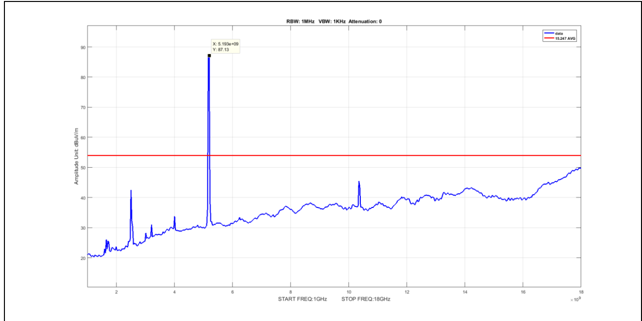
Plot 73. Undesirable Emissions, Average Spurious Emission 1-18GHz, BW 20M, Ch 5180M, A Mode ANT 1 (worst-case) V
