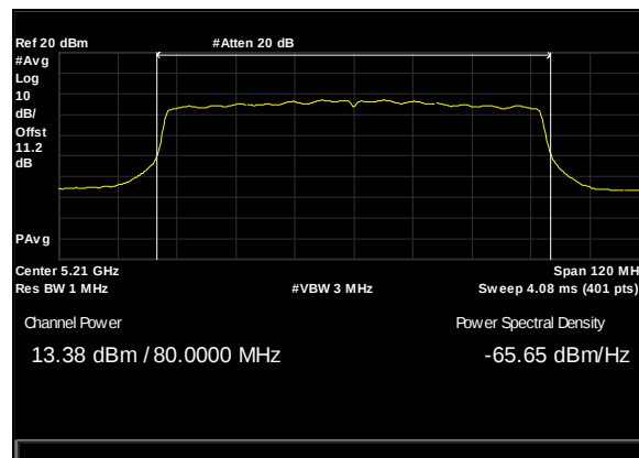
Plot 35. Conducted Output Power, BW 80M, CH. 5210 MHz, AC Mode, ANT 1
