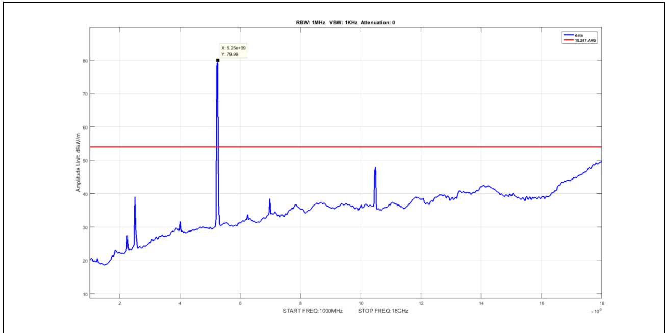
Plot 83. Undesirable Emissions, Average Spurious Emission 1-18GHz, BW 20M, Ch 5240M, N Mode ANT 1 (worst-case) V
