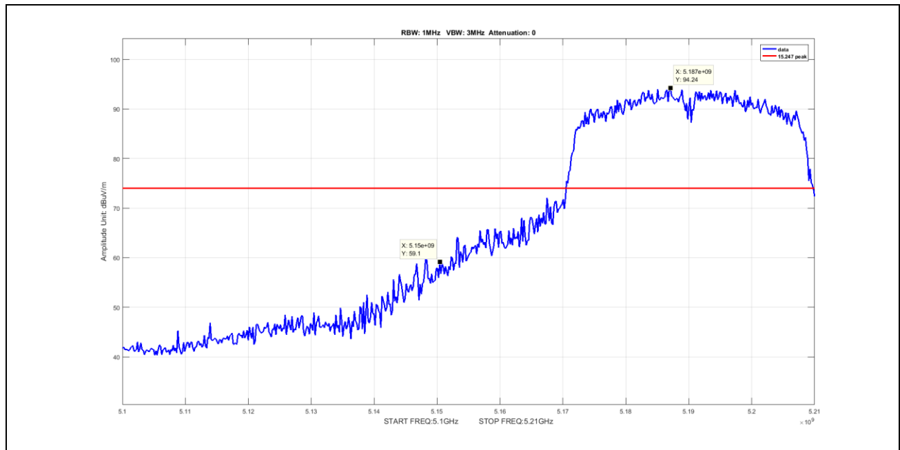
Plot 71. Undesirable Emissions, Peak Band Edge Spurious, BW 40M, Ch 5190M, N Mode ANT 1 (worst-case) V
