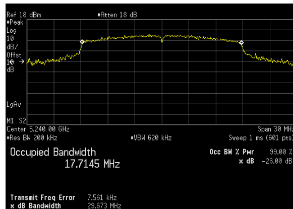
Plot 11. 26 dB Occupied Bandwidth, 26 dB, BW 20 M, Ch. 5240 MHz, N mode, ANT 0
