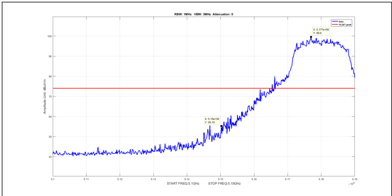
Plot 63. Undesirable Emissions, Peak Band Edge Spurious, BW 20M, Ch 5180M, A Mode ANT 1 (worst-case) V
