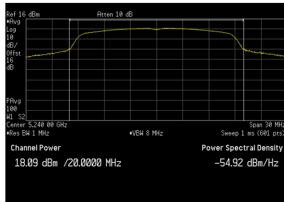
Plot 28. Conducted Output Power, BW 20M, Ch. 5240 MHz, N mode, ANT 0
