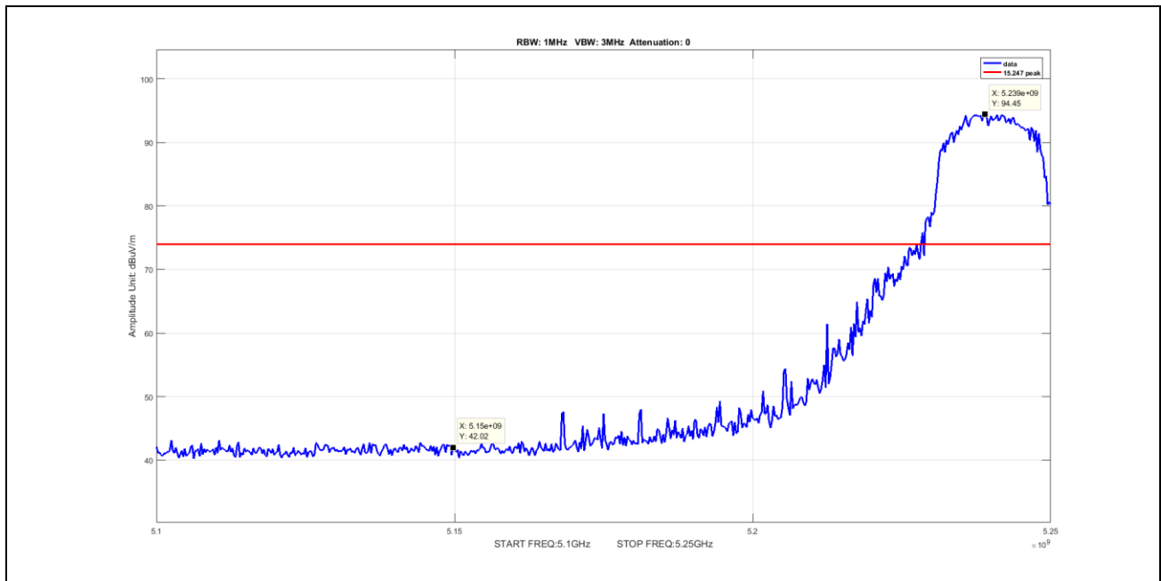
Plot 69. Undesirable Emissions, Peak Band Edge Spurious, BW 20M, Ch 5240M, N Mode ANT 1 (worst-case) V
