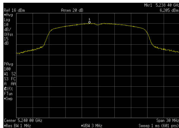
Plot 46. Power Spectral Density, BW 20 M, Ch. 5240 MHz, N mode, ANT 0
