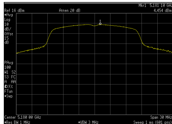
Plot 37. Power Spectral Density, BW 20 M, Ch. 5180 MHz, A mode, ANT 1
