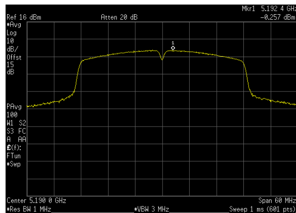
Plot 49. Power Spectral Density, BW 40 M, Ch. 5190 MHz, N mode, ANT 1
