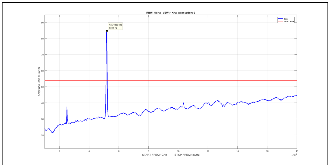
Plot 86. Undesirable Emissions, Average Spurious Emission 1-18GHz, BW 40M, Ch 5190M, N Mode ANT 0 (worst-case) V
