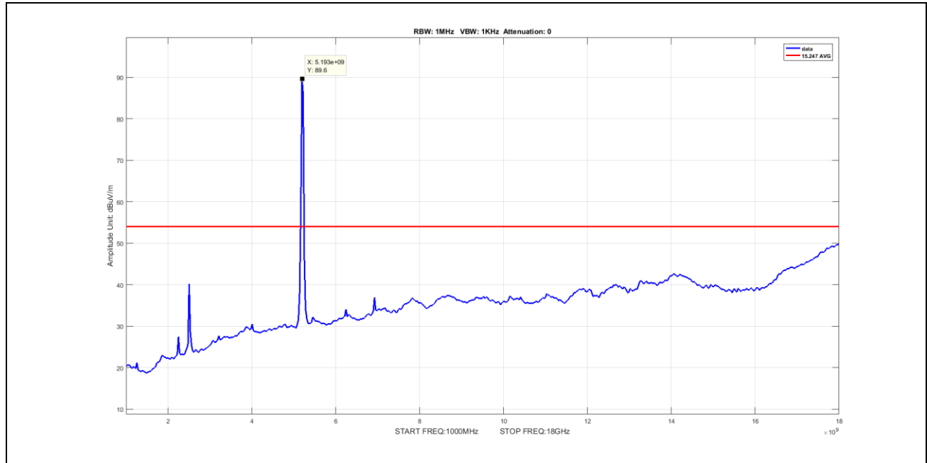
Plot 79. Undesirable Emissions, Average Spurious Emission 1-18GHz, BW 20M, Ch 5200M, N Mode ANT 1 (worst-case) V
