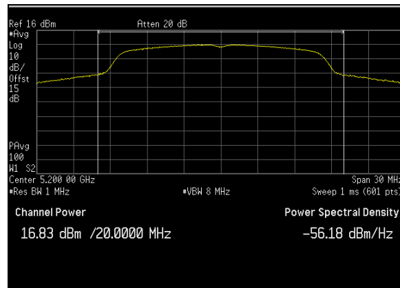
Plot 22. Conducted Output Power, BW 20M, Ch. 5200 MHz, A mode, ANT 0
