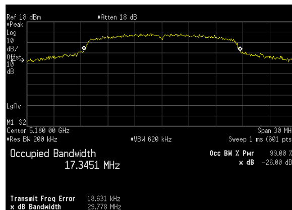
Plot 1. 26 dB Occupied Bandwidth, 26 dB, BW 20 M, Ch. 5180 MHz, A mode, ANT 0
