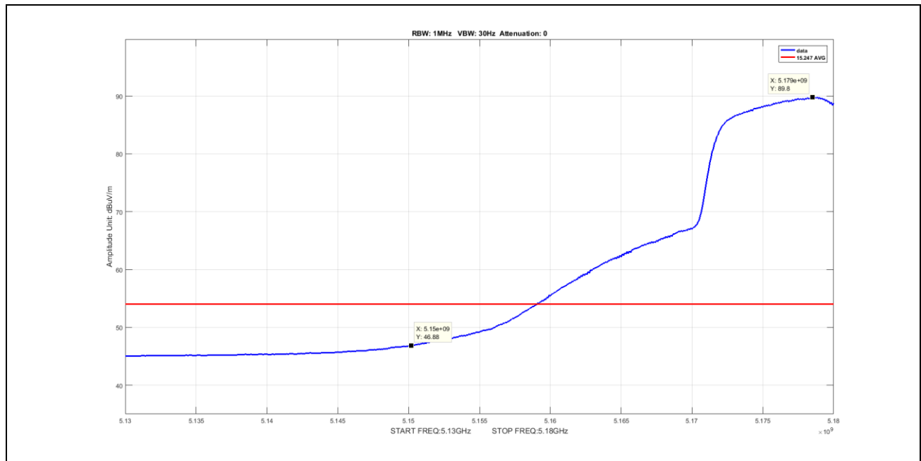
Plot 55. Undesirable Emissions, Average Band Edge Spurious, BW 20M, Ch 5180M, A Mode ANT 0 (worst-case) V
