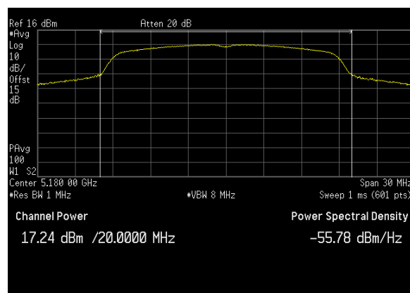
Plot 20. Conducted Output Power, BW 20M, Ch. 5180 MHz, N mode, ANT 0
