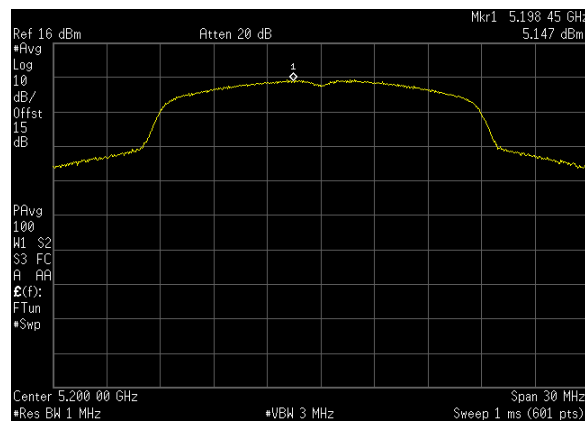
Plot 43. Power Spectral Density, BW 20 M, Ch. 5200 MHz, N mode, ANT 1
