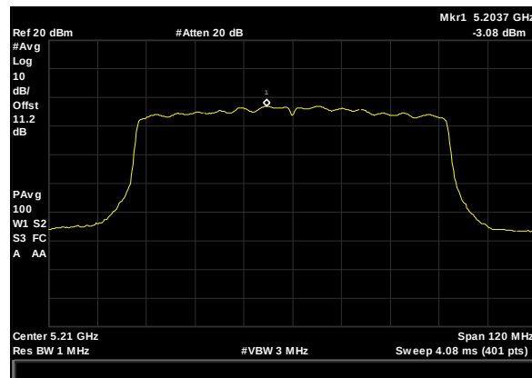
Plot 53. Power Spectral Density, BW 80 M, Ch. 5210 MHz, AC mode, ANT 1
