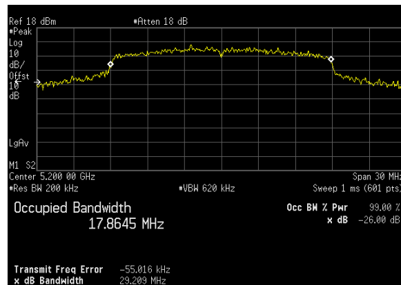
Plot 7. 26 dB Occupied Bandwidth, 26 dB, BW 20 M, Ch. 5200 MHz, N mode, ANT 0
