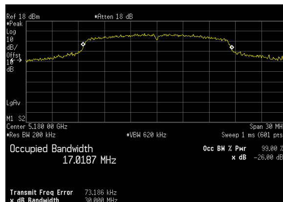
Plot 2. 26 dB Occupied Bandwidth, 26 dB, BW 20 M, Ch. 5180 MHz, A mode, ANT 1
