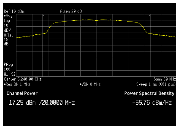
Plot 26. Conducted Output Power, BW 20M, Ch. 5240 MHz, A mode, ANT 0
