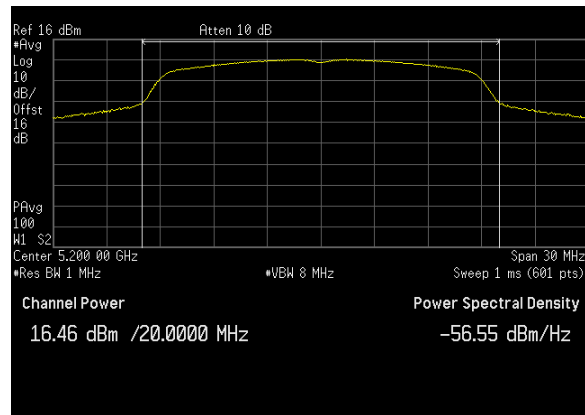
Plot 25. Conducted Output Power, BW 20M, Ch. 5200 MHz, N mode, ANT 1
