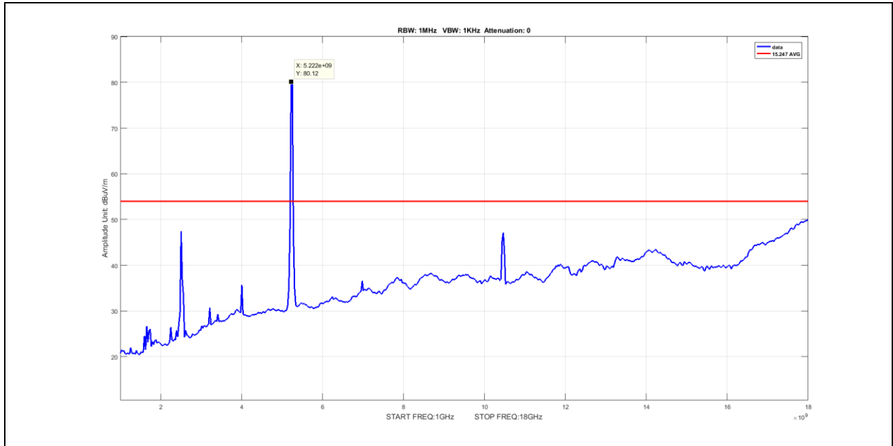
Plot 87. Undesirable Emissions, Average Spurious Emission 1-18GHz, BW 40M, Ch 5230M, N Mode ANT 1 (worst-case) V
