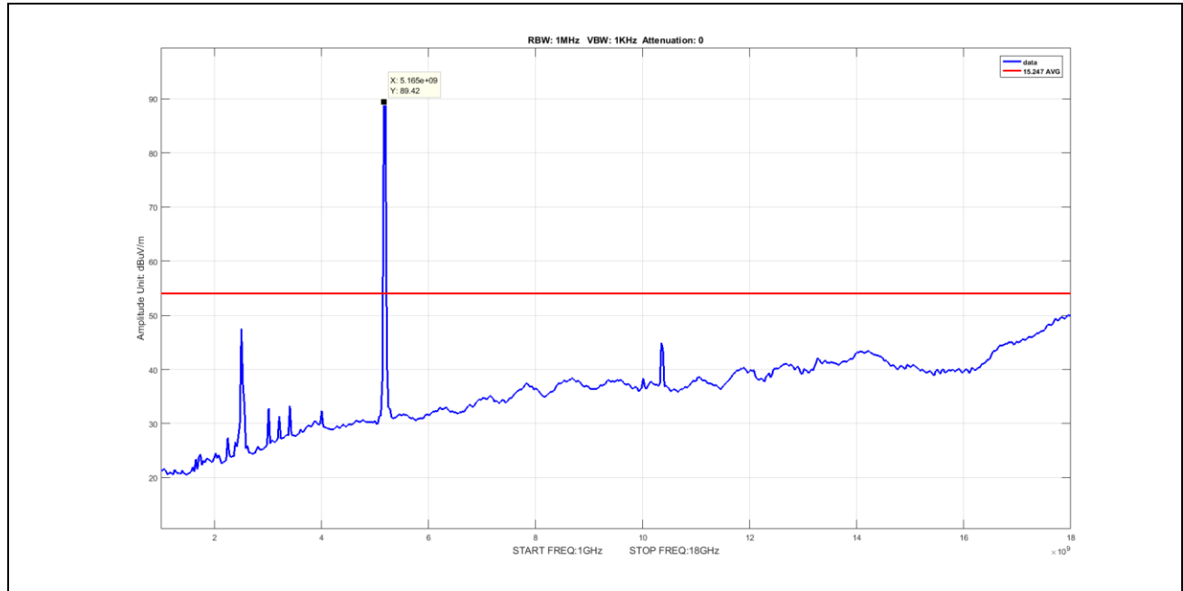
Plot 75. Undesirable Emissions, Average Spurious Emission 1-18GHz, BW 20M, Ch 5180M, N Mode ANT 1 (worst-case) V
