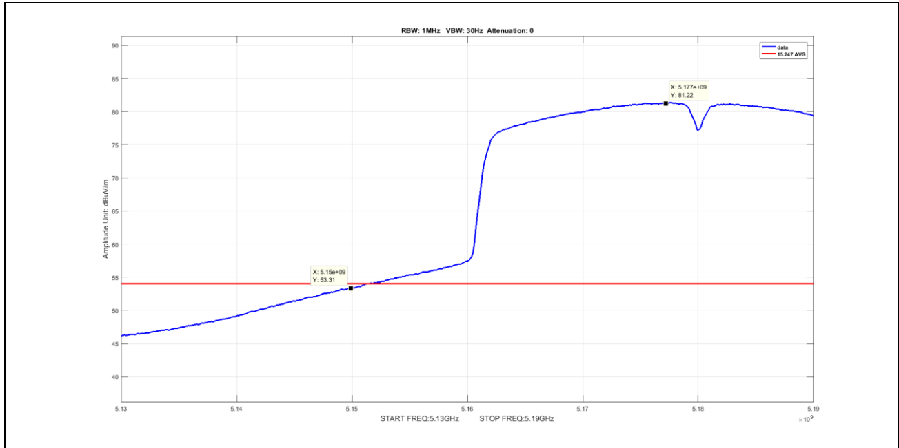
Plot 62. Undesirable Emissions, Average Band Edge Spurious, BW 40M, Ch 5190M, N Mode ANT 0 (worst-case) V
