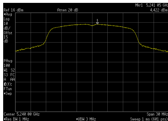
Plot 45. Power Spectral Density, BW 20 M, Ch. 5240 MHz, A mode, ANT 1
