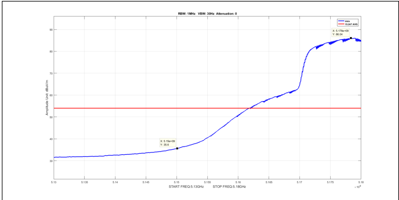
Plot 56. Undesirable Emissions, Average Band Edge Spurious, BW 20M, Ch 5180M, N Mode ANT 1 (worst-case) V
