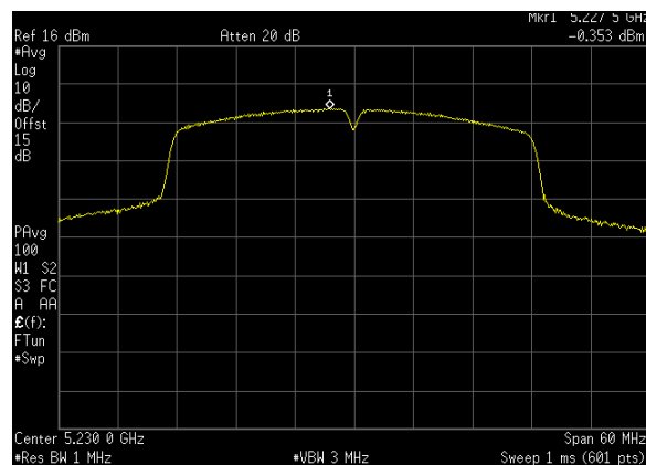
Plot 51. Power Spectral Density, BW 40 M, Ch. 5230 MHz, N mode, ANT 1
