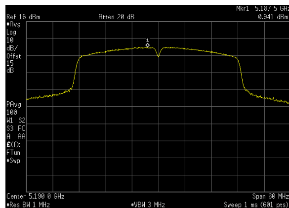
Plot 48 Power Spectral Density, BW 40 M, Ch. 5190 MHz, N mode, ANT 0
