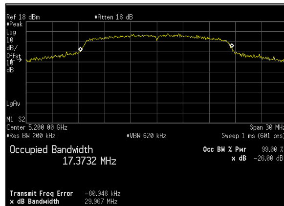
Plot 6. 26 dB Occupied Bandwidth, 26 dB, BW 20 M, Ch. 5200 MHz, A mode, ANT 1
