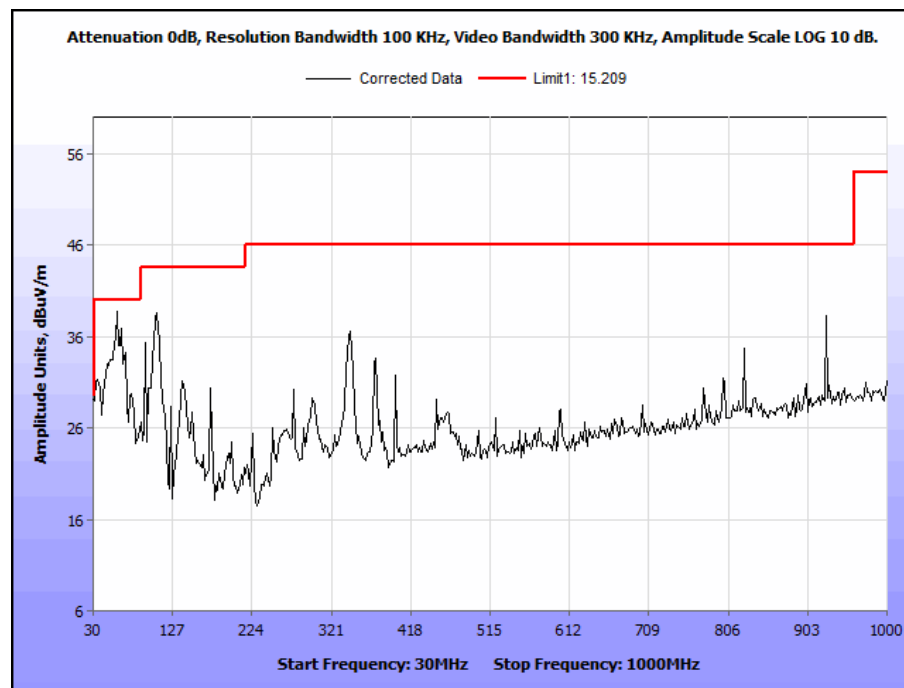
Plot 93. Undesirable Emissions, 30 MHz - 1 GHz (worst-case) V
