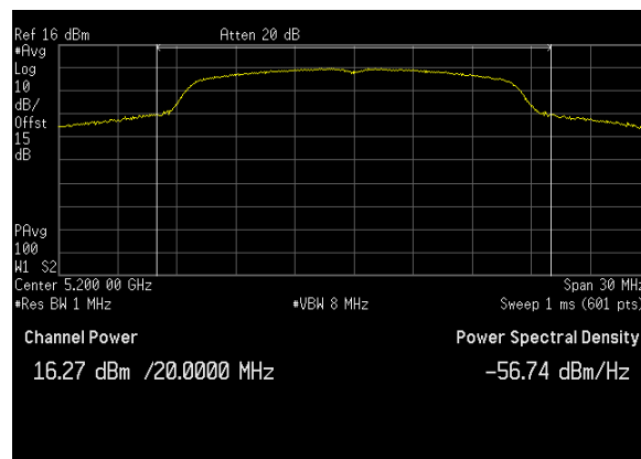
Plot 23. Conducted Output Power, BW 20M, Ch. 5200 MHz, A mode, ANT 1
