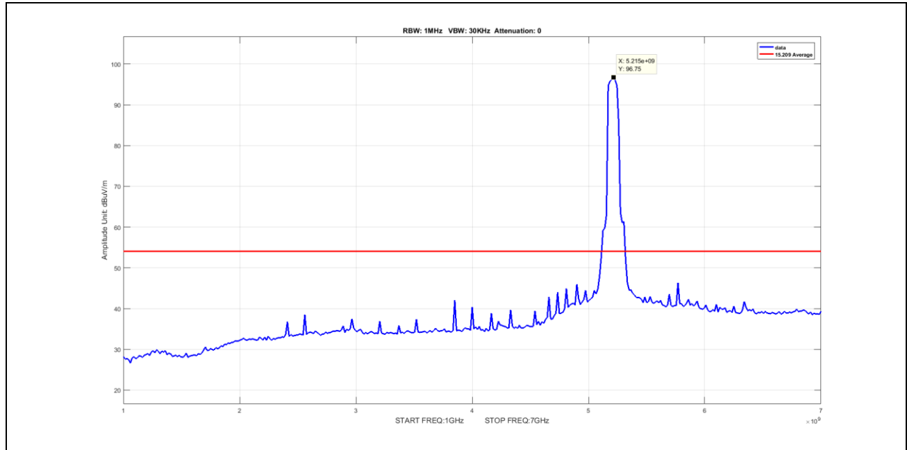
Plot 89. Undesirable Emissions, Average Spurious Emission 1-7GHz, BW 80M, Ch 5210M, AC Mode ANT 0 (worst-case) V
