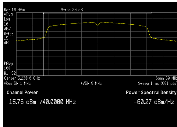
Plot 33. Conducted Output Power, BW 40M, Ch. 5230 MHz, N mode, ANT 1
