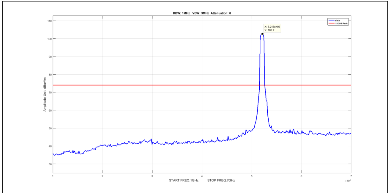
Plot 91. Undesirable Emissions, Average Spurious Emission 1-7GHz, BW 80M, Ch 5210M, AC Mode ANT 1 (worst-case) V
