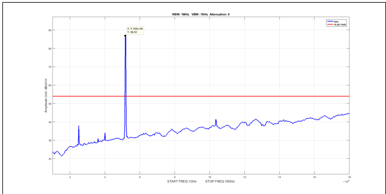
Plot 76. Undesirable Emissions, Average Spurious Emission 1-18GHz, BW 20M, Ch 5180M, N Mode ANT 0 (worst-case) V
