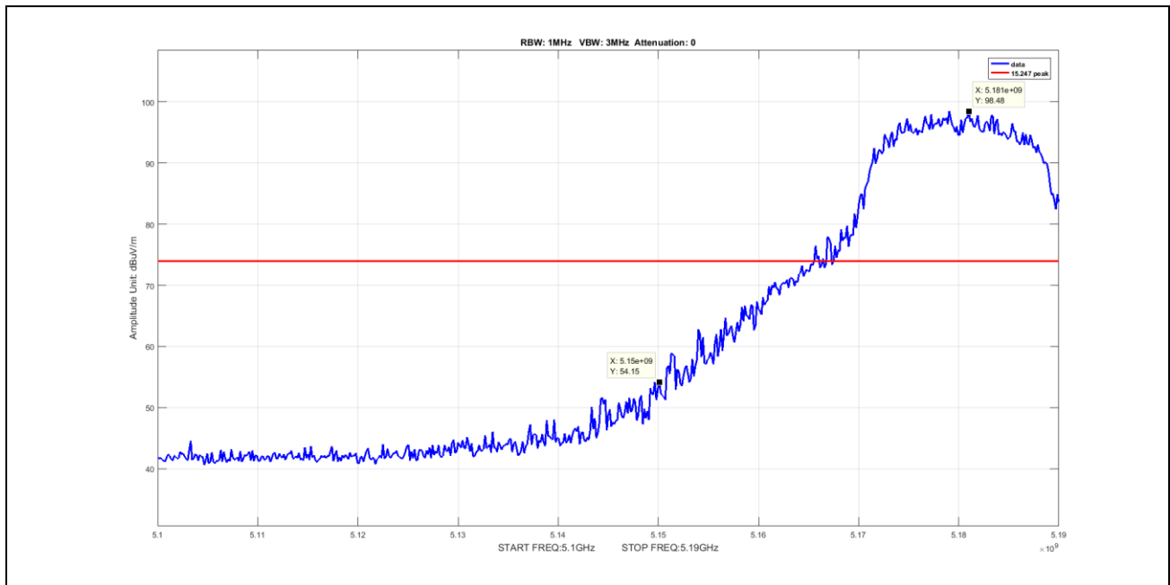
Plot 65. Undesirable Emissions, Peak Band Edge Spurious, BW 20M, Ch 5180M, N Mode ANT 1(worst-case) V
