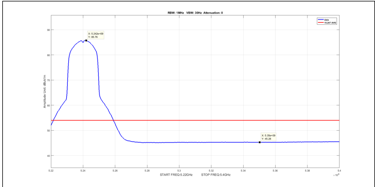
Plot 60. Undesirable Emissions, Average Band Edge Spurious, BW 20M, Ch 5240M, N Mode ANT 0 (worst-case) V
