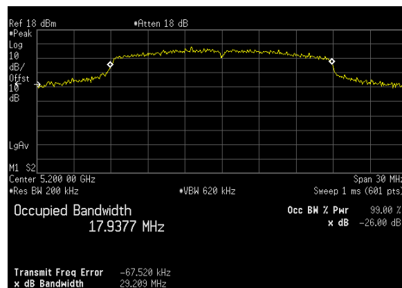
Plot 8. 26 dB Occupied Bandwidth, 26 dB, BW 20 M, Ch. 5200 MHz, N mode, ANT 1
