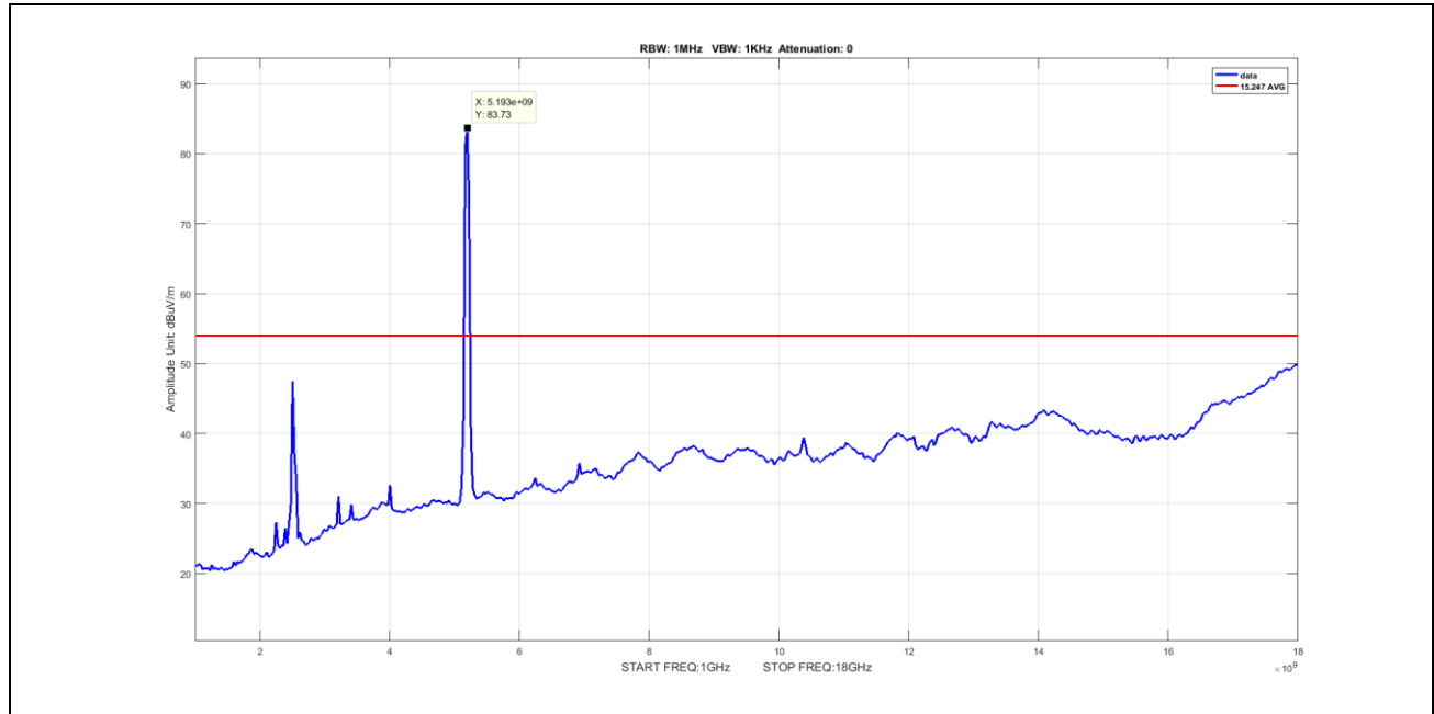
Plot 85. Undesirable Emissions, Average Spurious Emission 1-18GHz, BW 40M, Ch 5190M, N Mode ANT 1 (worst-case) V
