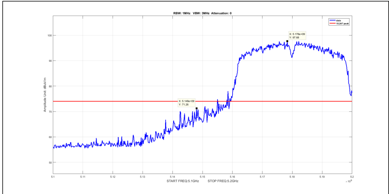
Plot 72. Undesirable Emissions, Peak Band Edge Spurious, BW 40M, Ch 5190M, N Mode ANT 0 (worst-case) V
