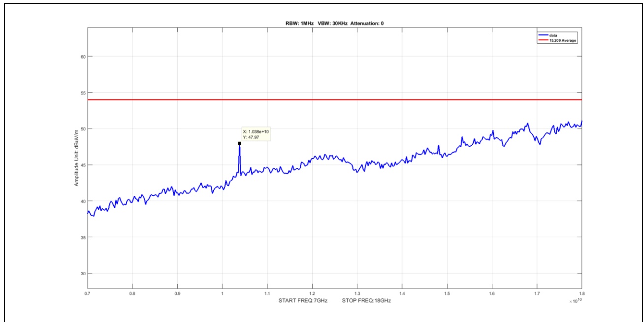
Plot 90. Undesirable Emissions, Average Spurious Emission 7-18GHz, BW 80M, Ch 5210M, AC Mode ANT 0 (worst-case) V
