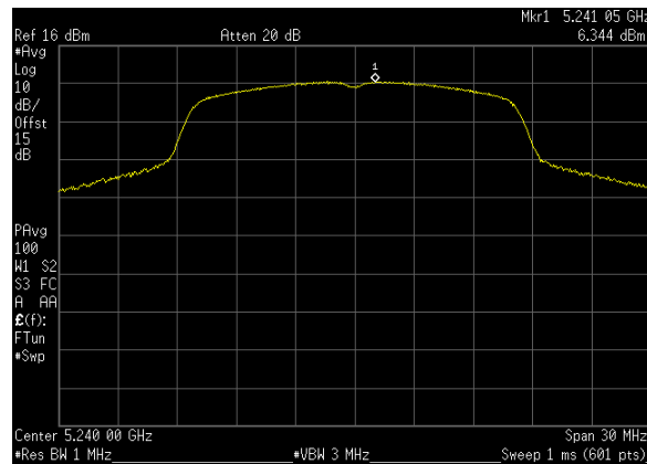
Plot 44. Power Spectral Density, BW 20 M, Ch. 5240 MHz, A mode, ANT 0
