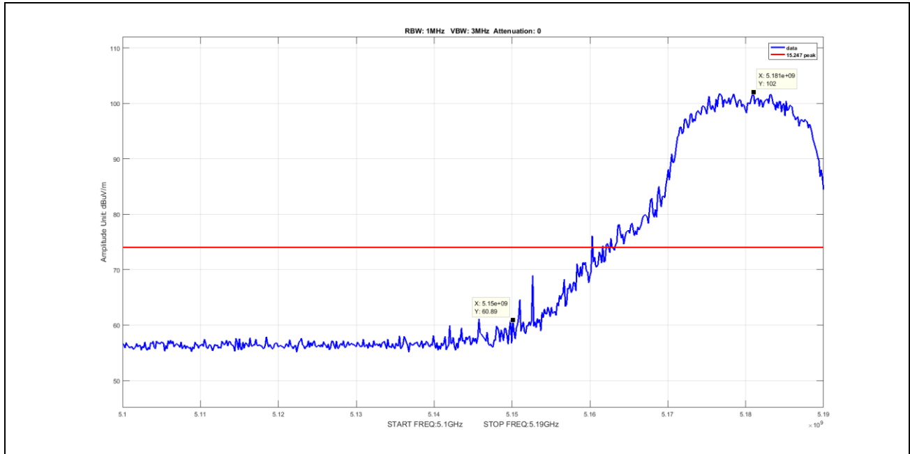
Plot 66. Undesirable Emissions, Peak Band Edge Spurious, BW 20M, Ch 5180M, N Mode ANT 0 (worst-case) V
