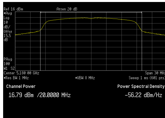
Plot 21. Conducted Output Power, BW 20M, Ch. 5180 MHz, N mode, ANT 1
