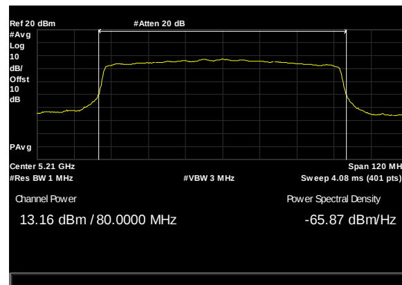
Plot 34. Conducted Output Power, BW 80M, CH. 5210 MHz, AC Mode, ANT 0
