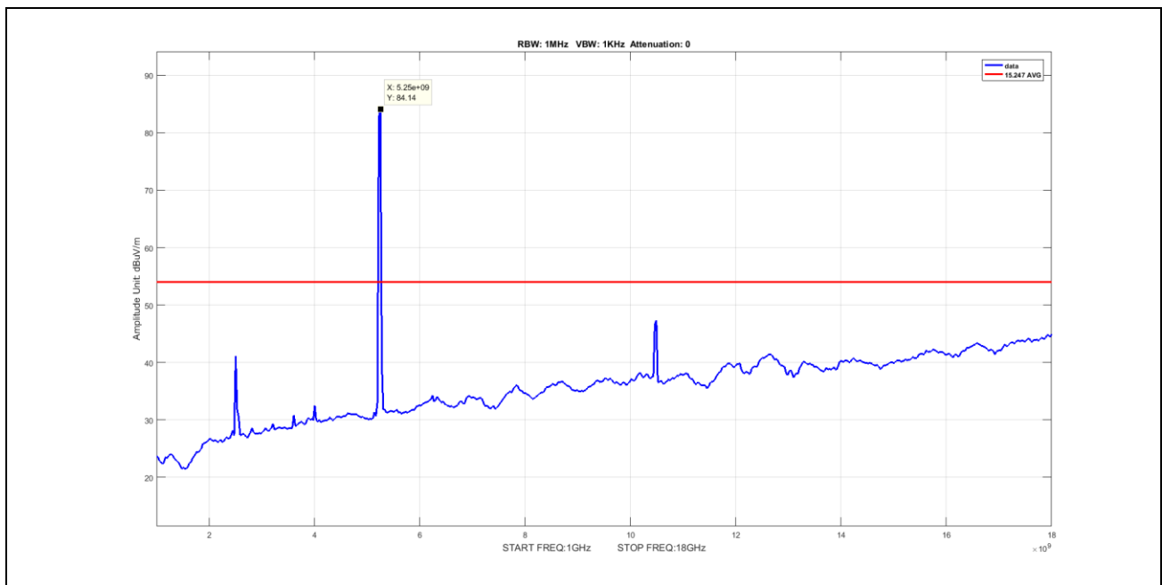
Plot 84. Undesirable Emissions, Average Spurious Emission 1-18GHz, BW 20M, Ch 5240M, N Mode ANT 0 (worst-case) V
