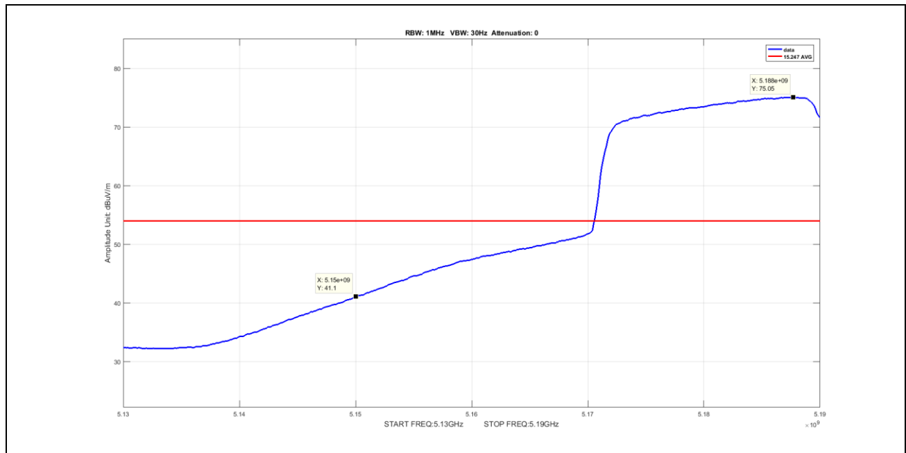
Plot 61. Undesirable Emissions, Average Band Edge Spurious, BW 40M, Ch 5190M, N Mode ANT 1 (worst-case) V
