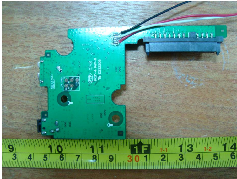
EUT –Indicate Light Board Top View
