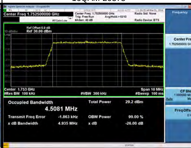
16QAM-20375
