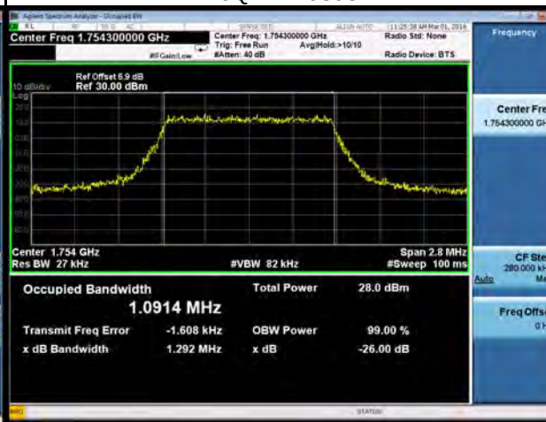
16QAM-20393
