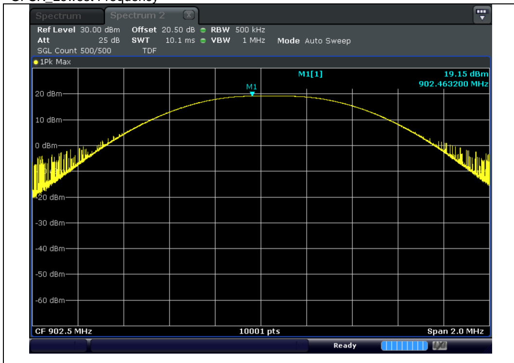
GFSK_Lowest Frequency
