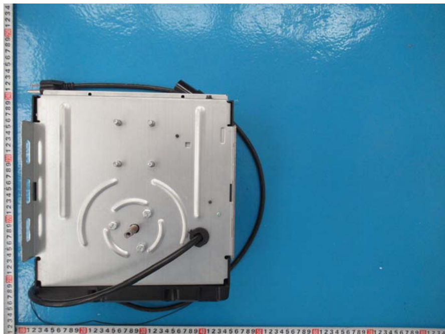
EUT (2211-D/615CC) – Bottom View
