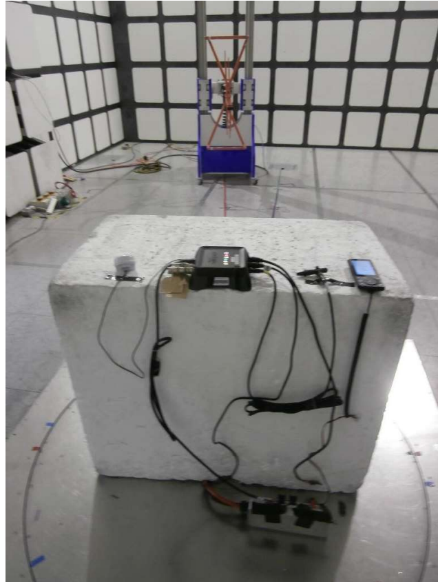
Figure 35 – Radiated Emissions, 30 MHz to 1 GHz, Orientation X
