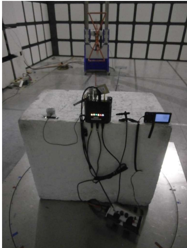
Figure 37 – Radiated Emissions, 30 MHz to 1 GHz, Orientation Z
