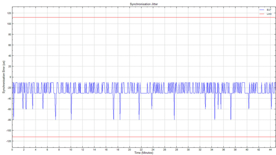
Synchronisation Jitter – UTC Direct
