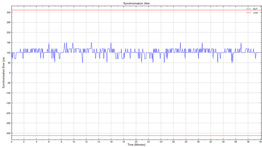
Synchronisation Jitter – UTC Indirect
