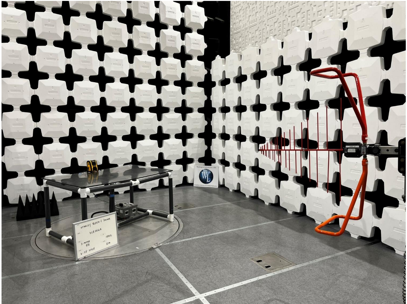
Radiated Testing, 30MHz to 1GHz
