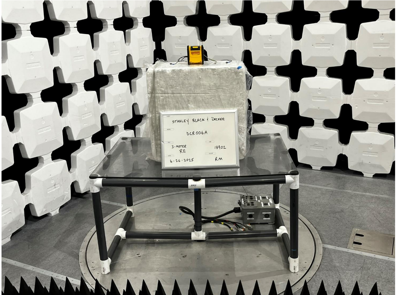
Radiated Testing, > 1GHz
