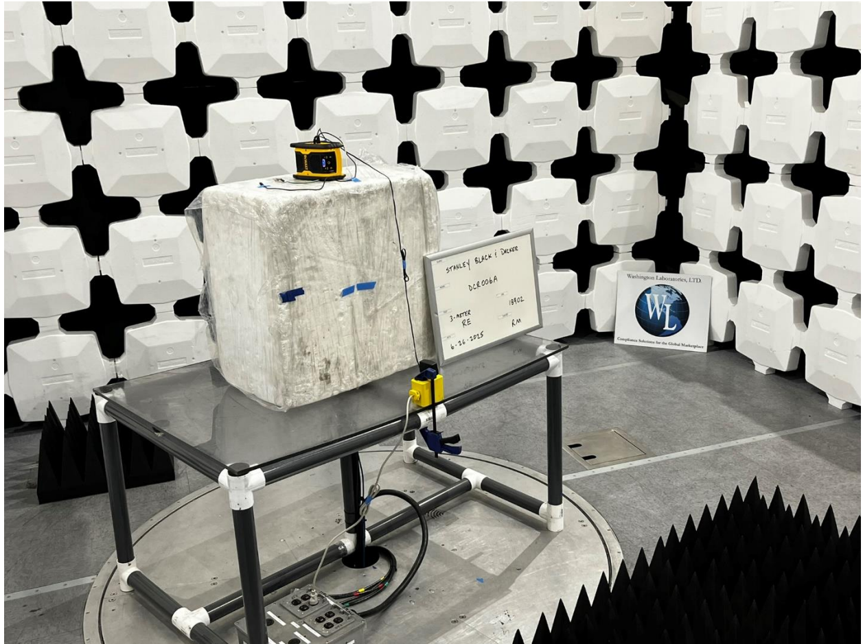
Radiated Testing, > 1GHz
