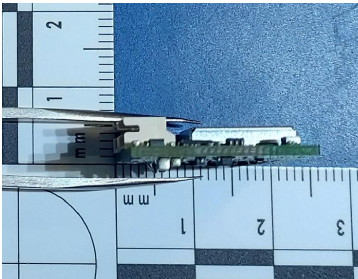
NA557427_edge2_No_Overmold
