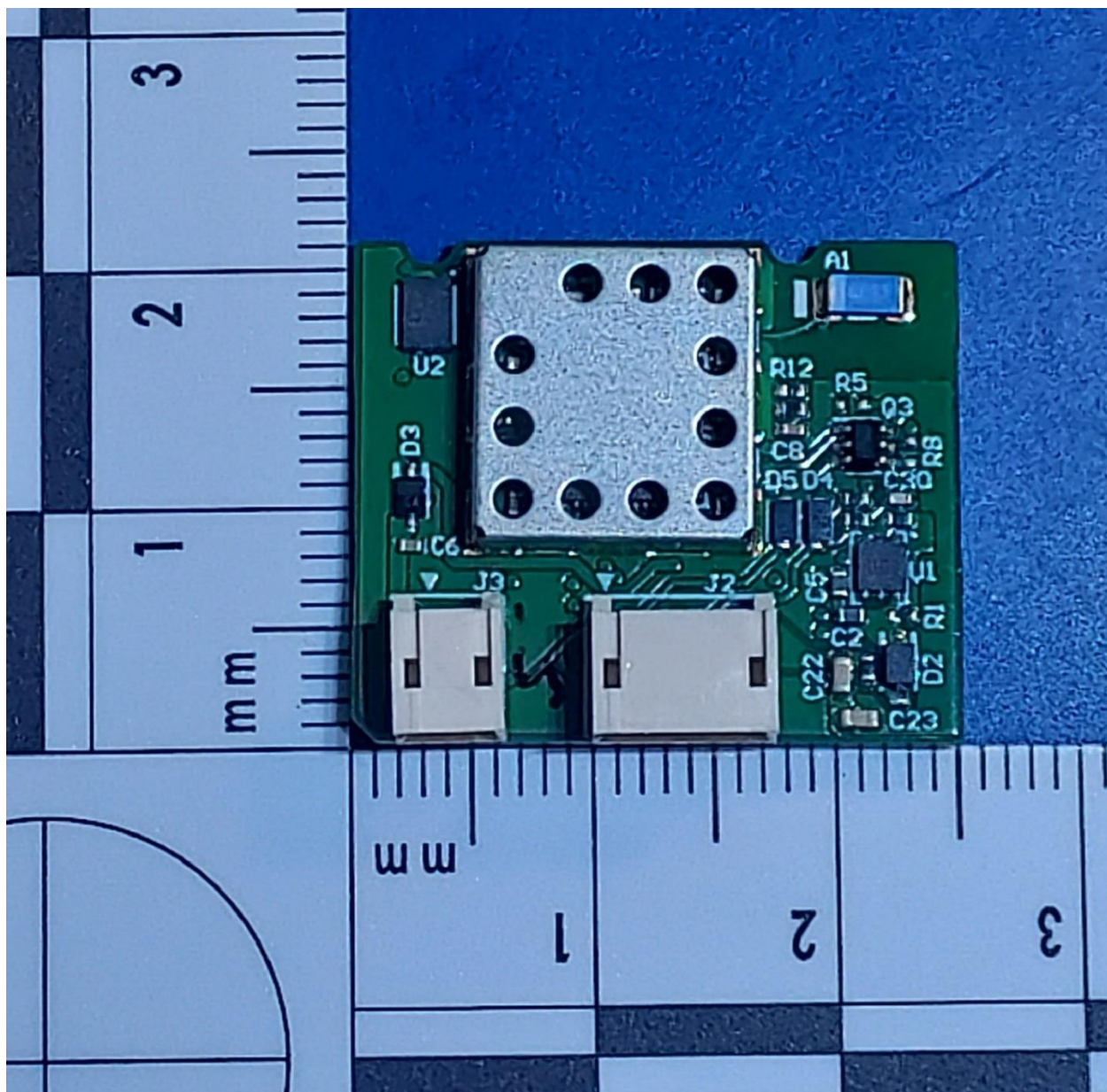
NA557427_top_No_Overmold
