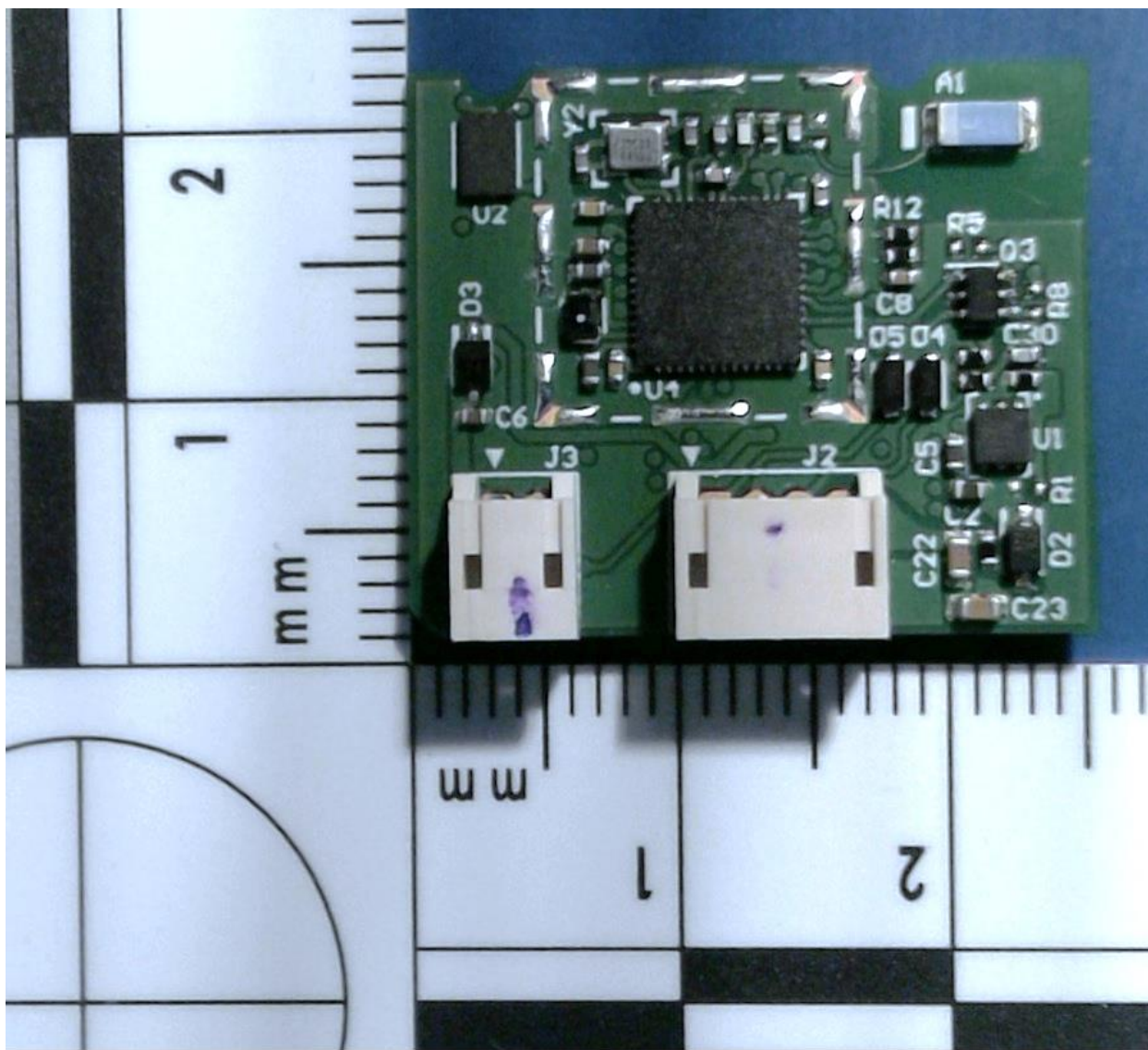
NA557427_top_No_Overmold_No_Shield
