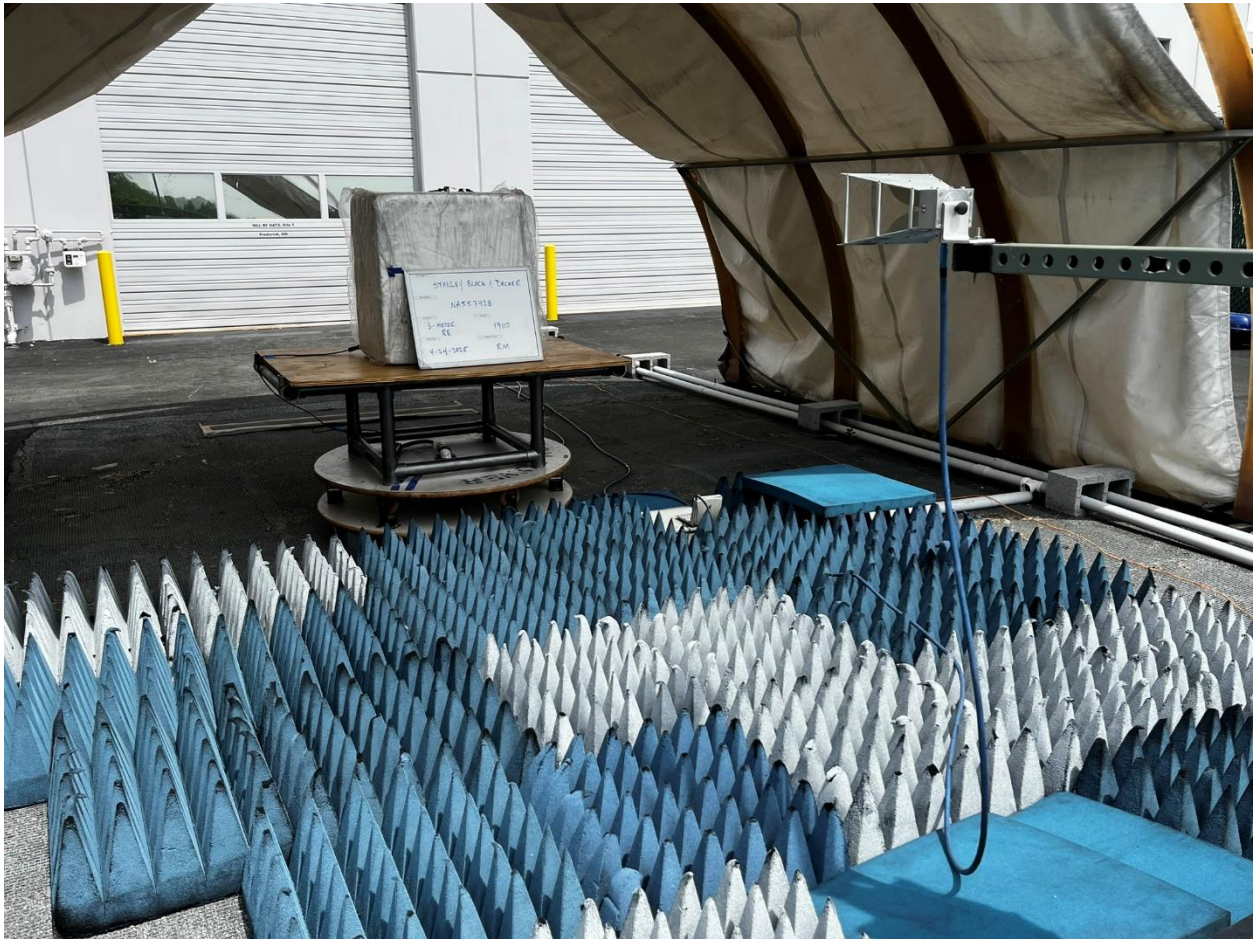
RE, > 1GHz View 4
