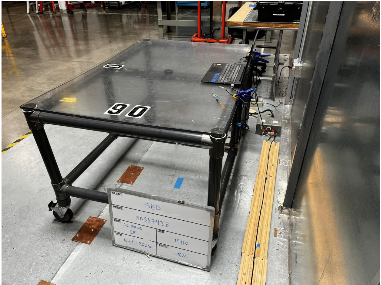
AC Powerline CE, Side View
