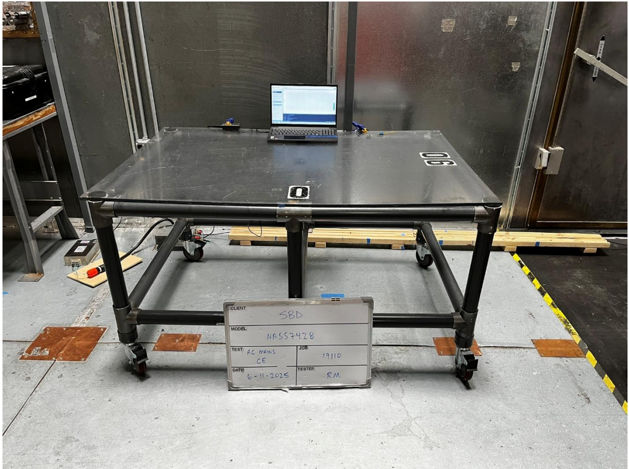
AC Powerline CE, Front View
