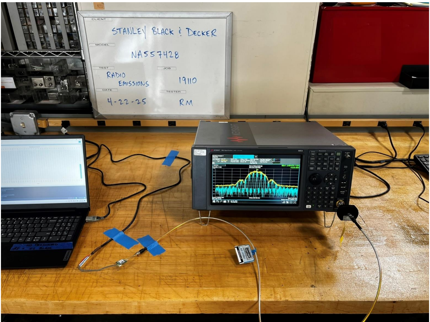
Radio Antenna Port Testing
