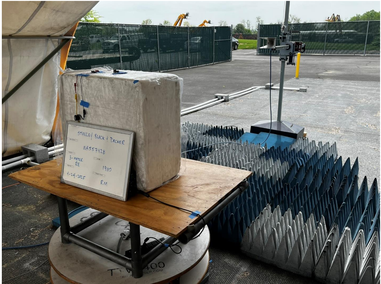
RE, > 1GHz View 3
