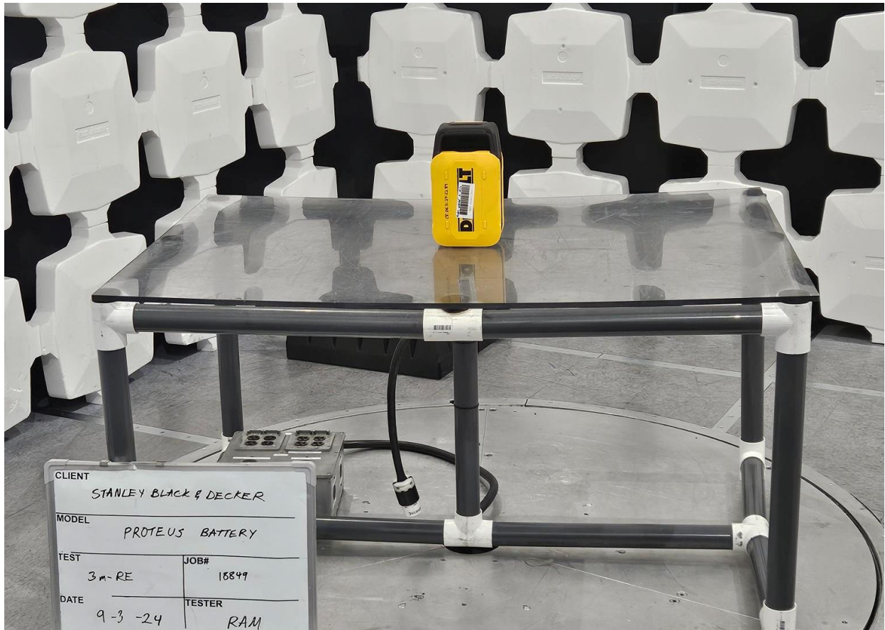
Radiated Emissions View 2, <1GHz
