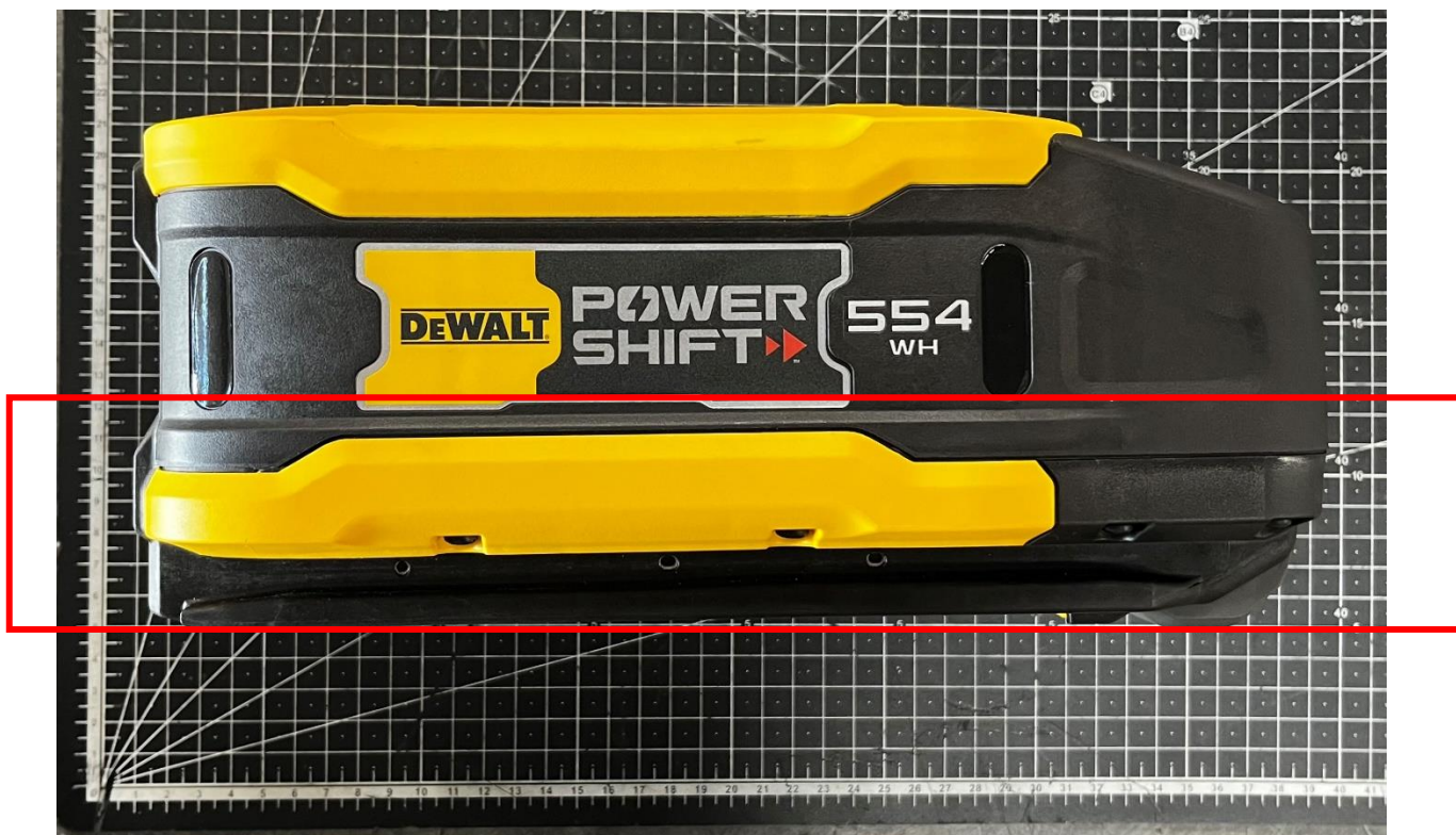
Host Battery Pack, Side View with Module Location
