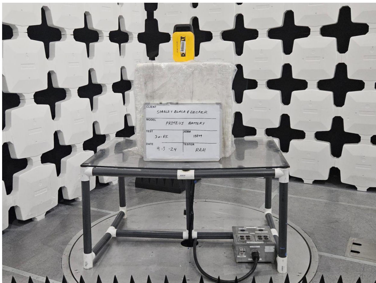
Radiated Emissions View 4, >1GHz
