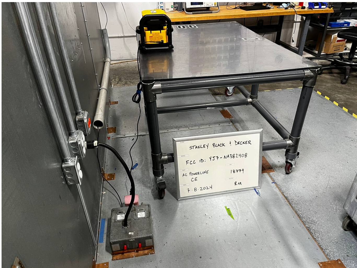
AC POWERLINE EMISSIONS
