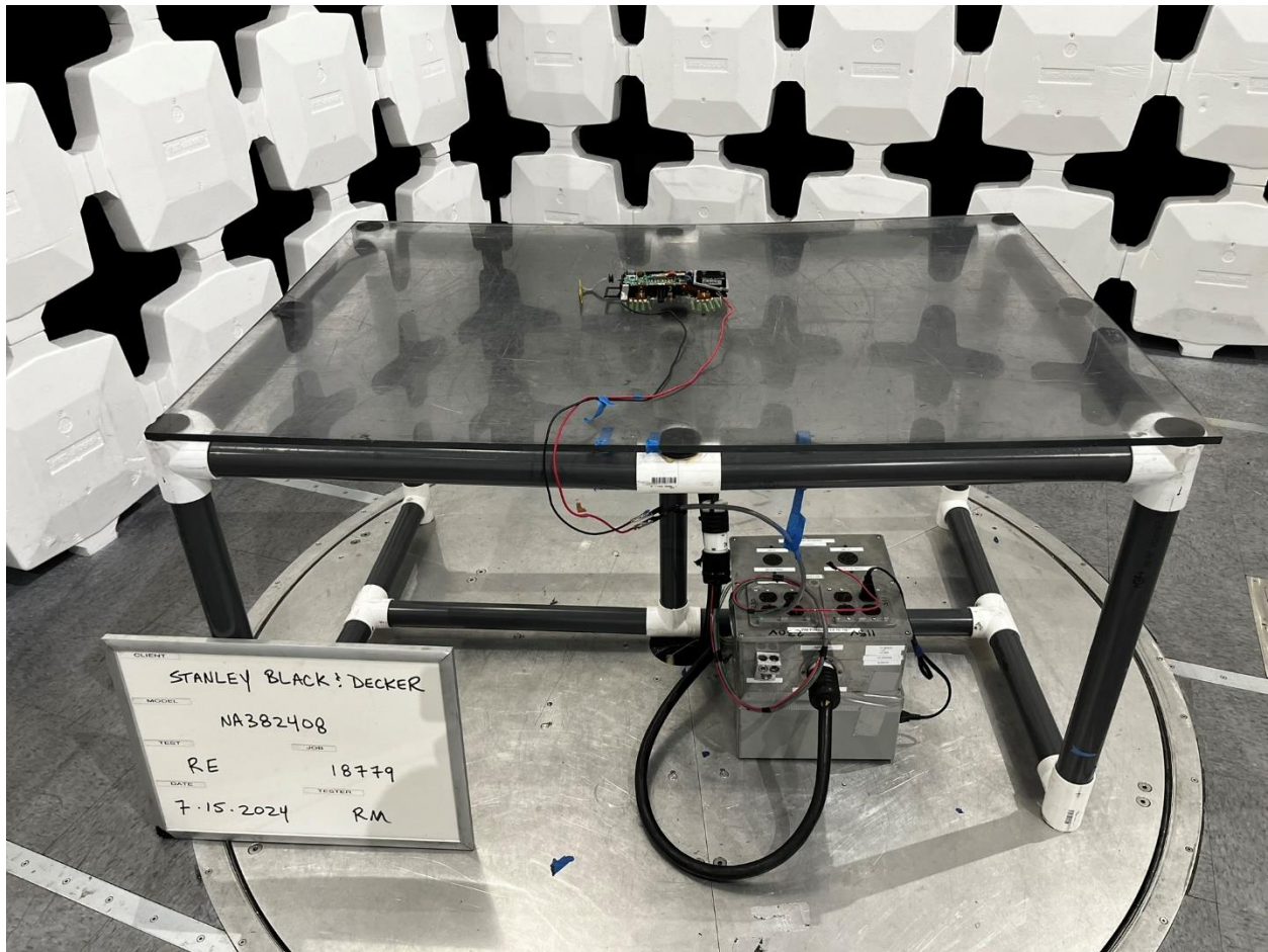
3-meter Radiated Emission, Rear View #2 (30M-1GHz)
