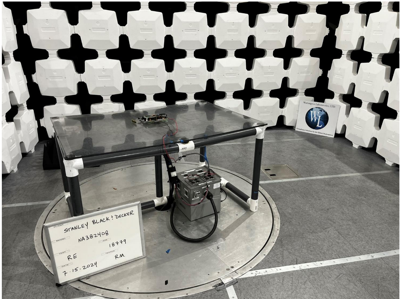
3-meter Radiated Emission, Rear View #1 (30M-1GHz)
