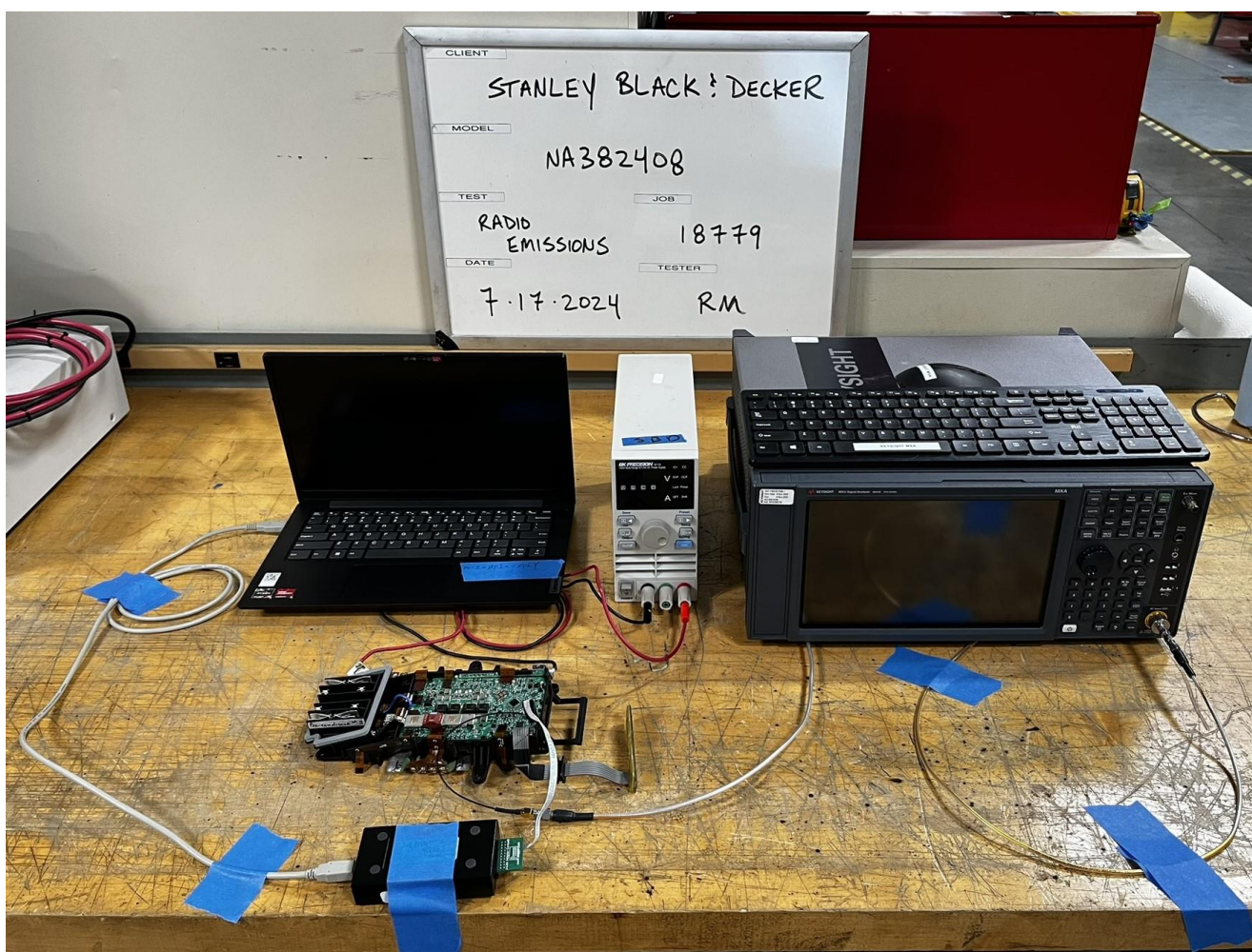
Benchtop Conducted, Radio Emissions
