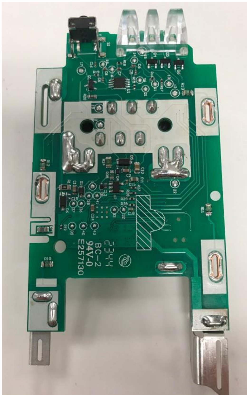
PCBA Bottom View
