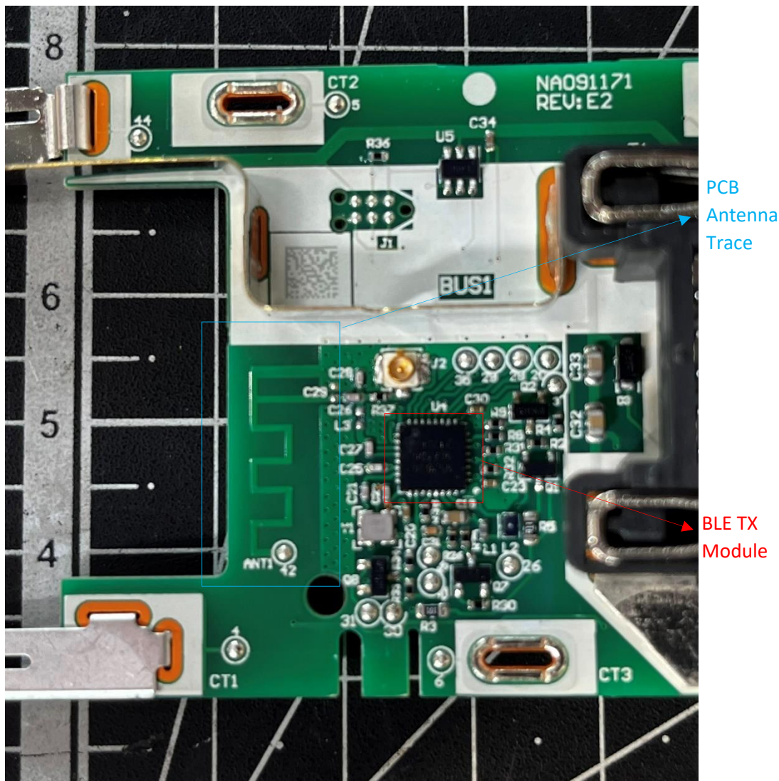
Antenna and PCB Identification Photograph
