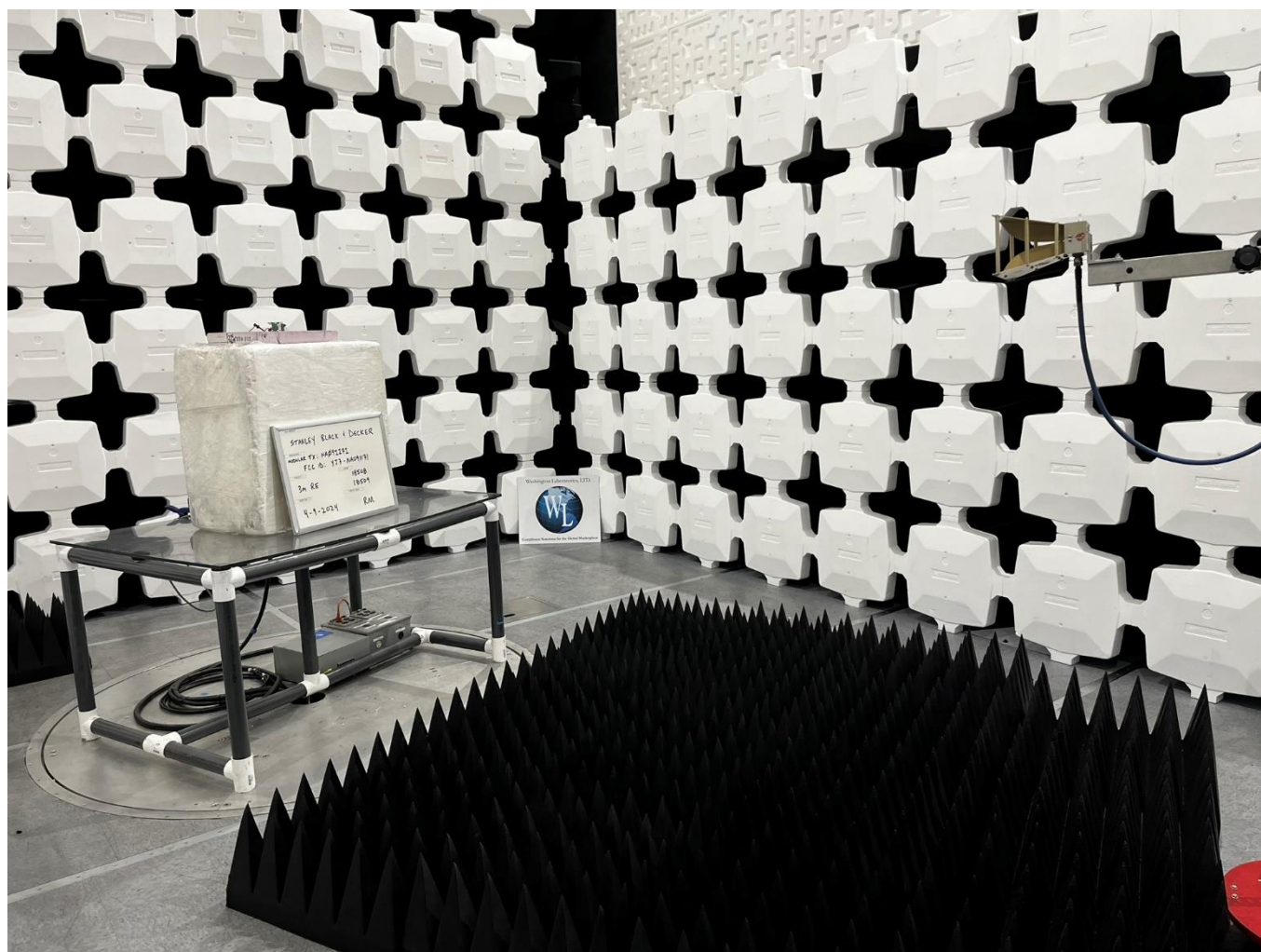
3-meter Radiated Emissions, View #4
