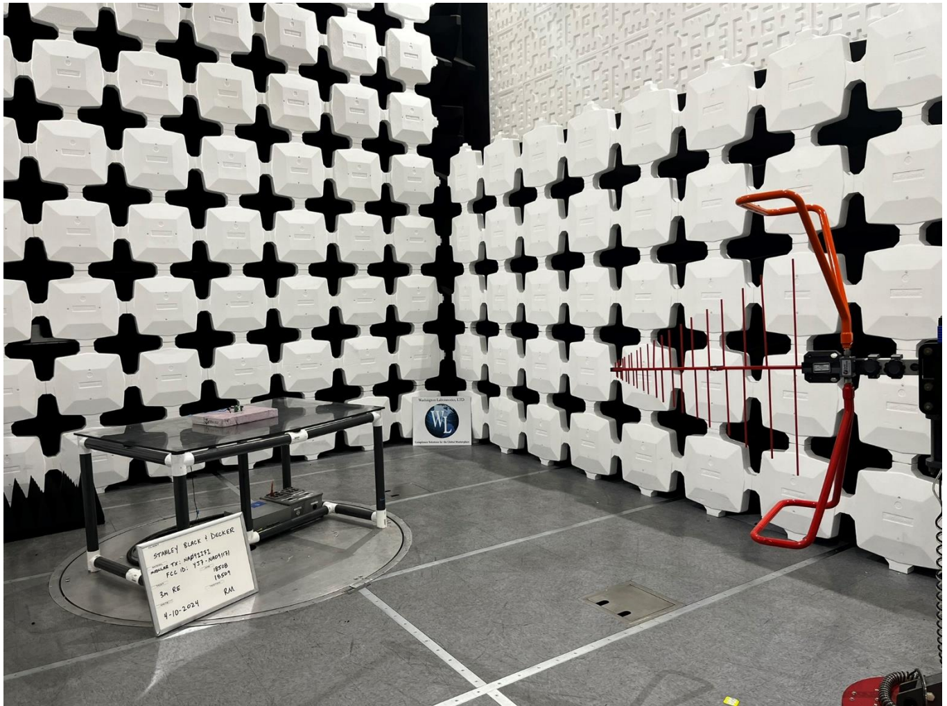
3-meter Radiated Emissions, View #1
