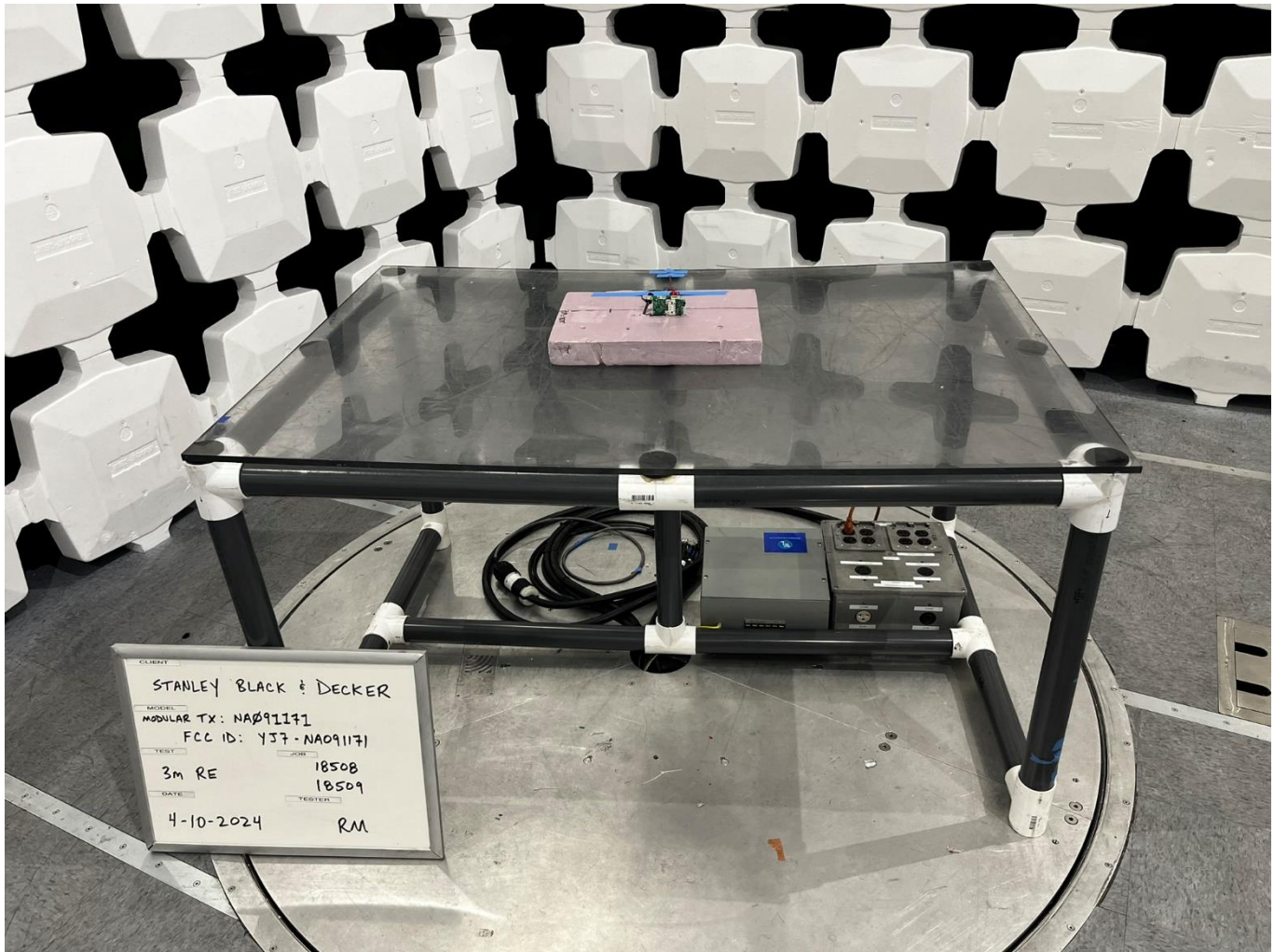
3-meter Radiated Emissions, View #2
