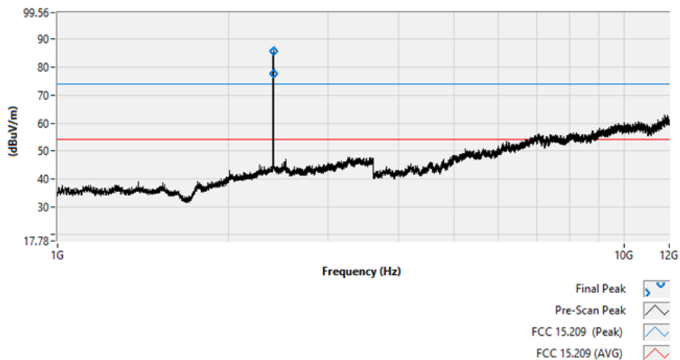
Pre-scan and Final Data (Horizontal)
