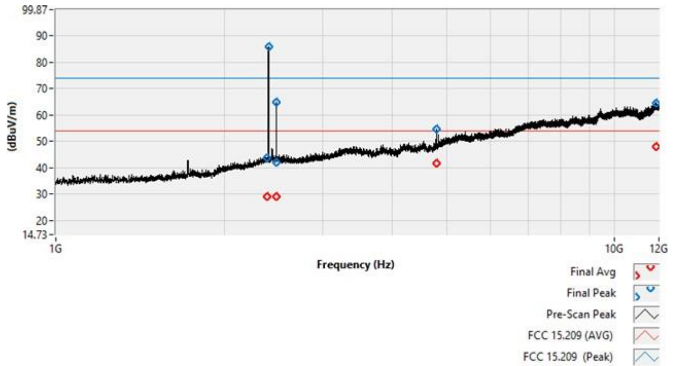
Worst-Case Pre-scan and Final Data (Vertical)
