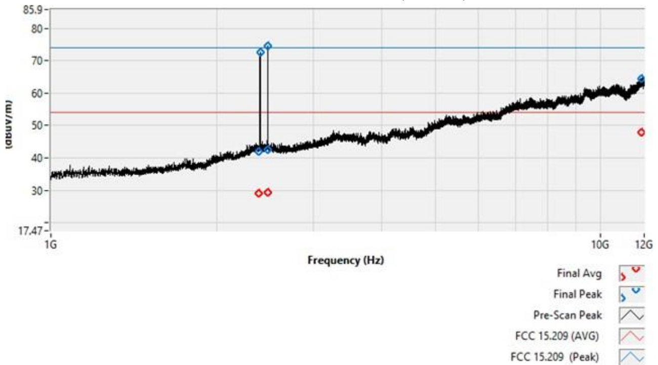
Worst-Case Pre-scan and Final Data (Horizontal)
