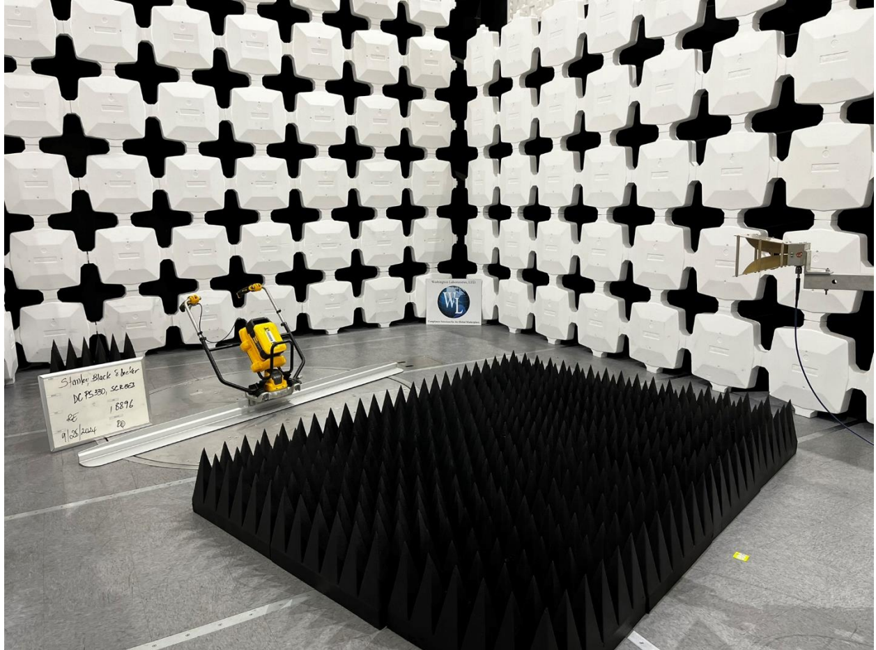
Radiated Emissions, handheld portion Evaluation, > 1GHz View 2
