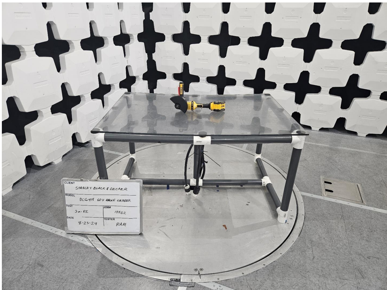
3-meter Radiated Emissions Test Configuration, Front View (30MHz-1GHz)
