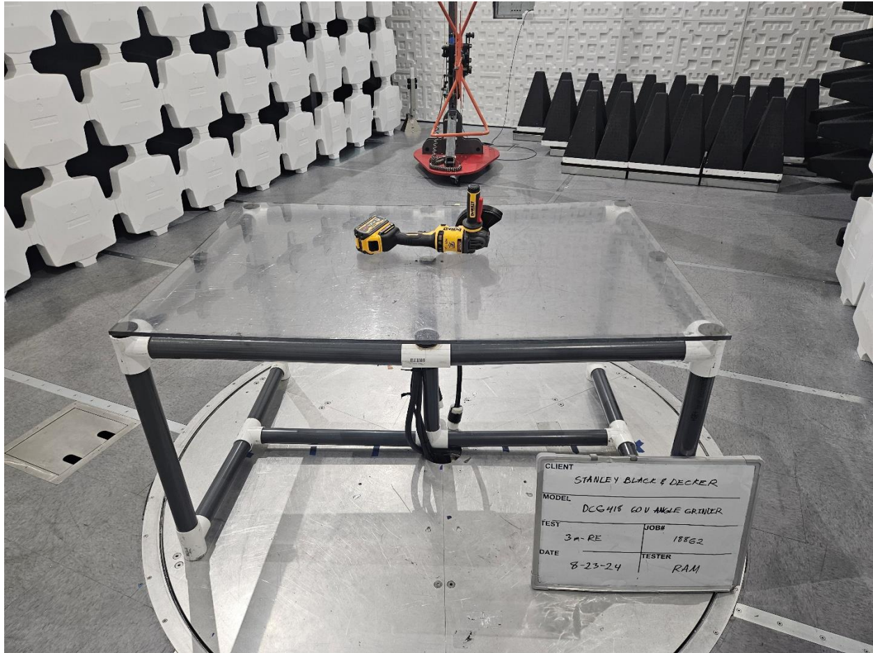
3-meter Radiated Emissions, Configuration Rear View (30MHz-1GHz)
