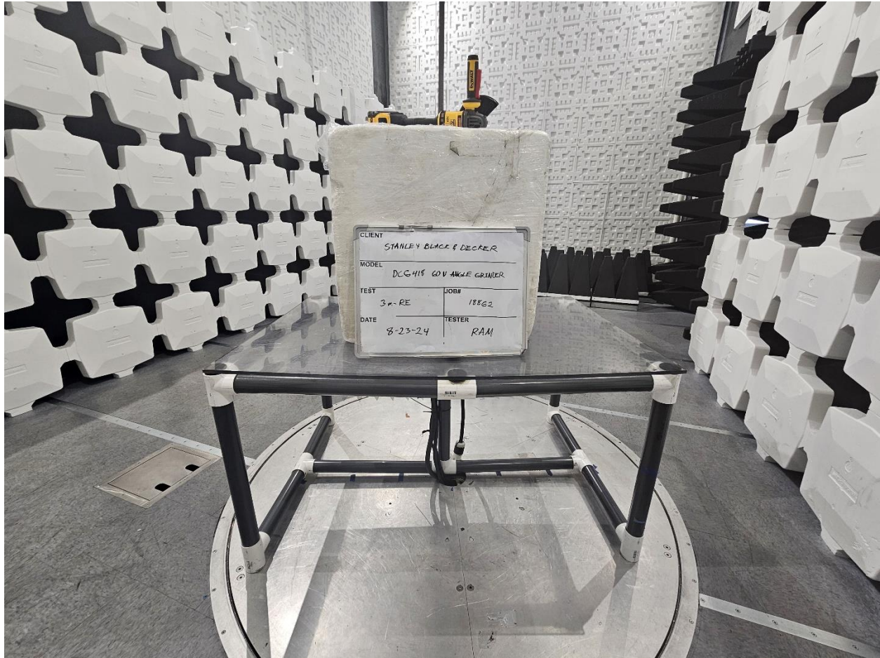
3-meter Radiated Emissions, Configuration Rear View (Above 1GHz)
