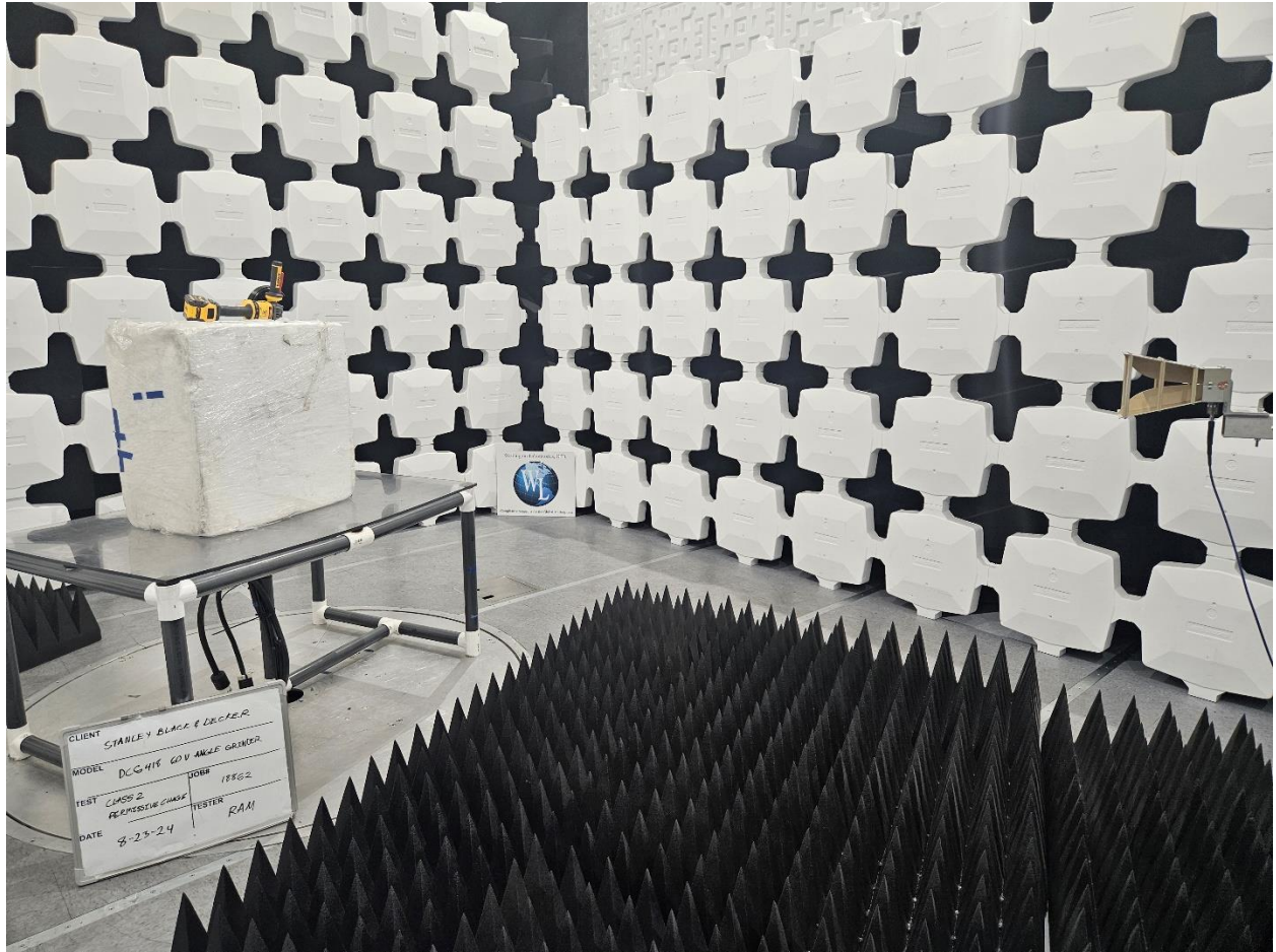
3-meter Radiated Emissions, Configuration Front View (Above 1GHz)
