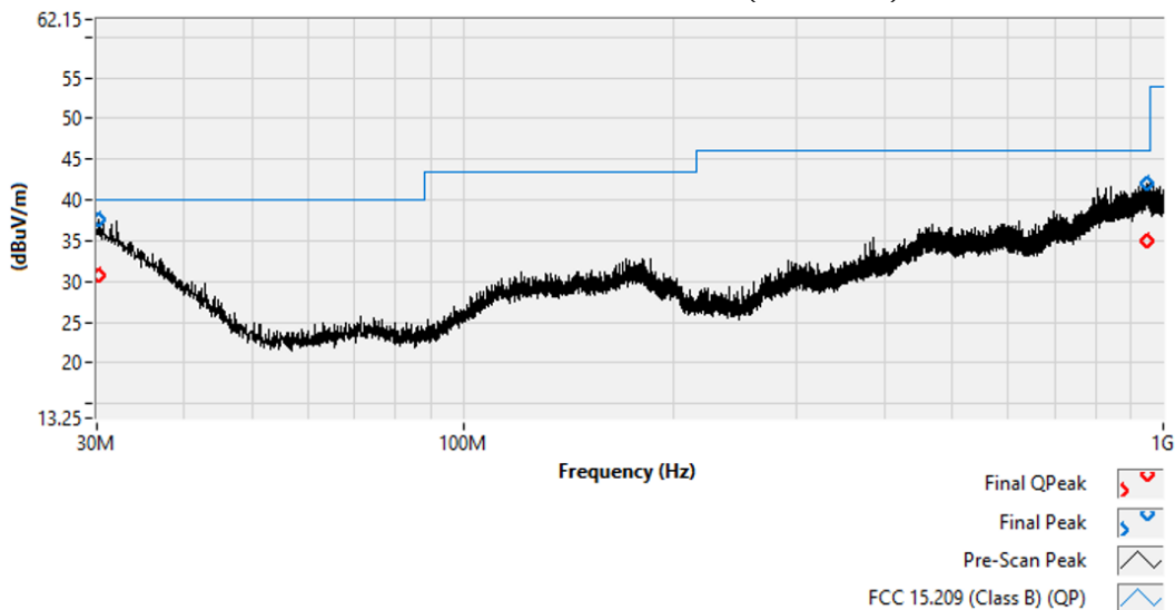
Worst-Case Pre-scan and Final Data (Horizontal)
