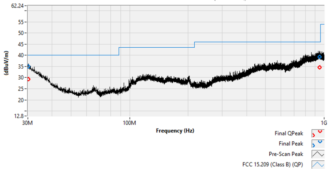
Worst-Case Pre-scan and Final Data (Vertical)
