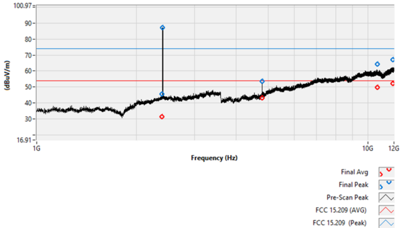
Worst-Case Pre-scan and Final Data (Vertical)
