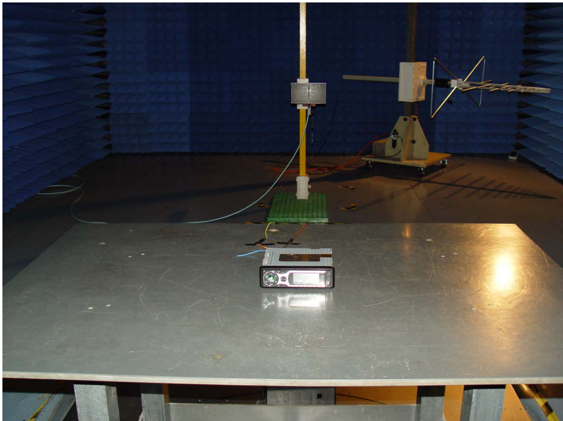
Radiated emissions test >1G
